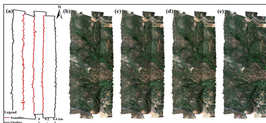
Figure 6. True color composite images before and after correction. (a) Outline and seamline of the hyperspectral mosaic image, (b) Uncorrected mosaic, (c) SCS+C corrected mosaic, (d) Minnaert+SCS corrected mosaic, (e) RA-TOC-CA corrected mosaic.
