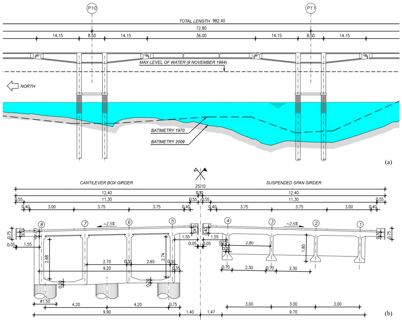
Figure 3. (a) Longitudinal section of Piers 10 and 11 and (b) cross sections of the A22 Po River Bridge. Dimensions in meters.
