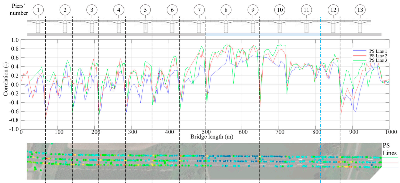
Figure 16. Linear correlation between PS displacement time series and temperature variation plotted against the length of the bridge. PSs are divided into three lines.
