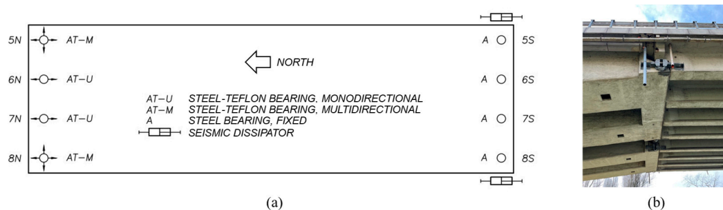
Figure 4. (a) Scheme of the suspended span bearings; (b) picture of the seismic dissipators.
