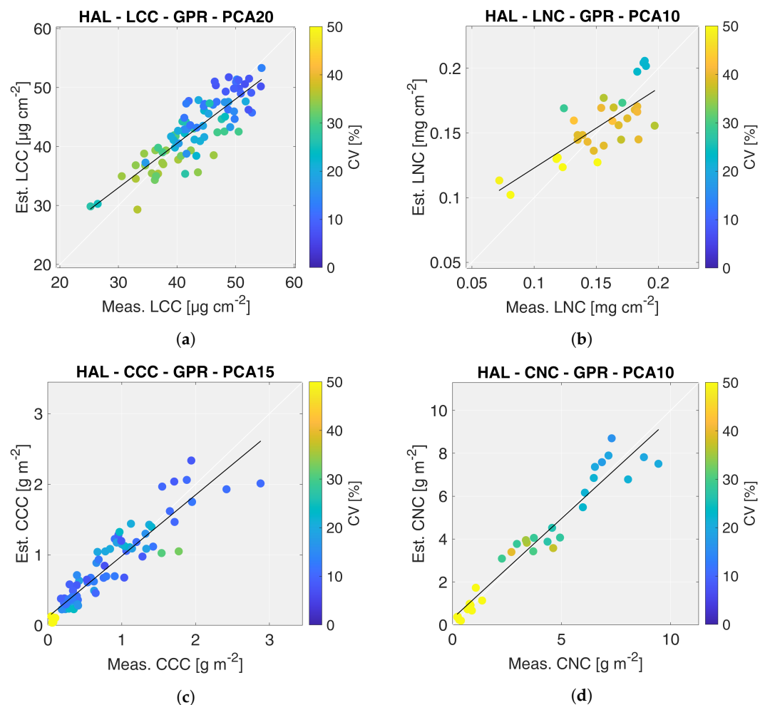
Figure 4. Scatter plots of the best HAL models: leaf chlorophyll content (a), leaf nitrogen content (b), canopy chlorophyll content (c), canopy nitrogen content (d). The colors of points represent the coefficient of variation (CV) estimated by the GPR algorithm.
