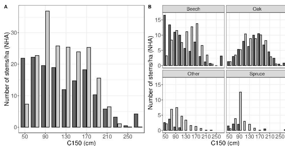
Figure 10. SSDs for the independent dataset: (A) total SSDs per hectare (all species) and (B) species-specific SSDs per hectare. Dark bars correspond to field measurements and light bars to predictions.
