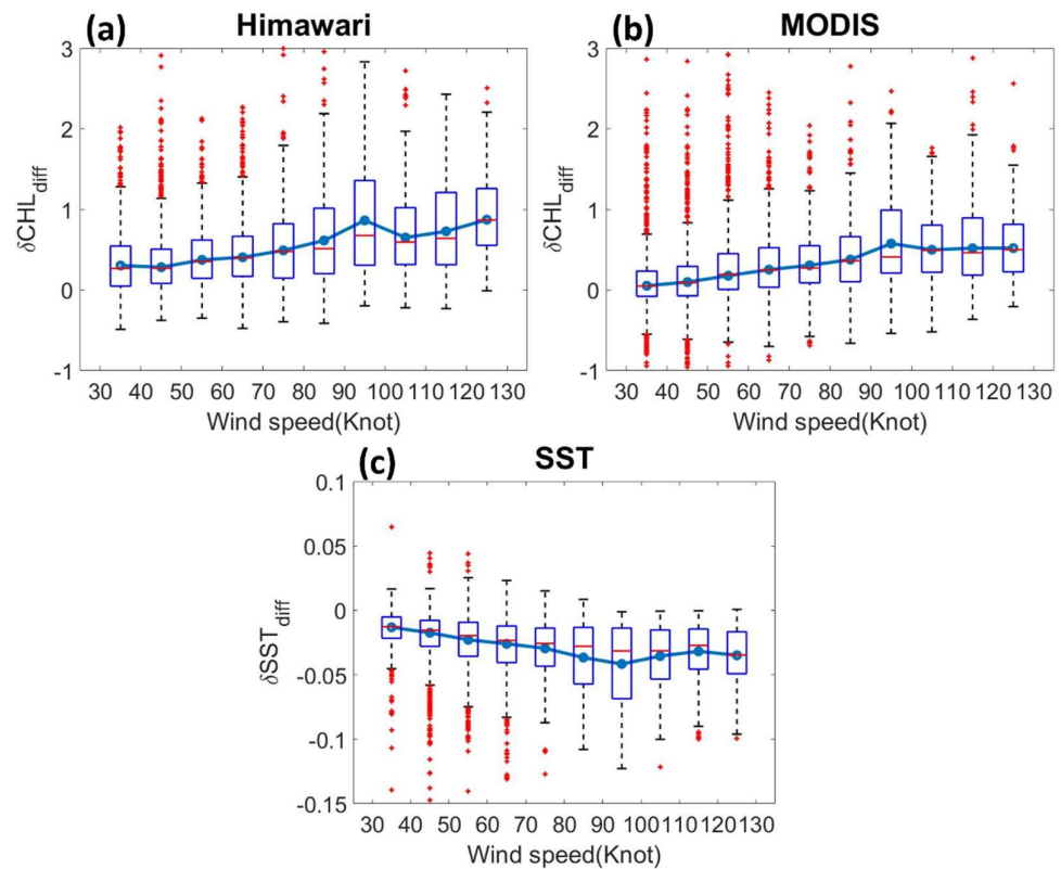
Figure 7. Typhoon-induced Chl-a changes ( \delta CHL_{diff} ) corresponding to different wind forcing strengths calculated on the basis of Equation 3 for (a) AHI and (b) MODIS composites. The change rate of SST ( \delta SST_{diff} ) corresponding to different wind forcing is shown in (c). The lowest and highest sides of the blue rectangles denote the lower quartile (25th percentile) and upper quartile (75th percentile), respectively. The red line in the rectangles denotes the median. The minimum and maximum bars denote the lower quartile -1.5 \times IQR and upper quartile +1.5 \times IQR , respectively, where IQR denotes the upper quartile–lower quartile. The red plus signs denote the outliers. Light blue lines connect the means of each interval removing outliers.
