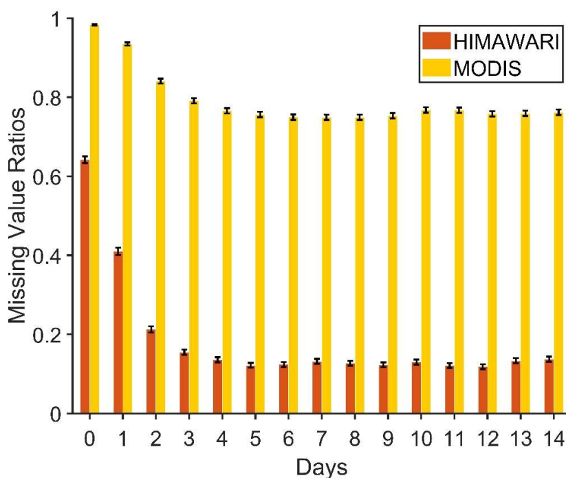
Figure 3. Characteristics of the ratios of missing values of Himawari-8 AHI images (bars in orange) and MODIS images (bars in yellow). The error bars represent the 95% confidence intervals from the mean values on different days for the two datasets.
