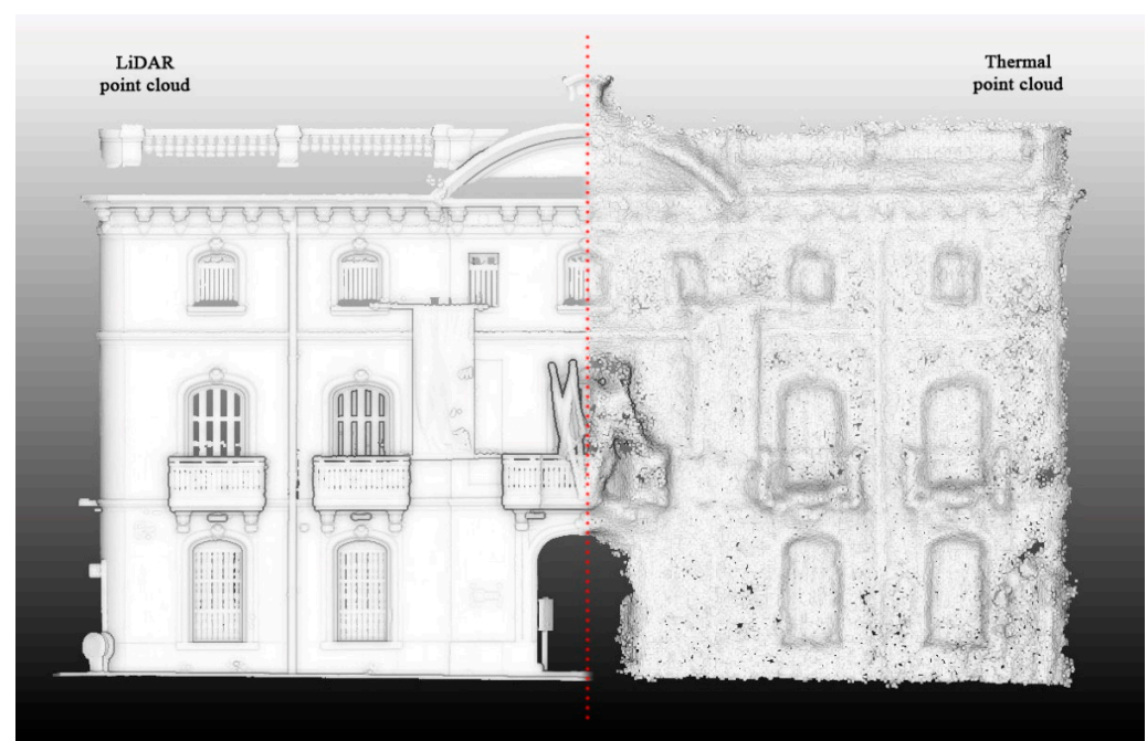
Figure 12. On the left, LiDAR point cloud of the southern façade. On the right, photogrammetric dense point cloud derived from TIR images.
