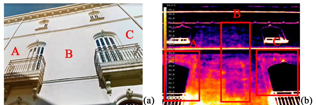
Figure 14. (a) Colour image of a section of the eastern façade of the Palacio; (b) thermal image of the same area. It is possible to observe some anomalies not visible in the colour image but clearly detectable in the thermal image (highlighted in red as A, B and C).
