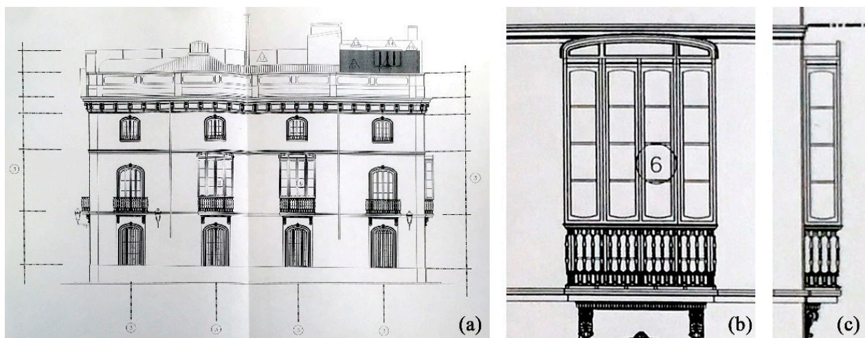
Figure 16. (a) CAD drawing of the eastern façade in 1995 before renovation. The two central windows of the second floor are shown with a glass housing, which was later removed; (b) front view of the housing; (c) side view. Architect Francisco Esquembre Casañ. Intermediate Municipal Archive of the Valencia City Council. Urban Police, file number 608, year 1995.
