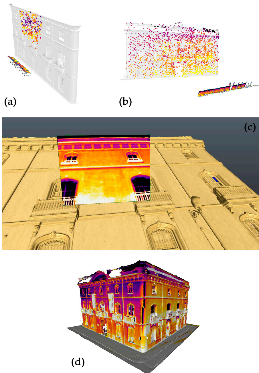
Figure 7. (a) Oriented block of thermal images following an SfM-based pipeline (upper area of the central modules of the northern façade); (b) oriented block of thermal images following an SfM-based pipeline (southern façade); (c) example of oriented TIR image projected of the three-dimensional surface; (d) 3D mesh after the first phase of the texturisation.
