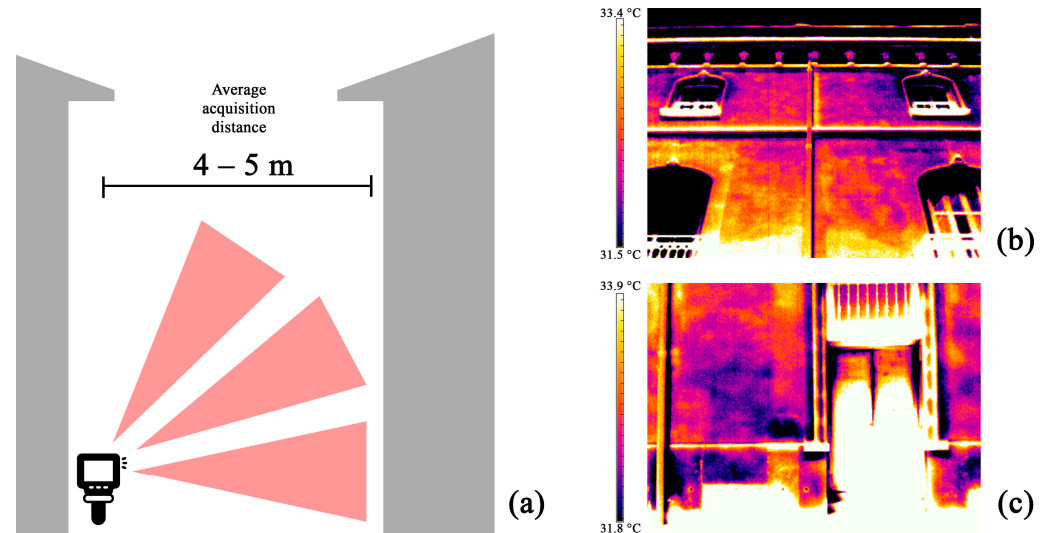
Figure 5. (a) TIR image acquisition scheme; (b) example of a thermal image acquired, of the upper area of the façade, and, therefore, characterised by a high perspective distortion; (c) example of a thermal image acquired, corresponding to the first floor of the building, covering only a limited portion of the façade.
