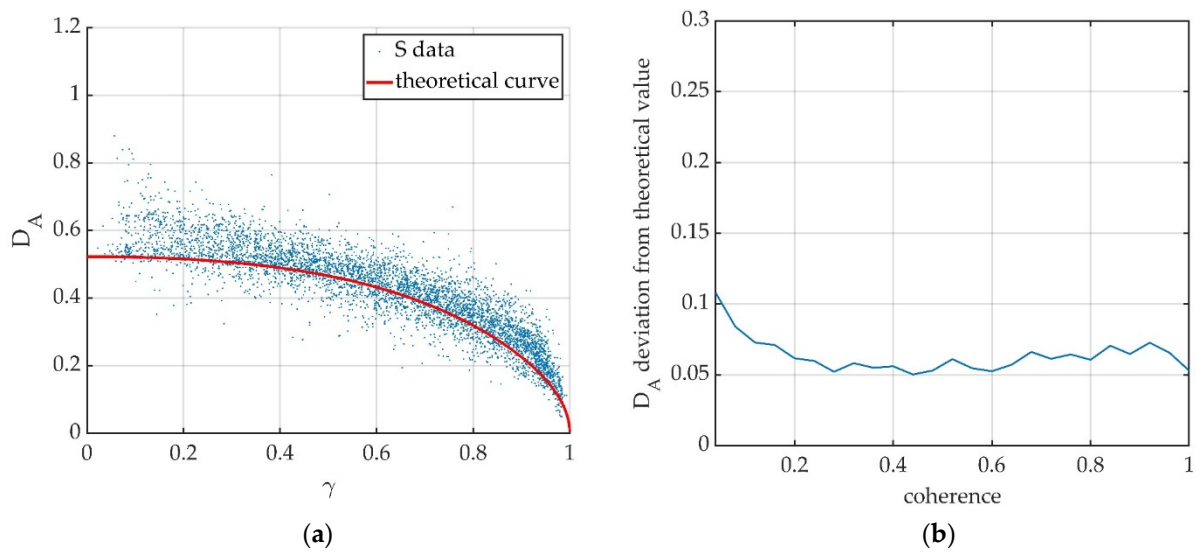
Figure 7. Results obtained for S-band data. (a) Relation between amplitude dispersion index D_A and coherence \gamma of experimental data compared to the theoretical red curve, Equation (14). Each dot represents a resolution cell in the analyzed area. (b) Deviation of experimental D_A values from theoretical ones.
