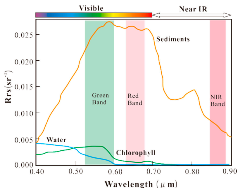
Figure 5. Remote sensing reflectance (Rrs) of clear water (blue), water with chlorophyll content (green), and water with sediments (orange). The green, red, and NIR bands of Landsat 8 images are drawn in the above figure. Note that the figure is modified from Sherry's research [44].
