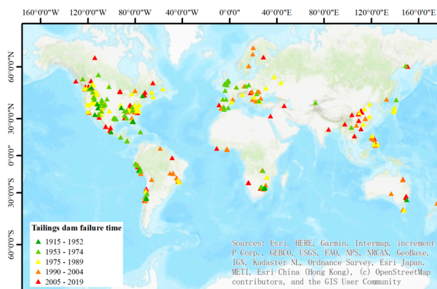
Figure 4. Tailings dam failures (1915–2019) with their occurrence times.
