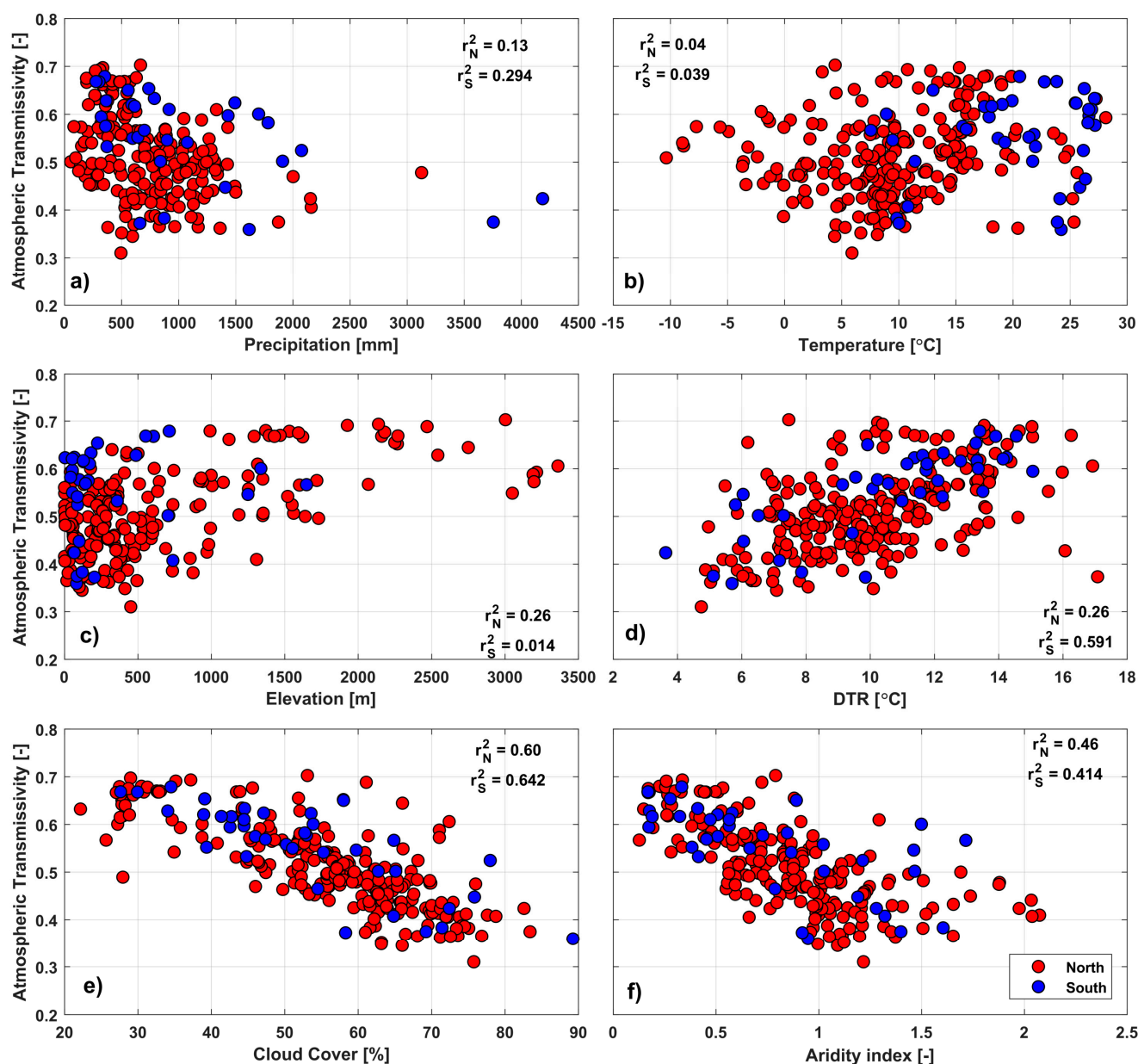
Figure 4. Atmospheric transmissivity ( \tau ) plotted as a function of six different variables for the NH and the SH. Locations lying in the NH across the globe are denoted by red, and the locations lying in the SH across the globe are denoted with blue. Six different \tau affecting factors selected in this study are (a) precipitation; (b) temperature; (c) elevation; (d) diurnal temperature range (DTR); (e) cloud cover; and (f) aridity index. All these variables are separated based on their geographical information obtained from the Ameriflux, Fluxnet, and Ozflux stations.
