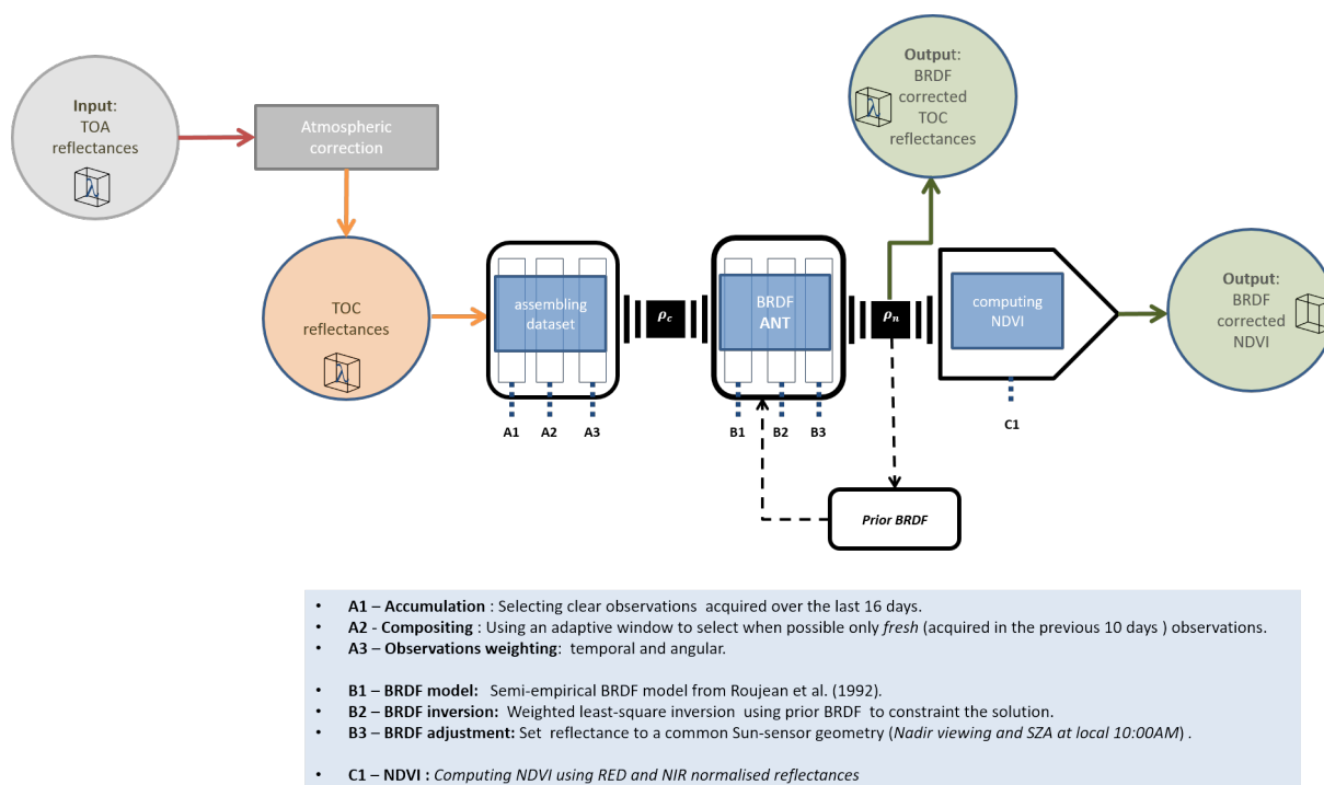
Figure 2. Diagram flow of the BRDF processor. Inputs and outputs are TOC reflectances and NDVI, respectively. The BRDF correction is applied independently to each spectral band and is pixel-based.
