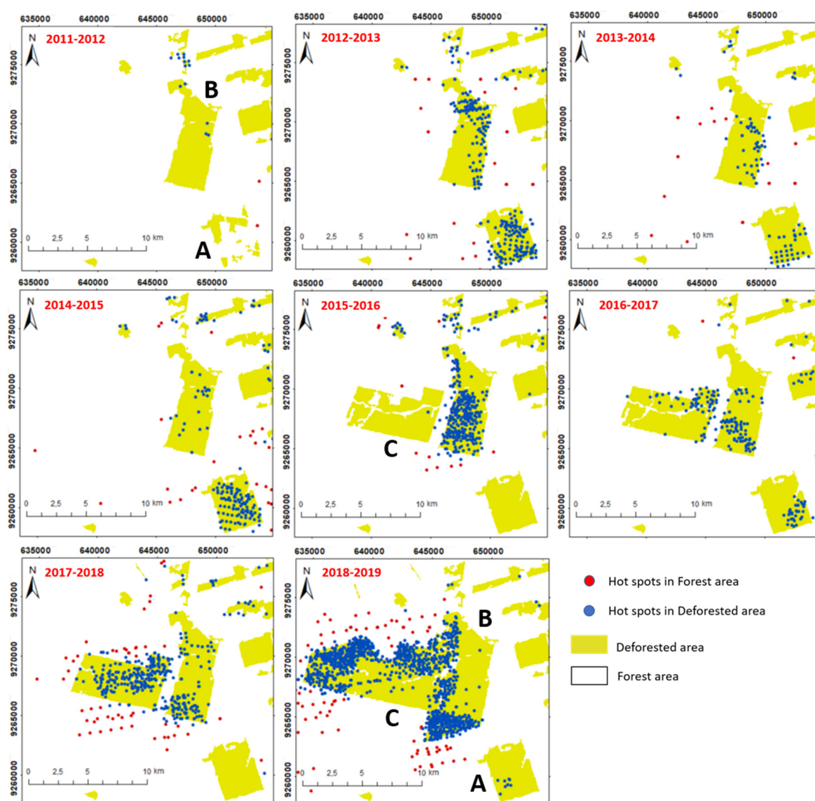
Figure 8. Deforestation dynamics from PY2011–2012 to PY2018–2019 in a portion of the Novo Progresso region. The figure, from upper-left to low-right, shows the yearly evolution of hotspots related to deforestation in deforested (blue dots) and forested (red dots) areas.
