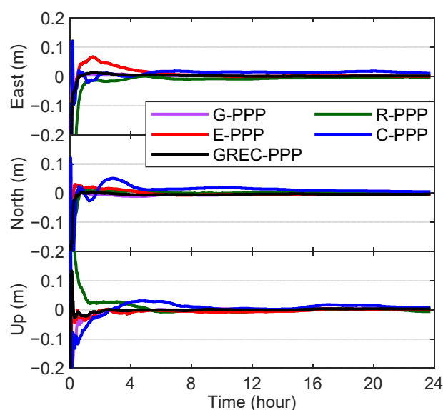
Figure 11. Epoch-wise position errors of static PPP using CNES real-time precise products at station KIR0 on 17 May 2020.
