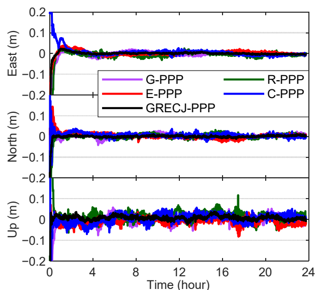
Figure 12. Epoch-wise position errors of kinematic PPP using ESA final precise products at station KIR0 on 17 May 2020.
