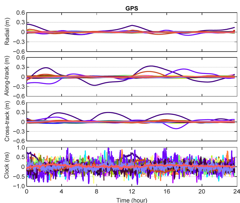
Figure 3. Epoch-wise orbit and clock differences for GPS satellites between GFZ and WHU precise products on DOY 122 of 2020.
