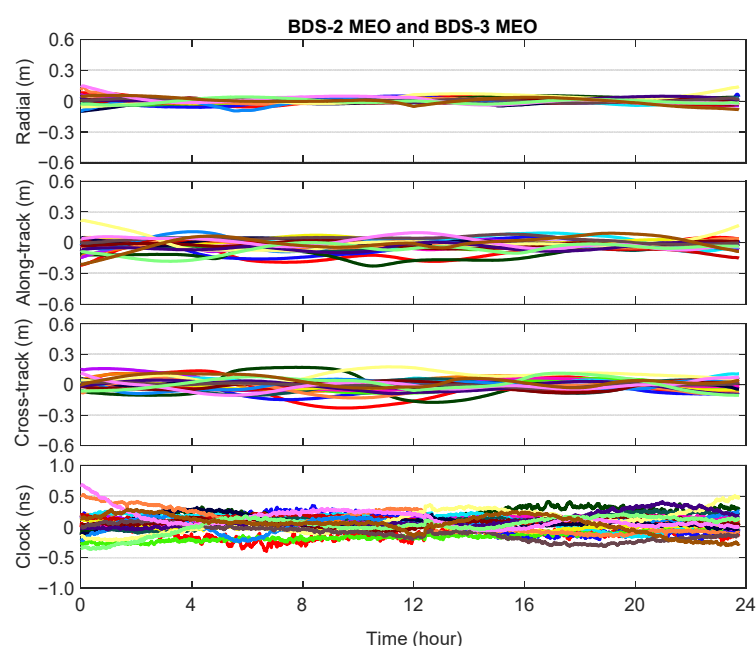
Figure 7. Epoch-wise orbit and clock differences for BDS-2 and BDS-3 MEO satellites between GFZ and WHU precise products on DOY 122 of 2020.
