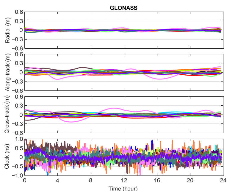
Figure 4. Epoch-wise orbit and clock differences for GLONASS satellites between GFZ and WHU precise products on DOY 122 of 2020.
