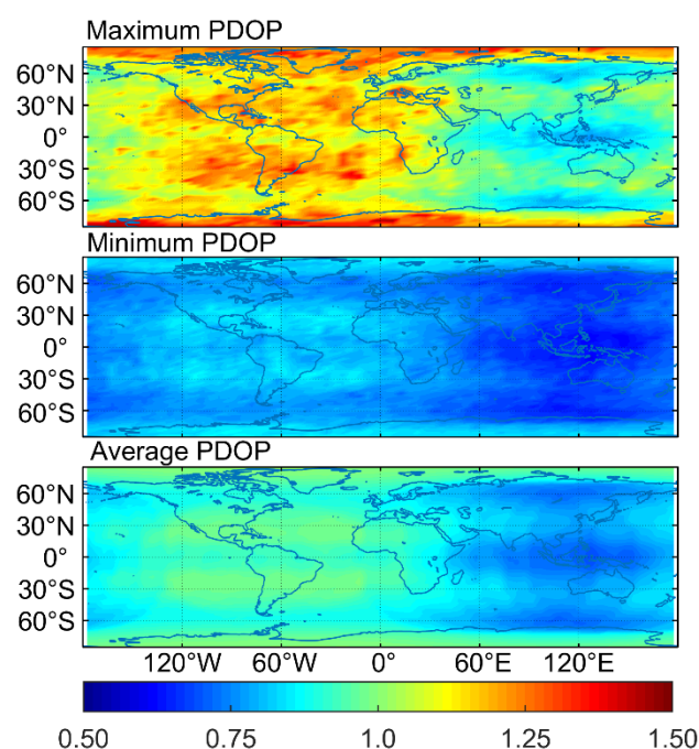
Figure 2. Global maps of maximum, minimum and average PDOP values for five-system combination on DOY 122 of 2020.
