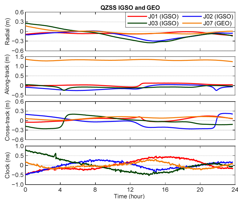
Figure 8. Epoch-wise orbit and clock differences for QZSS GEO and IGSO satellites between GFZ and WHU precise products on DOY 122 of 2020.
