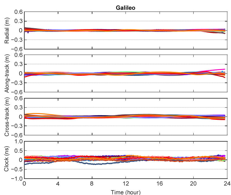
Figure 5. Epoch-wise orbit and clock differences for Galileo satellites between GFZ and WHU precise products on DOY 122 of 2020.
