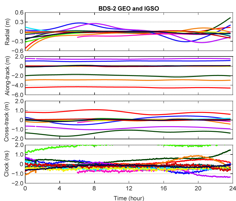
Figure 6. Epoch-wise orbit and clock differences for BDS-2 GEO and IGSO satellites between GFZ and WHU precise products on DOY 122 of 2020.
