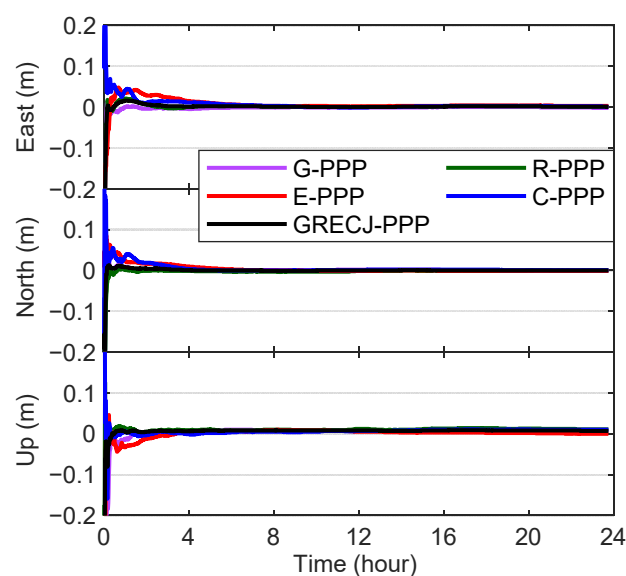
Figure 10. Epoch-wise position errors of static PPP using ESA final precise products at station KIRO on 17 May 2020.
