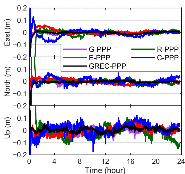
Figure 13. Epoch-wise position errors of kinematic PPP using CNES real-time precise products at station KIR0 on 17 May 2020.
