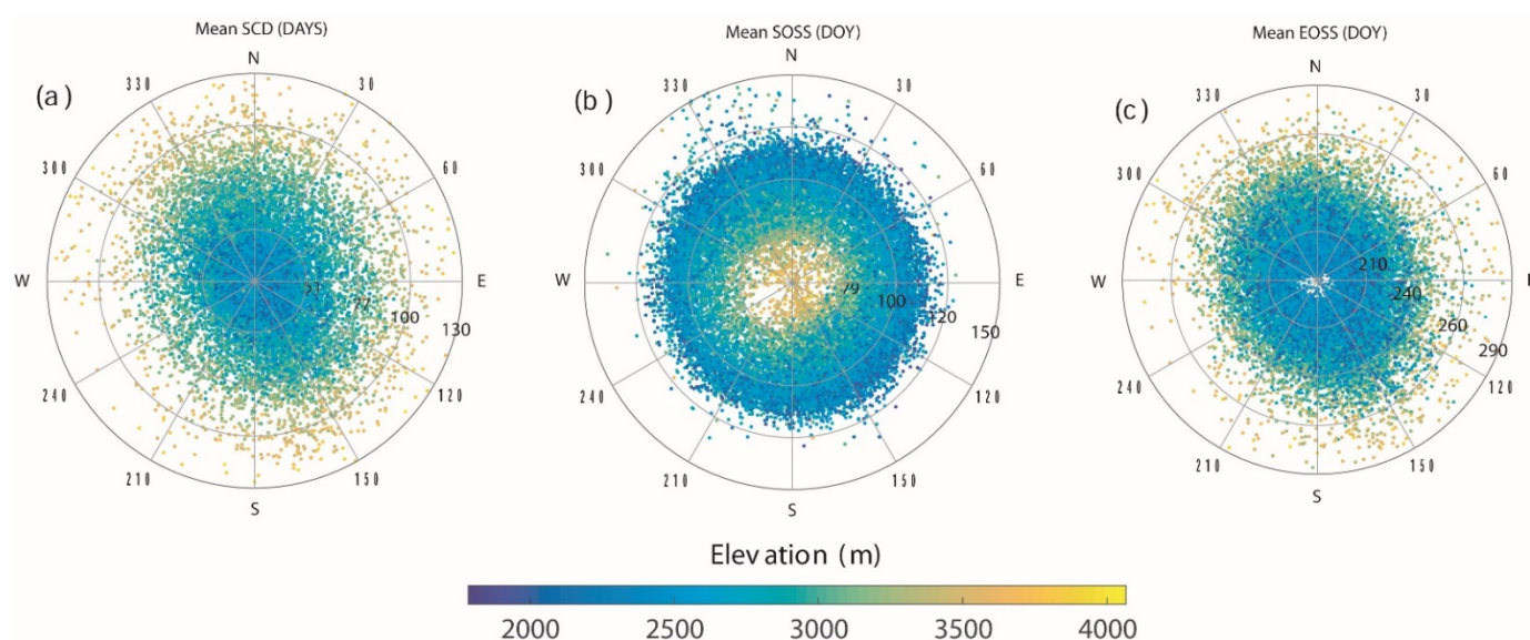
Figure 8. Mean SCD (a), mean SOSS (b), and mean EOSS (c) based on aspect, 2001–2016.
