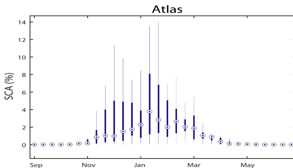
Figure 3. Box plot of the variations in a 10-day fSCA. Area across the snow seasons between 2001 and 2016, Atlas Mountains.
