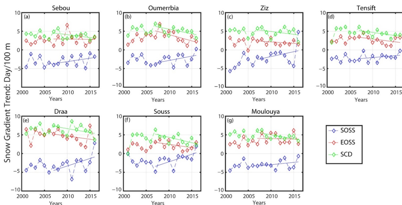
Figure 11. Snow metrics lapse rate (day/100 m) between 2001 and 2016 over the seven river basins.
