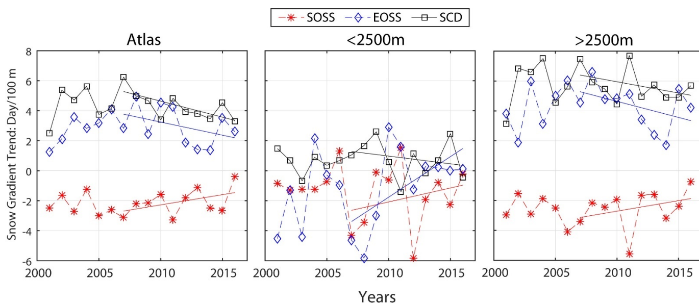
Figure 10. The trend of the snow metrics gradient between 2001 and 2016 over the whole Atlas chain and by altitude range.
