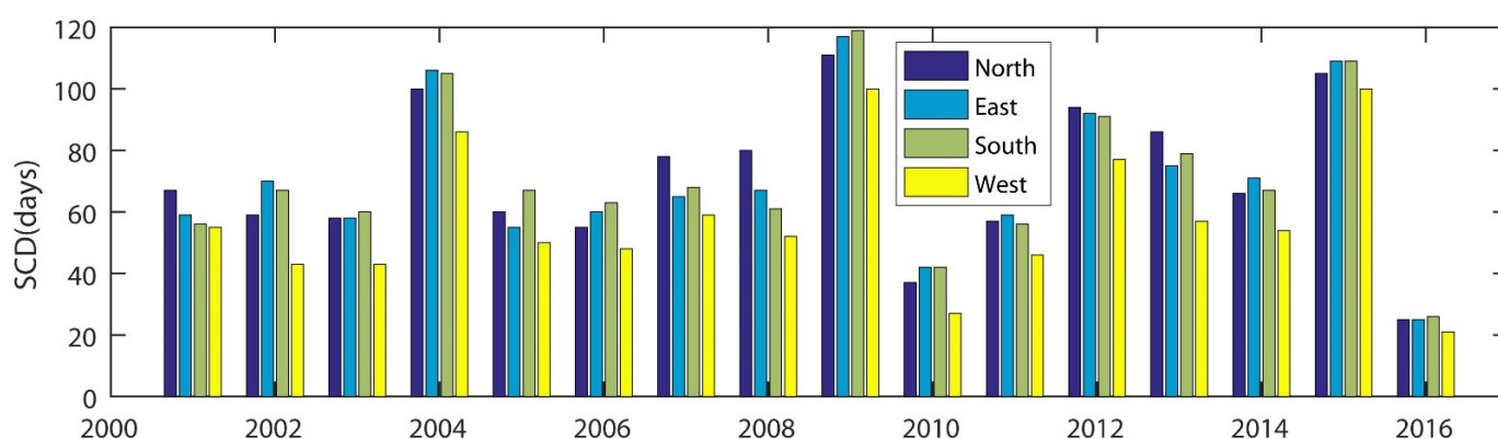
Figure 7. Evolution of the annual SCDs of four aspects in each hydrologic year, from 2001 to 2016, in the Atlas chain.
