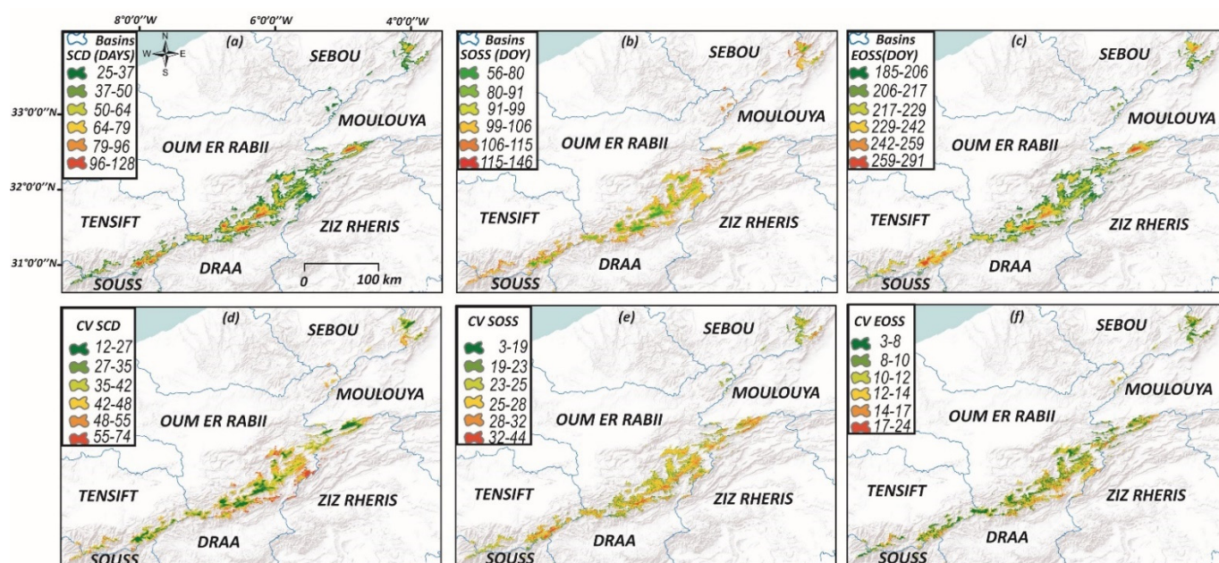
Figure 5. Mean annual snow cover metrics (SCD (a), SOSS (b), and EOSS (c), and associated coefficient of variation (d–f), 2001–2016.
