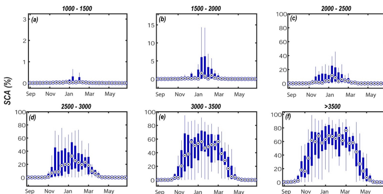
Figure 4. Boxplot of the variations in the 10-day fSCA for the snow seasons between 2001 and 2016, by elevation band: (a) altitudes between 1000 and 1500 m, (b) altitudes between 1500 and 2000 m, (c) altitudes between 2000 and 2500 m, (d) altitudes between 2500 and 3000 m, (e) altitudes between 3000 and 3500 m and (f) altitudes above 3500 m.
