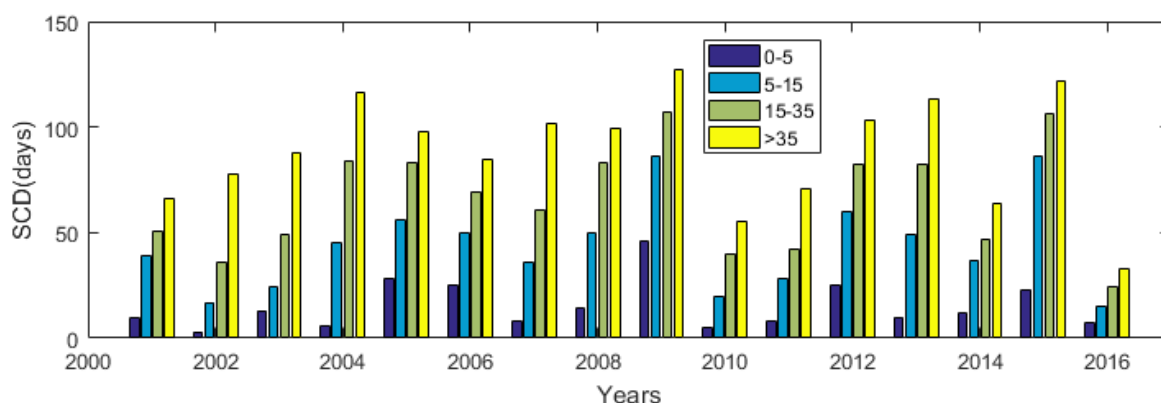
Figure 9. Evolution of annual SCDs of the four slopes from 2001 to 2016 in the Atlas chain.
