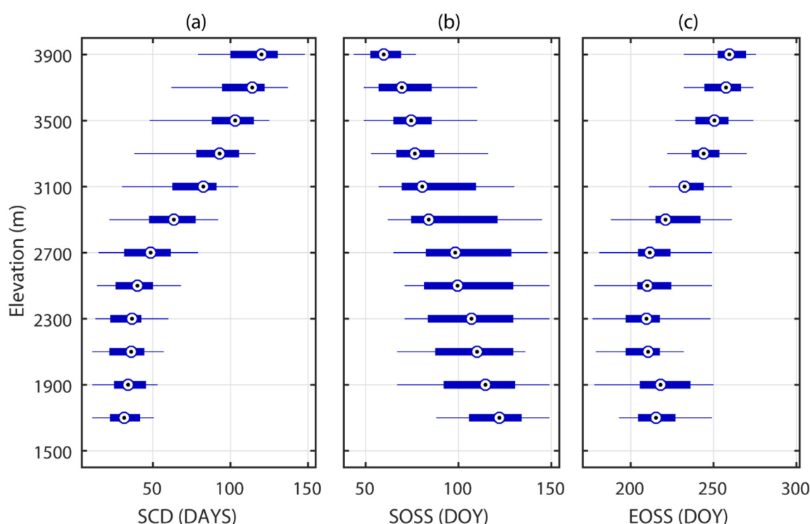
Figure 6. Snow cover metrics based on elevation bands in the Atlas Mountains, 2001–2016. (a) SCD, (b) SOSS, (c) EOSS.
