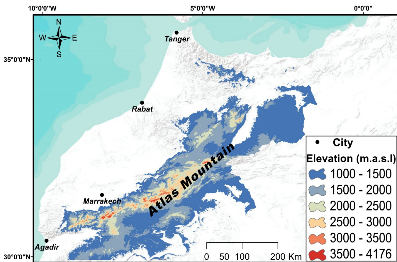
Figure 1. Location of the mountainous area higher than 1000 m in Morocco.
