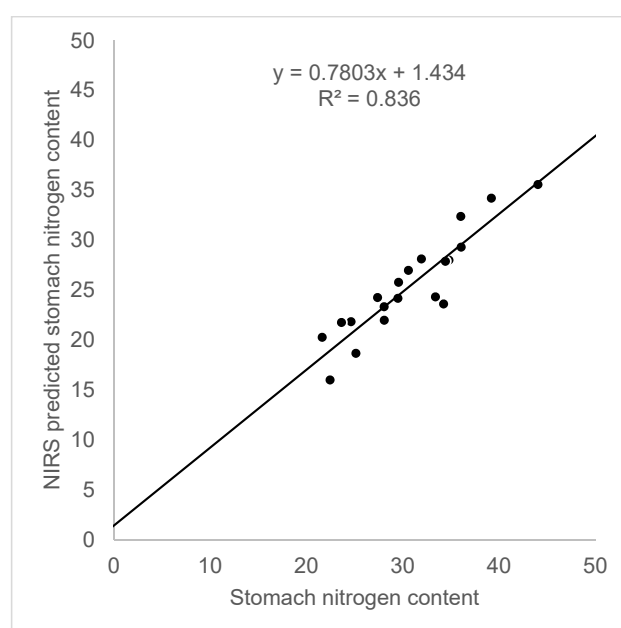
Figure 4. The fit between the nitrogen content in the rodent stomachs determined by a classic chemical analysis and predicted NIRS values.
