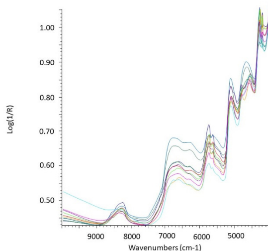
Figure 3. Example of untransformed NIR spectra of rodent stomach contents ( n = 10 ).
