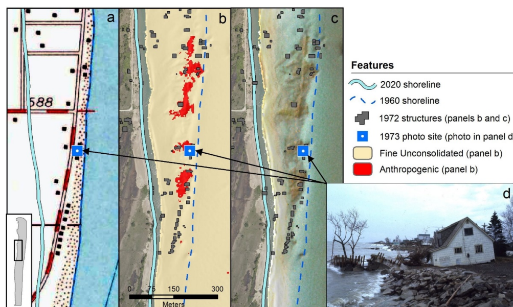
Figure 24. Shoreline changes and destruction of infrastructure illustrated in the central part of the study area as a result of lake level changes between 1960 and 2020: (a) 1960 topographic map obtained from the U.S. Geological Survey [57] showing homes and roads along the shoreline with the superimposed 2020 shoreline (digitized from RGB aerial imagery collected by the JALBTCX in 2020), (b) Tier 1 substrate classification result using airborne data inputs from 17 July 2018, highlighting remnants of various infrastructure found offshore (1973 structures digitized from historic topographic maps, [58]) and classified as anthropogenic substrate (in red), (c) airborne fusion image from 17 July 2018 also illustrating offshore benthic environment, and (d) 1973 photograph showing destruction of a home impacted by the shoreline erosion [59].
