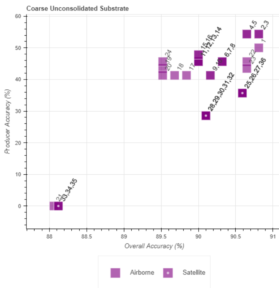
Figure 10. Tier 1 plot of coarse unconsolidated substrate classification performance, comparing percent overall accuracy and percent producer accuracy for airborne and satellite data combinations. Number labels refer to unique classification input data combinations identified in the Index field in Table A1, Appendix A.
