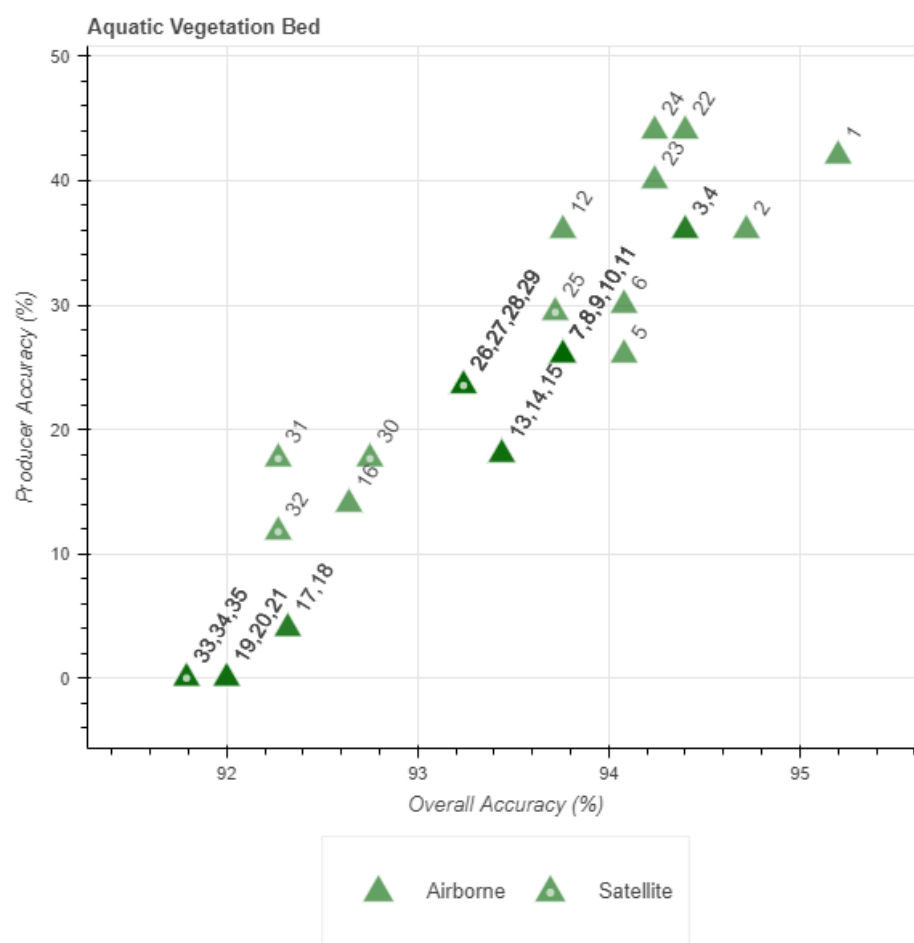
Figure 16. Tier 1 plot of aquatic vegetation bed classification performance, comparing percent overall accuracy and percent producer accuracy for airborne and satellite data combinations. Number labels refer to unique classification input data combinations identified in the Index field in Table A2, Appendix A.
