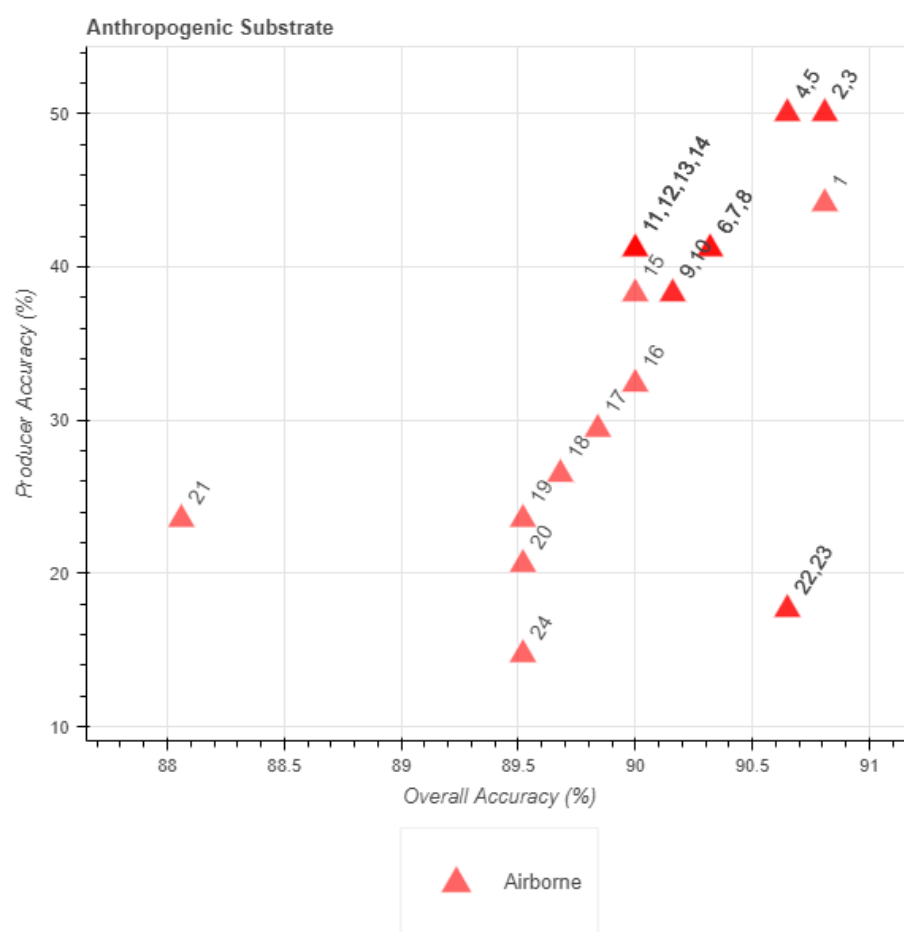
Figure 12. Tier 1 plot of anthropogenic substrate classification performance, comparing percent overall accuracy and percent producer accuracy for airborne only data combinations. Number labels refer to unique classification input data combinations identified in the Index field in Table A1, Appendix A. Note that satellite classification of anthropogenic substrates is not included because the satellite inputs were insufficient for discriminating those features.
