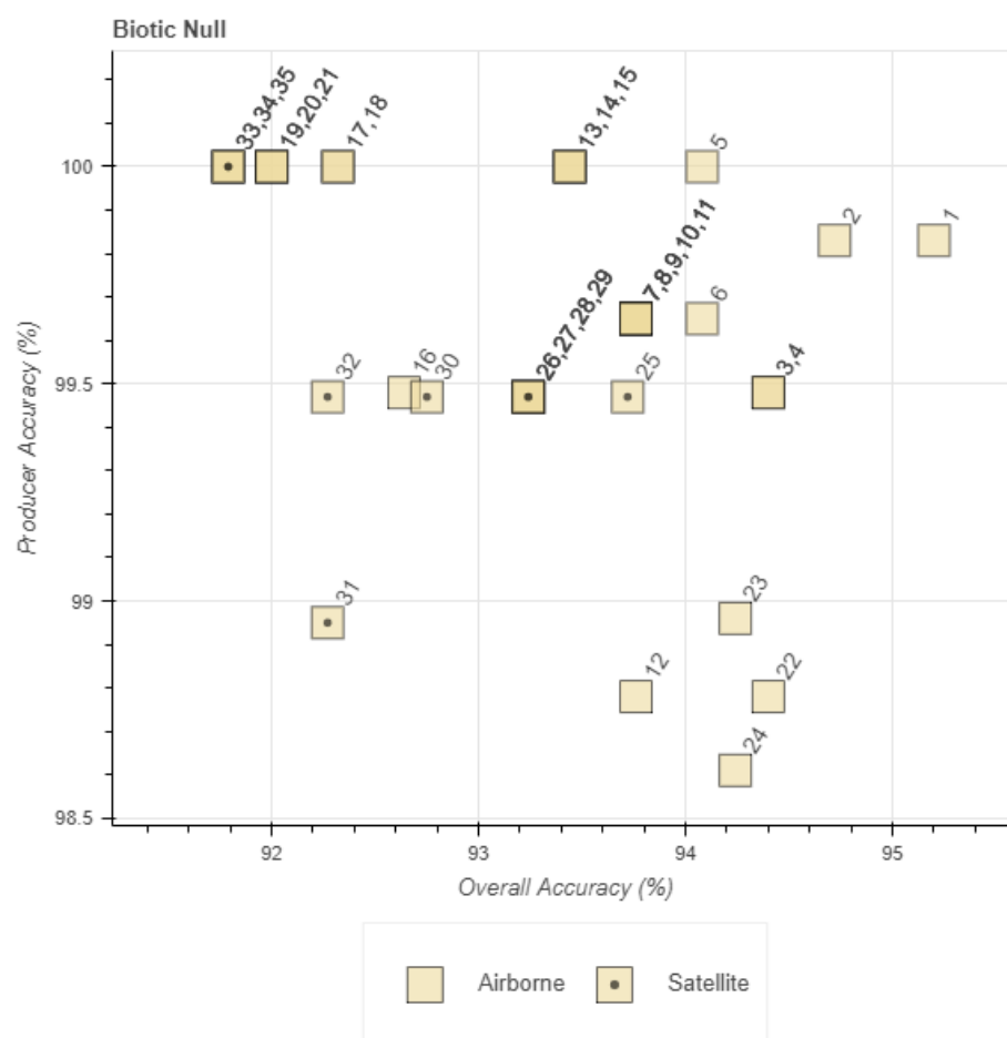
Figure 17. Tier 1 plot of biotic null classification performance, comparing percent overall accuracy and percent producer accuracy for airborne and satellite data combinations. Number labels refer to unique classification input data combinations identified in the Index field in Table A2, Appendix A.
