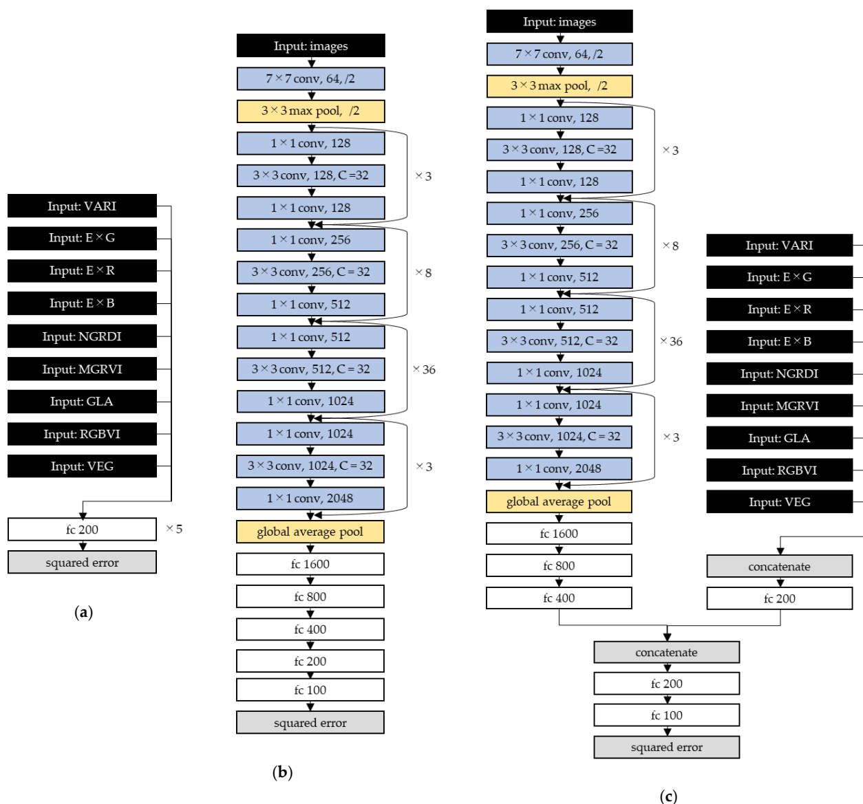
Figure 6. Network architectures for the three patterns of input datasets of DL used in this study: (a) nine types of CIs; (b) RGB images; (c) nine types of CIs and RGB images. “C = 32” indicates grouped convolutions with 32 groups. “7 × 7 conv 64,/2” indicates a convolution layer using 64 kinds of 7 × 7 kernel filter with a stride of 2 pixels. “fc 200” indicates a fully connected layer with 200 outputs.
