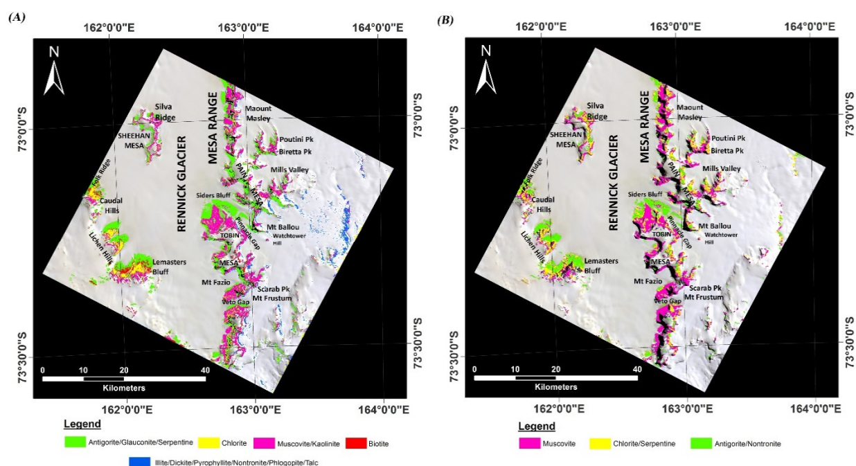
Figure 9. (A) CEM classification mineral map for the Mesa Range scene derived from fraction images of the selected endmember minerals using ASTER VINR+SWIR bands. (B) CEM classification mineral map for the Mesa Range scene derived from fraction images of the selected endmember minerals using ASTER TIR bands.
