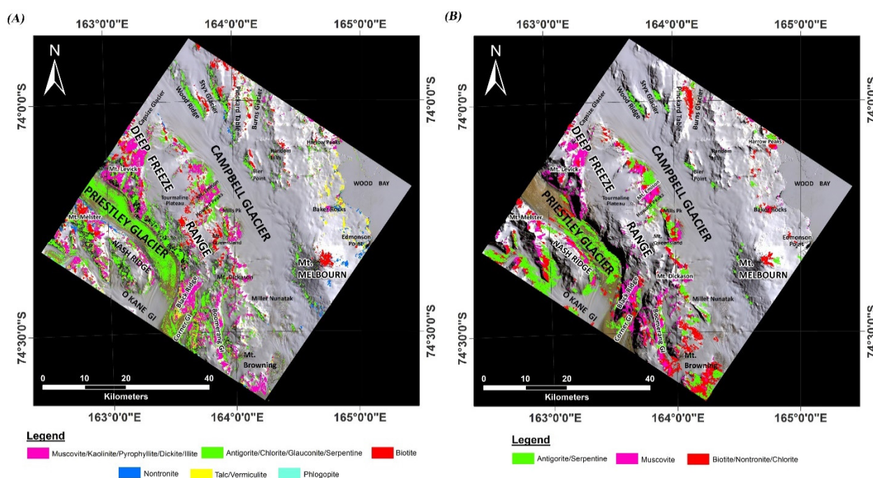
Figure 12. (A) CEM classification mineral map for the Campbell Glacier (II) scene derived from fraction images of the selected endmember minerals using ASTER VNIR+SWIR bands. (B) CEM classification mineral map for the Campbell Glacier (II) scene derived from fraction images of the selected endmember minerals using ASTER TIR bands.
