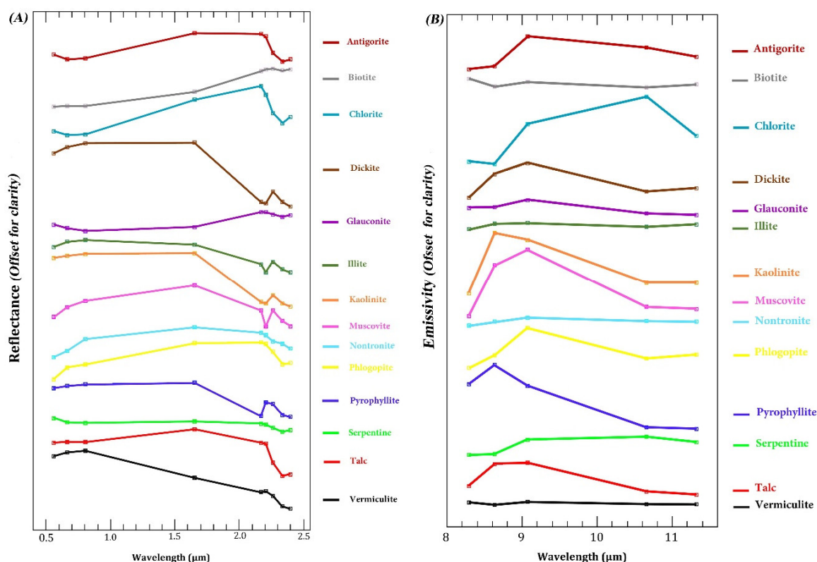
Figure 4. Laboratory reflectance spectra of the selected phyllosilicate minerals re-sampled to response functions of ASTER VNIR+SWIR and TIR bands. (A) ASTER VNIR+SWIR bands; (B) ASTER TIR bands. Cubes indicate the location of the ASTER VNIR+SWIR and TIR bands.
