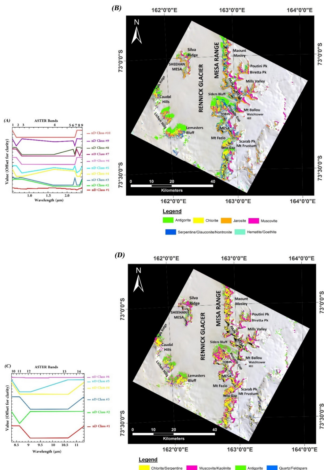
Figure 5. (A) Endmember spectra extracted from ASTER VNIR+SWIR bands using the n-Dimensional analysis technique for the Mesa Range. (B) MTMF classification mineral maps derived from MF score images (VNIR+SWIR bands) for the Mesa Range scene. (C) Endmember spectra extracted from ASTER TIR bands using the n-Dimensional analysis technique for the Mesa Range. (D) MTMF classification mineral maps derived from MF score images (TIR bands) for the Mesa Range scene.
