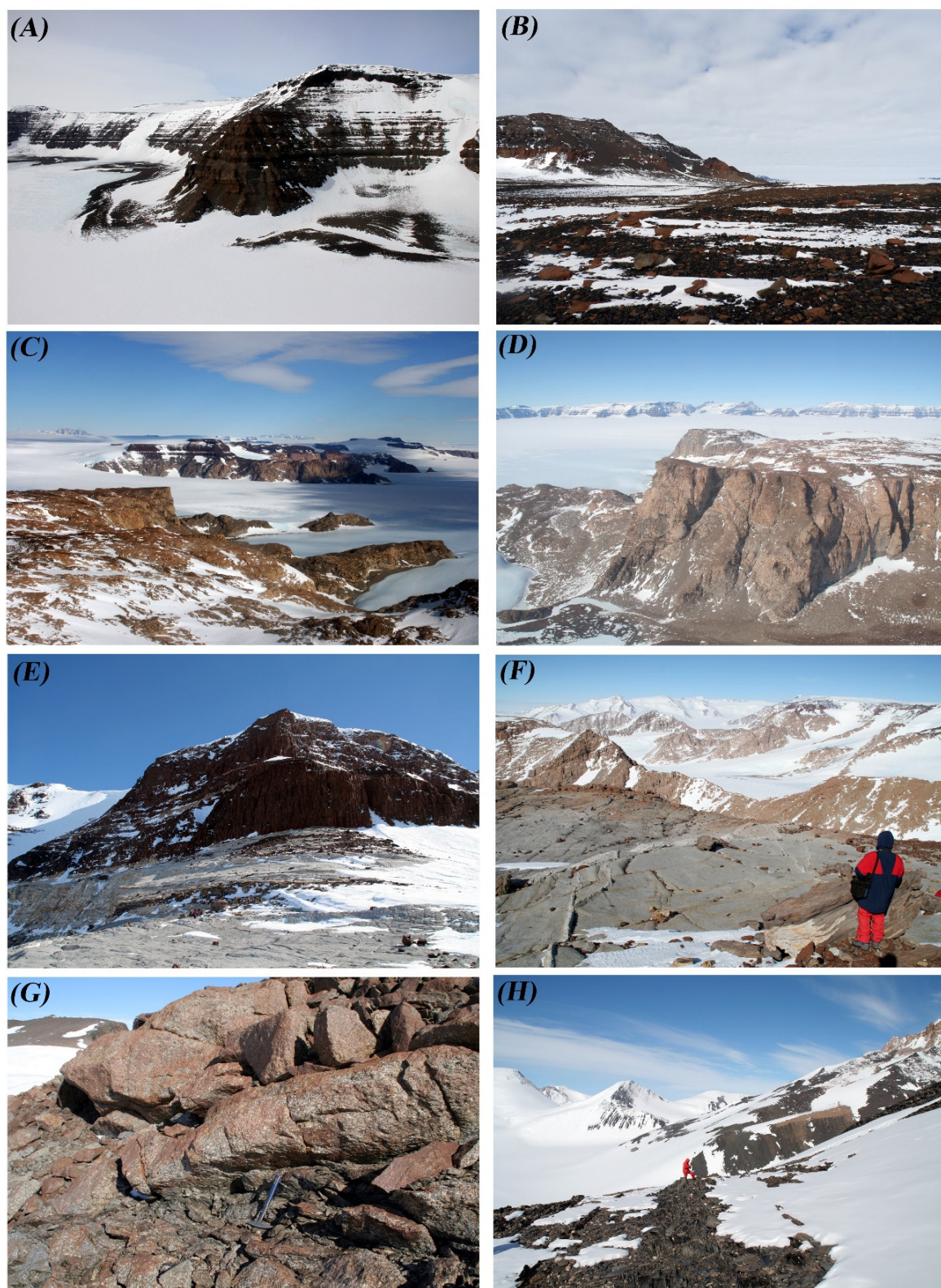
Figure 13. Field photographs of the bedrock lithologies. (A) Helicopter view of Kirkpatrick Basalts (series of lava flows) in the western flank of Tobin Mesa, southern Mesa Range; (B) Regional view of glacial deposits and debris composed of Kirkpatrick Basalts and Ferrar Dolerite associated with zeolite-bearing volcanoclastic and sandstone in southern Mesa Range; (C) Regional view of the exposures of sheeted leucogranite of the Granite Harbour Intrusives and schists of the Wilson Metamorphic Complex and sandstone of the Beacon Supergroup, Lichen Hills, Mesa Range area; (D) Helicopter view of flat hills with steep escarpments of Granite Harbour Intrusives and schists of the Wilson Metamorphic Complex, which is partly covered by weathered erratic and tills on top and debris at the foot of steep slopes, Lichen Hills, Mesa
