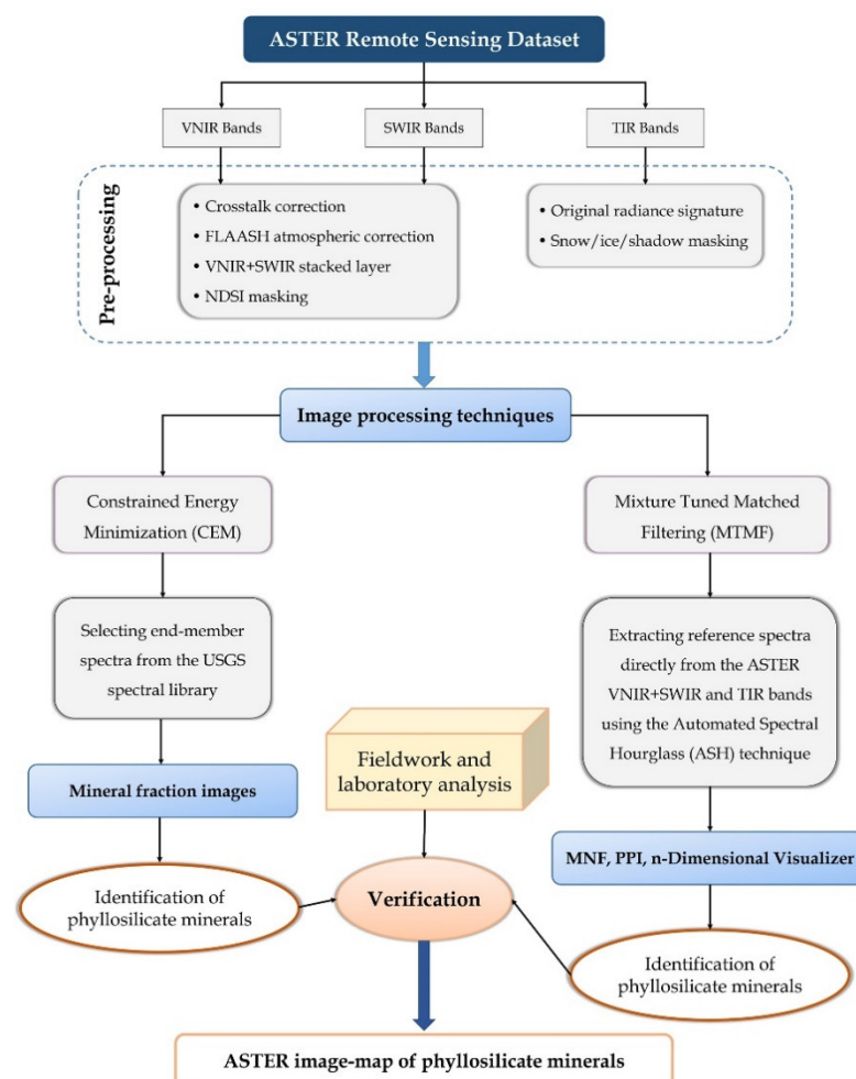
Figure 3. An overview of methodological flowchart used in this study.
