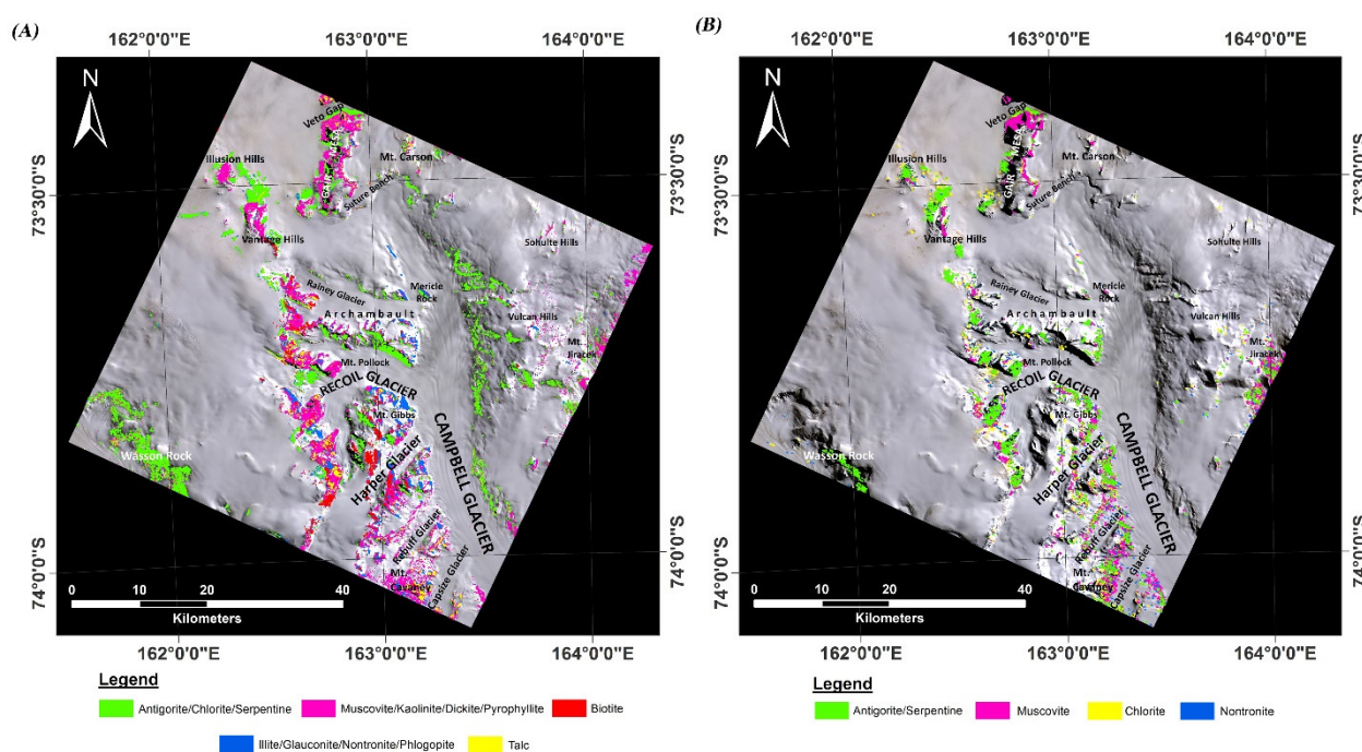
Figure 10. (A) CEM classification mineral map for the Campbell Glacier (I) scene derived from fraction images of the selected endmember minerals using ASTER VINR+SWIR bands. (B) CEM classification mineral map for the Campbell Glacier (I) scene derived from fraction images of the selected endmember minerals using ASTER TIR bands.
