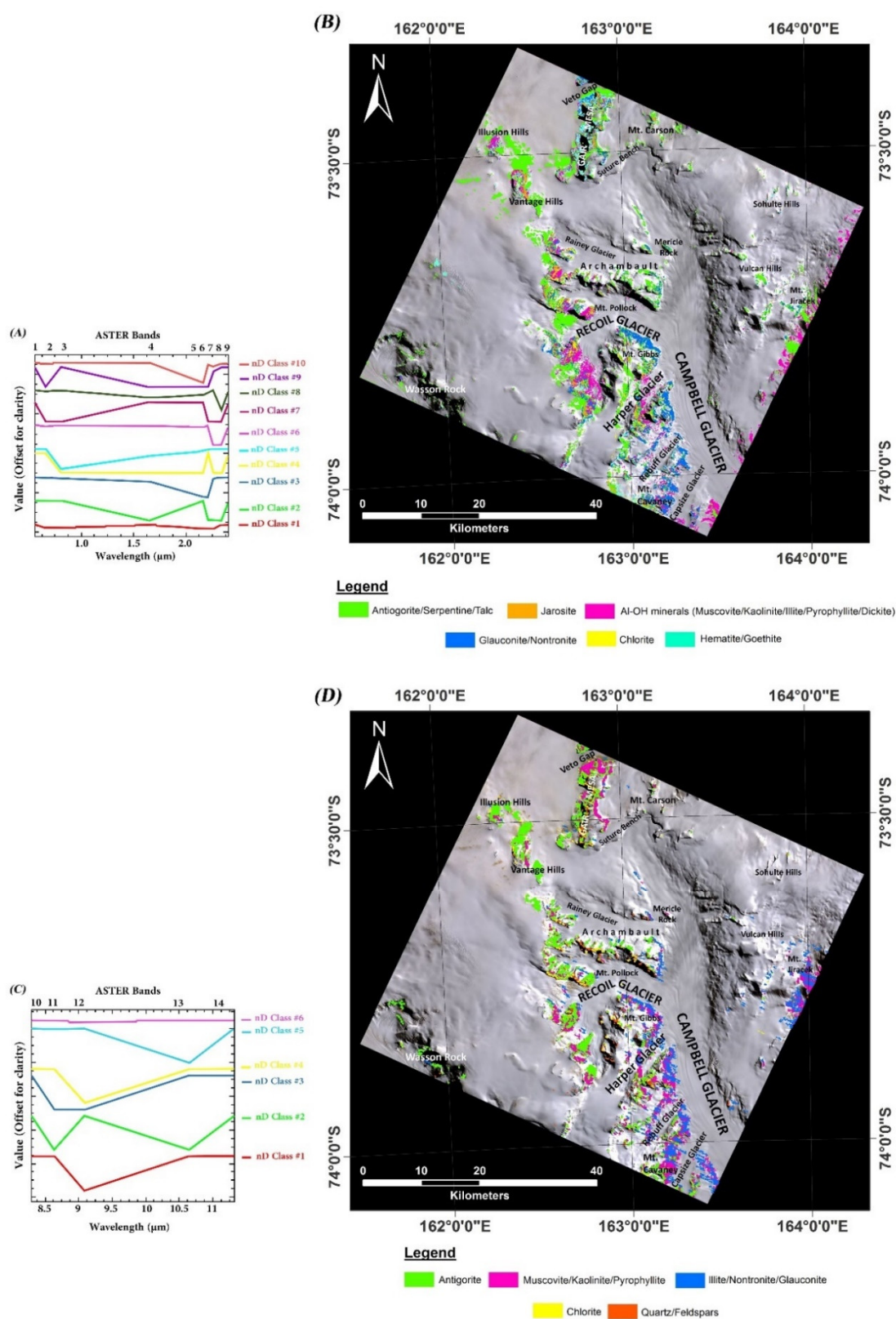
Figure 6. (A) Endmember spectra extracted from ASTER VINR+SWIR bands using the n-Dimensional analysis technique for the Campbell Glacier (I). (B) MTFM classification mineral maps derived from MF score images (VINR+SWIR bands)
