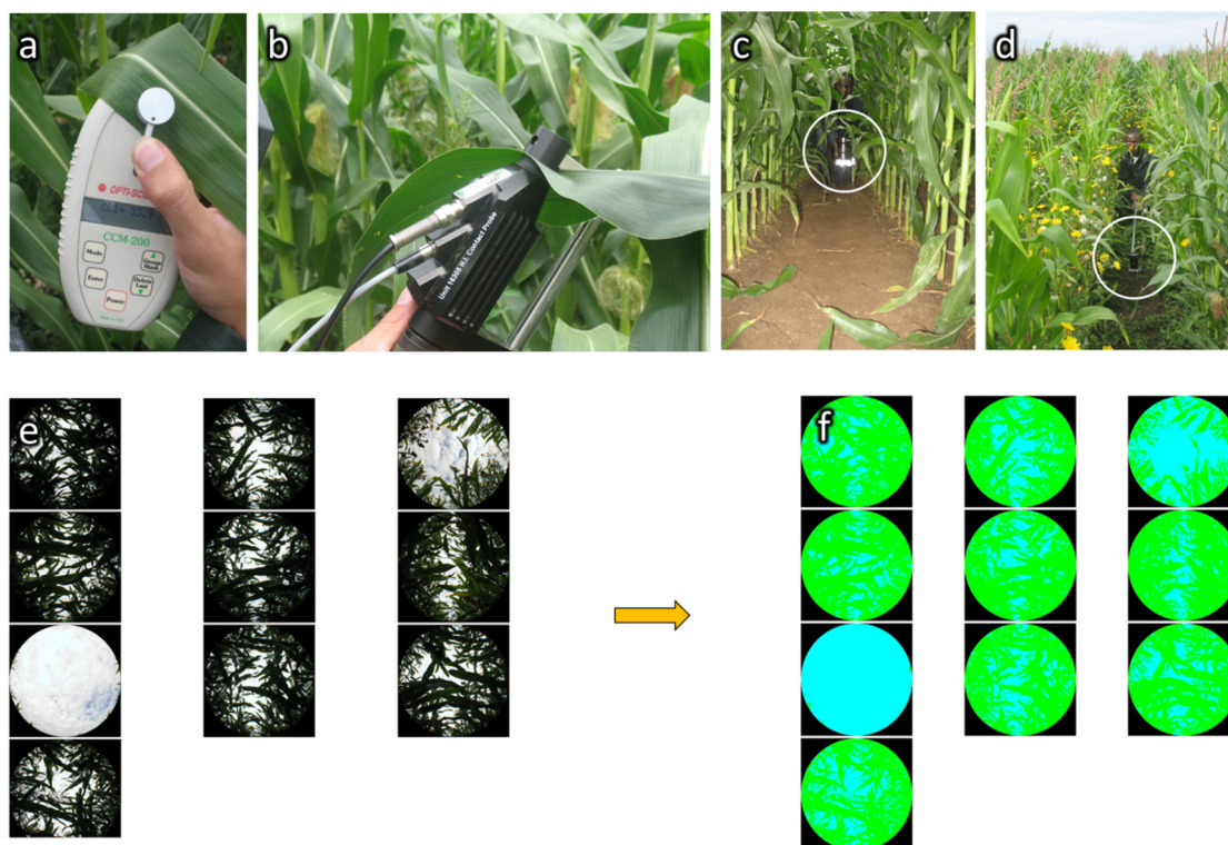
Figure 3. Illustrations of three types of in situ parameter measurements. (a) Chlorophyll content measurement on a conventional maize leaf with a Chlorophyll Content Meter CCM200; (b) Hyperspectral reflectance measurement on a conventional maize leaf with an high intensity contact probe of an Analytical Spectral Device (ASD) FieldSpec3 spectroradiometer equipped with a leaf clip; (c-d-e-f) Hemispherical pictures for the Plant Area Index (PAI) and Fraction of Absorbed Photosynthetically Active Radiation (FAPAR) measurements in conventional (c) and organic (d) maize fields and sample of corresponding raw (e) and classified (f) pictures for an organic maize field.
