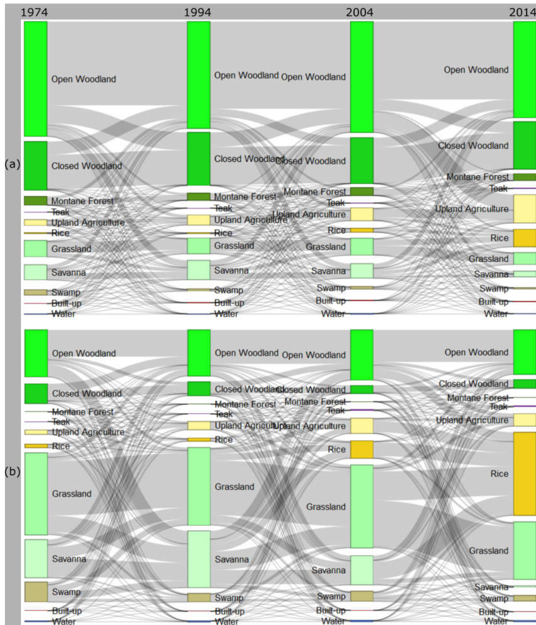
Figure 10. Sankey plots of the LULC changes (a) within the whole Kilombero catchment, and (b) within the Kilombero Ramsar site.
