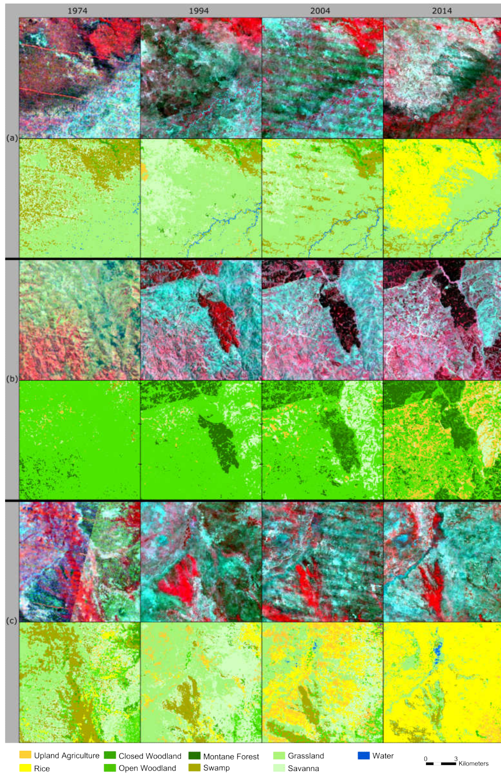
Figure 7. Details of the classification for three different locations (a, b, c). Each upper row shows RGB false color composites (mean NIR – mean red – mean green), the lower rows show the respective classification result. (a) Conversion of a swamp at the northern margins of the Kilombero floodplain to agricultural land (here: rice). (b) Forest plantation in the western part of the catchment. (c) Conversion of swamps, floodplain grassland, and savanna to cropland used for rice cultivation (southern part of the floodplain). Even though some artifacts are visible, the RF classifier is capable of producing consistent and useful maps. Only a few isolated pixels are visible.
