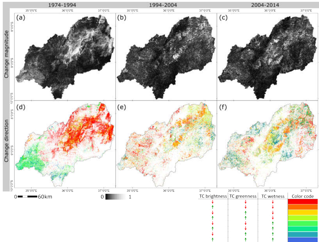
Figure 8. Robust change vector analysis (RCVA)-based spectral change detection results: change magnitude (a–c), and change direction (d–f). Change direction is indicated only in places where change magnitude exceeds a threshold (TC = tasseled cap).
