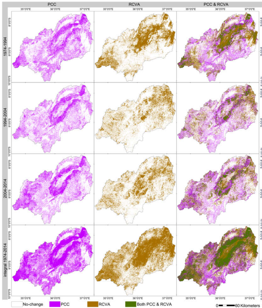
Figure 9. Post-classification comparison (PCC)-based (left) and spectral (center column) changes, and overlay of both (right). The bottom row shows the overlay of all periods (i.e., 1974–2014); the bottom right plot shows the overlay of all periods and both methods. White areas experienced no change, magenta areas denote PCC-based changes, brown areas show RCVA-based spectral changes, and green areas show both PCC and spectral changes.
