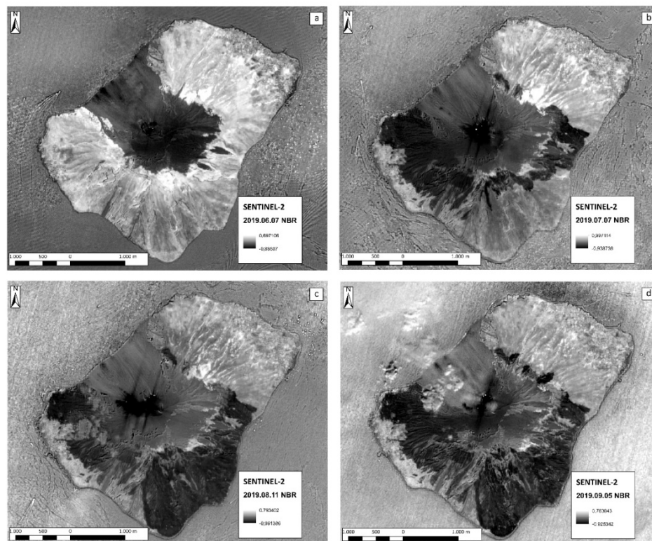
Figure 4. Sentinel-2 images-derived NBR on: (a) 7 th June 2019 (pre-eruption), (b) 7 th July 2019, (c) 11 th August 2019, (d) 5 th September 2019. Thermal (black) anomalies in the summit area and Sciarra del Fuoco in (b), and (c), are related to the effusive activity.
