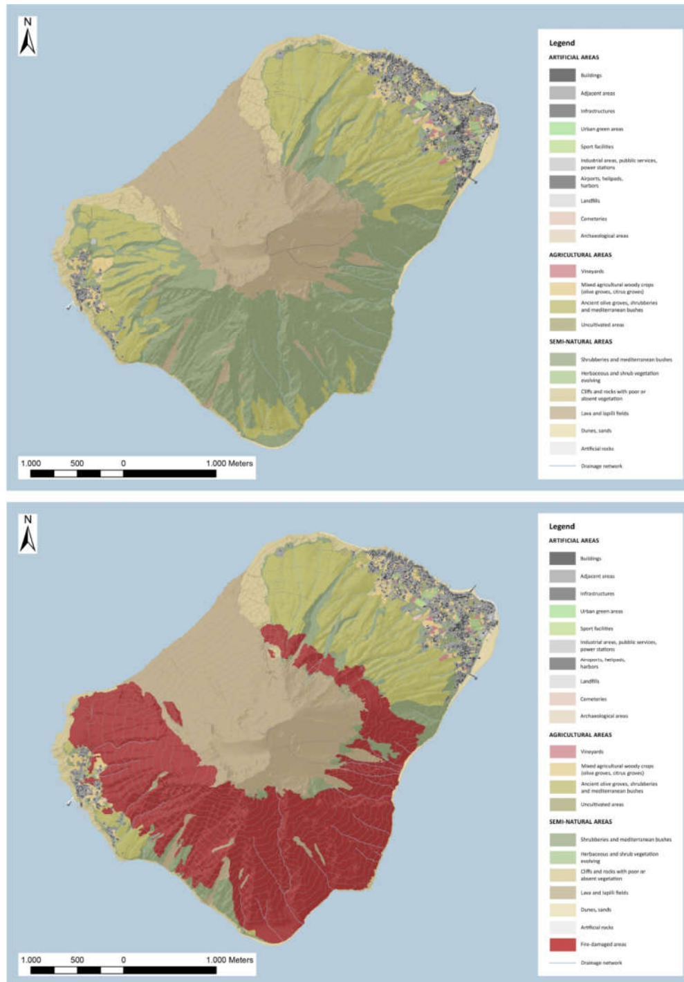
Figure 7. Land use map (LU) pre-eruption (2018) and post-eruption (2019).
