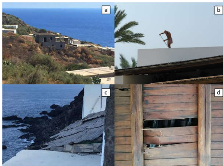
Figure 8. Tephra accumulation on the roofs in (a) and (b), damages to the canopies in (c) and (d) at Ginostra, following the 3 rd July 2019 paroxysmal explosion.
