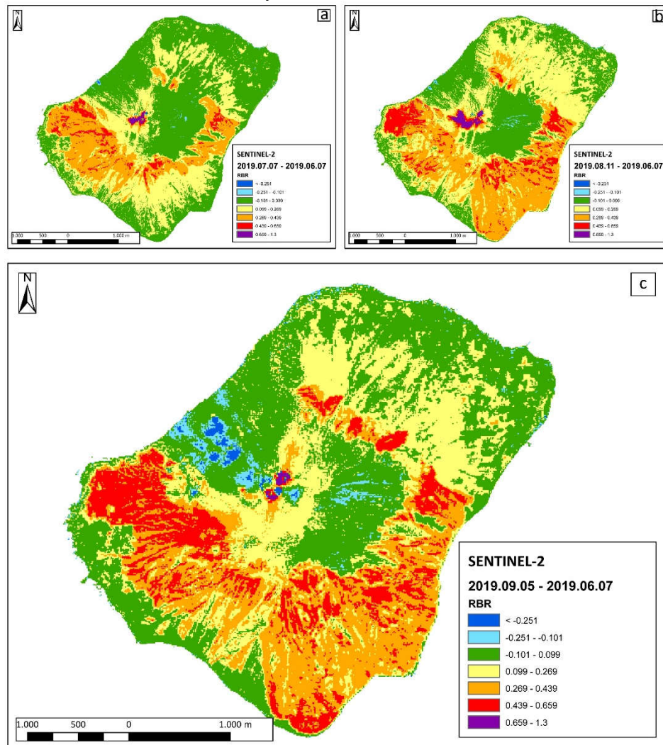
Figure 5. Sentinel-2 images-derived Relativized Burn Ratio (RBR) on: (a) 7 th June 2019 – 7 th July 2019, (b) 7 th June 2019 – 11 th August 2019, (c) 7 th June 2019 – 5 th September 2019.
