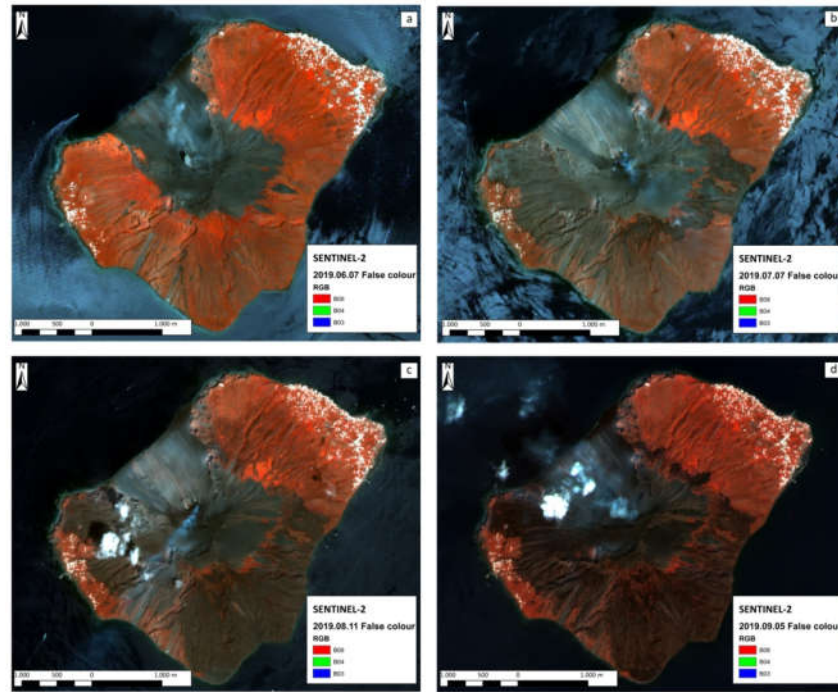
Figure 2. Sentinel-2 image (false color) collected on: (a) 7 th June 2019 (pre-eruption), (b) 7 th July 2019, (c) 11 th August 2019, (d) 5 th September 2019.
