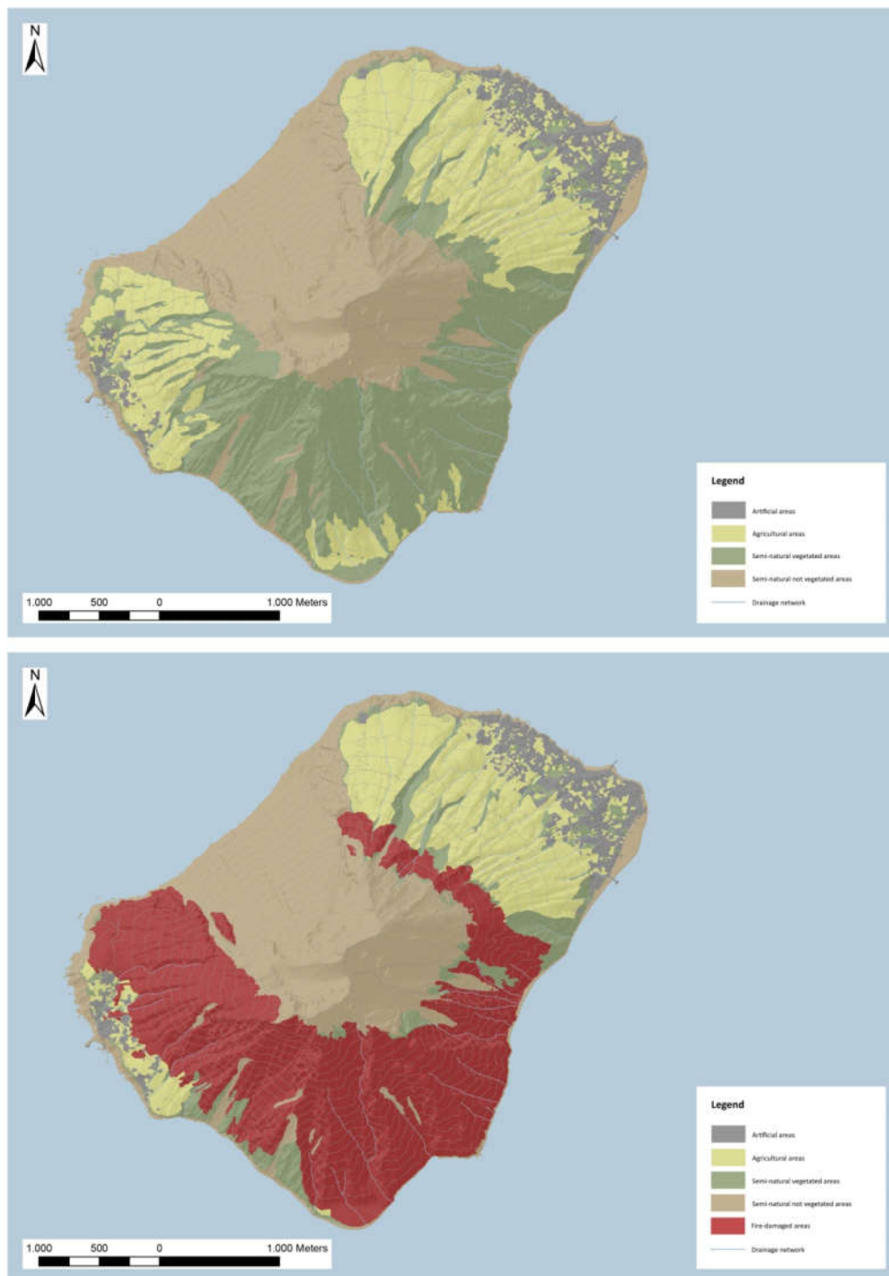
Figure 6. Land cover map (LC) pre-eruption (2018) and post-eruption (2019).
