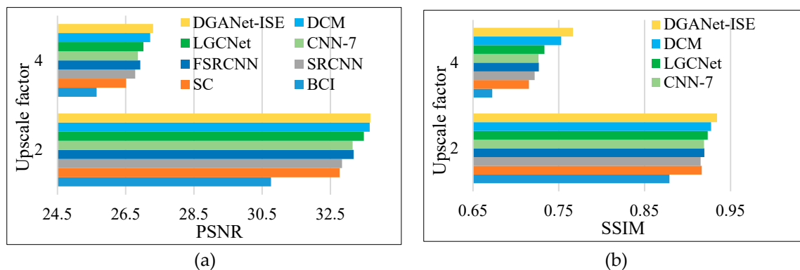
Figure 5. Peak signal-to-noise ratio (PSNR) and structural similarity index (SSIM) comparison results using the UCMerced data set. (a) PSNR results of different methods; (b) SSIM results of different methods.
