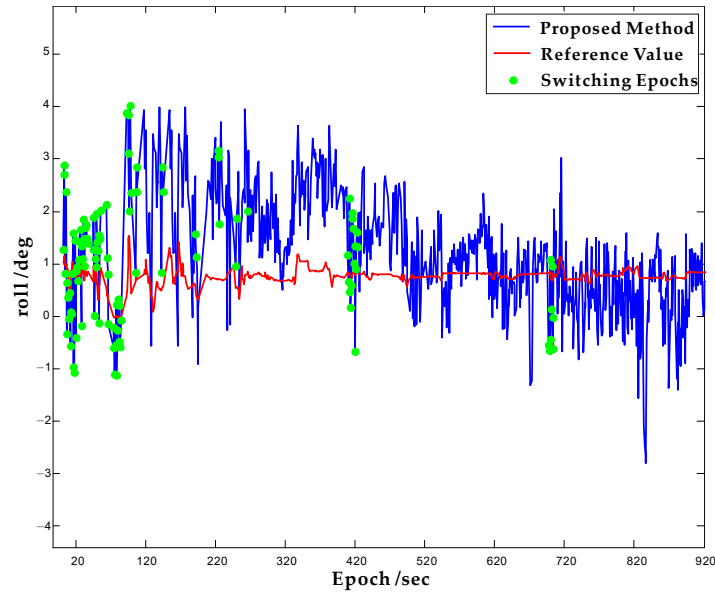
Figure 11. The result of roll angle.
