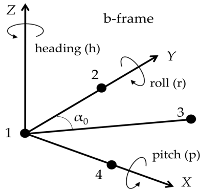
Figure 1. Baselines layout in the direct method and three attitude angles.
