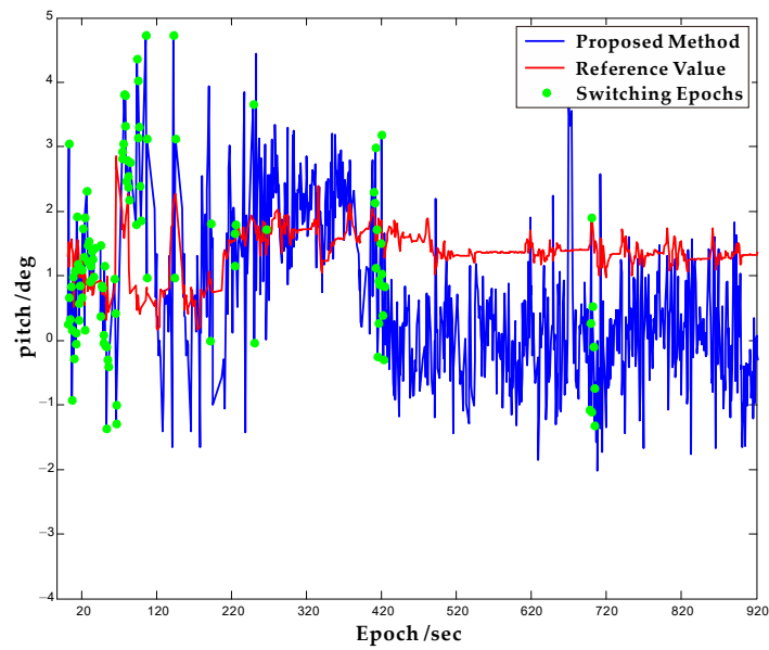
Figure 10. The result of pitch angle.
