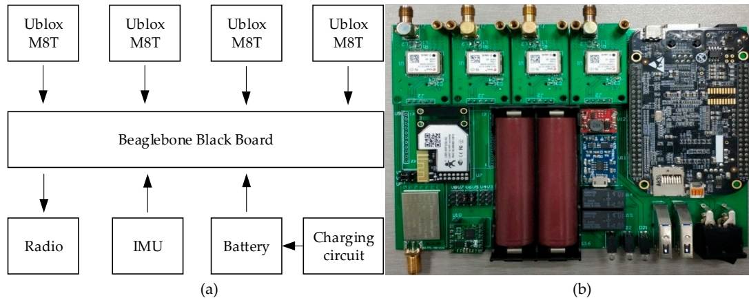
Figure 4. The schematic and physical diagram of the platform.(a) Schematic diagram; (b) Physical diagram.
