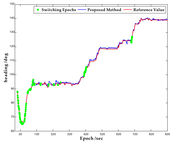
Figure 9. The result of heading angle.
