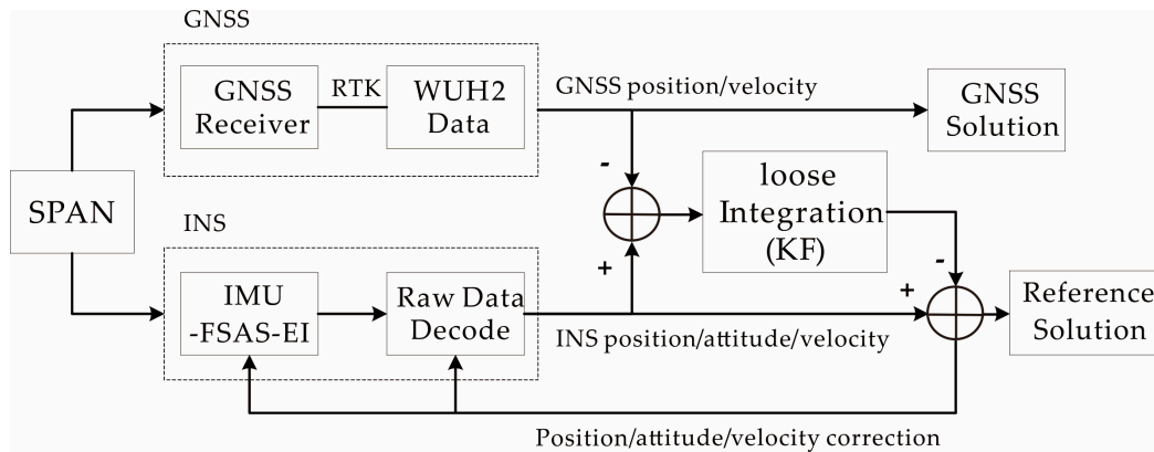
Figure 7. The acquisition process of reference coordinates and attitude.
