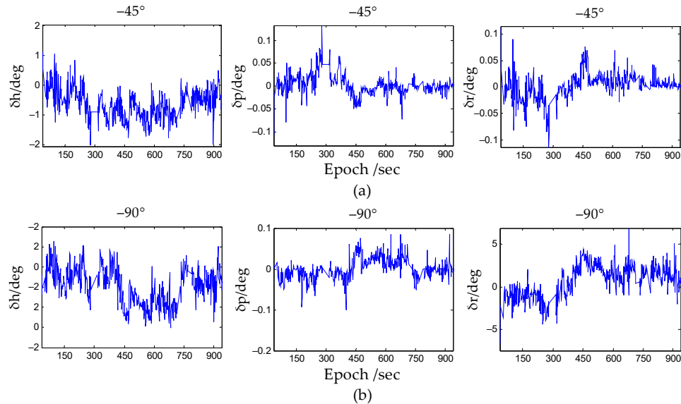
Figure 8. (a) Difference between the results of the -45^\circ baseline and 0^\circ baseline; (b) Difference between the results of the -90^\circ baseline and 0^\circ baseline.
