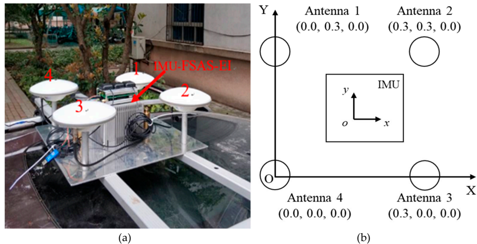
Figure 5. Hardware platform diagram.(a) Hardware platform installation; (b) Antennas and IMU layout.
