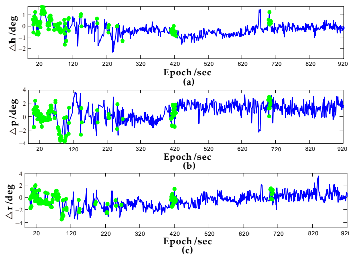
Figure 13. (a) Error statistics of heading angle; (b) Error statistics of pitch angle; (c) Error statistics of roll angle
