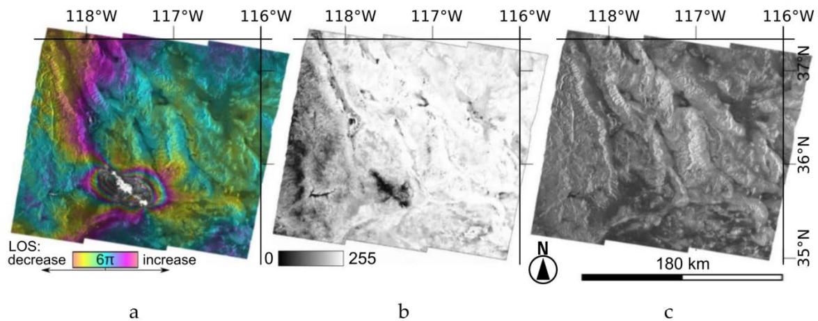
Figure 10. Additional LiCSAR interferometric products over Ridgecrest earthquake (4 July 2019) of frame 071D_05377_131313 (epochs from 4 and 16 July 2019): (a) co-seismic unwrapped phase, (b) coherence image (values stored in 8 bits) and (c) radar intensity image from a post-seismic epoch.
