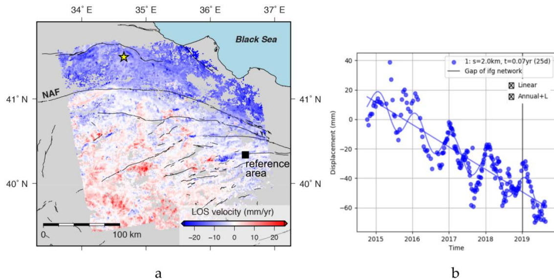
Figure 11. Line of sight (LOS) velocity map and time series for frame 014A_04939_131313, which corresponds to a region around the North Anatolian Fault (NAF). (a) Velocity map with active faults [67]. Black square is the reference area used for the velocity field determination. Yellow star is the location of the time series shown in (b). (b) Displacement time series from the location corresponding to the yellow star in (a) relative to the reference area. The best-fit linear and annual seasonal trends are overlain on the time series. The sizes of the spatial and temporal filters are 2 km and 25 days, respectively.
