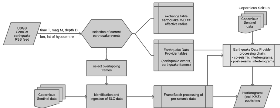
Figure 6. LiCSAR Earthquake Interferometric Synthetic Aperture Radar (InSAR) Data Provider processing flowchart. The system leads to the generation of co-seismic and post-seismic interferograms initiated by ingesting information about current earthquakes from the United States Geological Survey (USGS) ComCat service.
