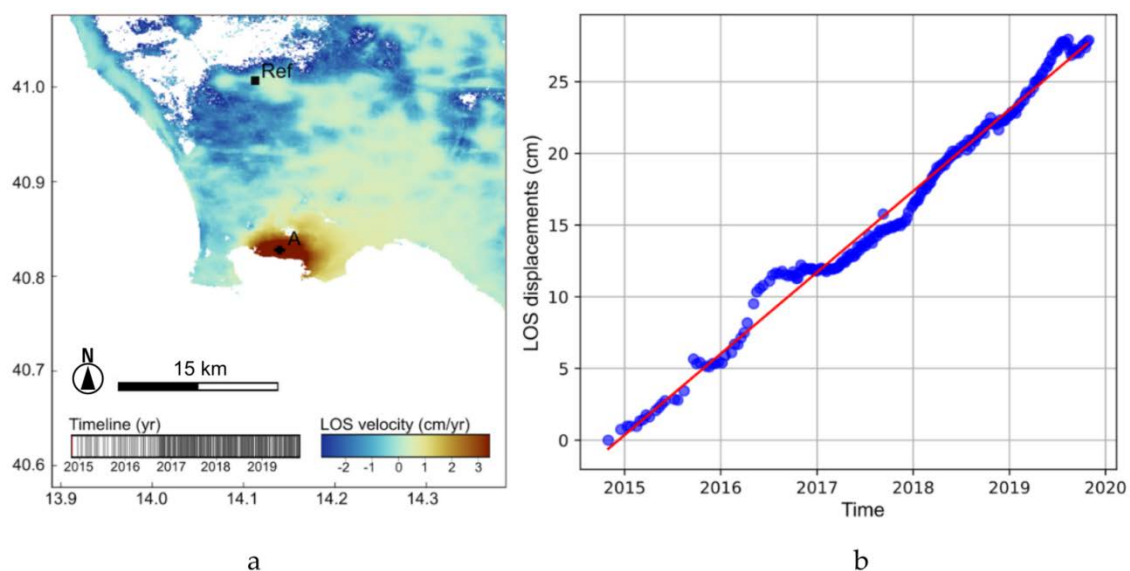
Figure 14. LiCSBAS InSAR time series derived from LiCSAR products showing (a) the LOS velocity map generated for the Campi Flegrei area (frame ID 022D_04826_121209) and (b) the displacement time-series for point A, centered on the caldera, with respect to the reference area located ~20 km north of the caldera.
