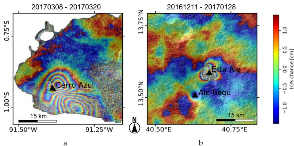
Figure 12. Descending wrapped interferograms generated by the LiCSAR system showing ground deformation associated with (a) the March 2017 intrusion at Cerro Azul and (b) the January 2017 intrusion at Erta Ale.
