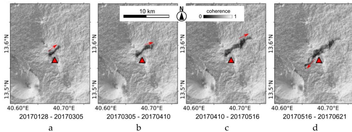
Figure 13. Coherence time series at Erta Ale showing the emplacement of the lava flow during the early stage of the 2017 eruption, from InSAR combinations (having 36-days temporal difference) between: (a) 20170128–20170305, (b) 20170305–20170410, (c) 20170410–20170516, (d) 20170516–20170621. The red triangle locates the volcanic edifice and the red arrows indicate the direction of propagation of the lava flow for each period.
