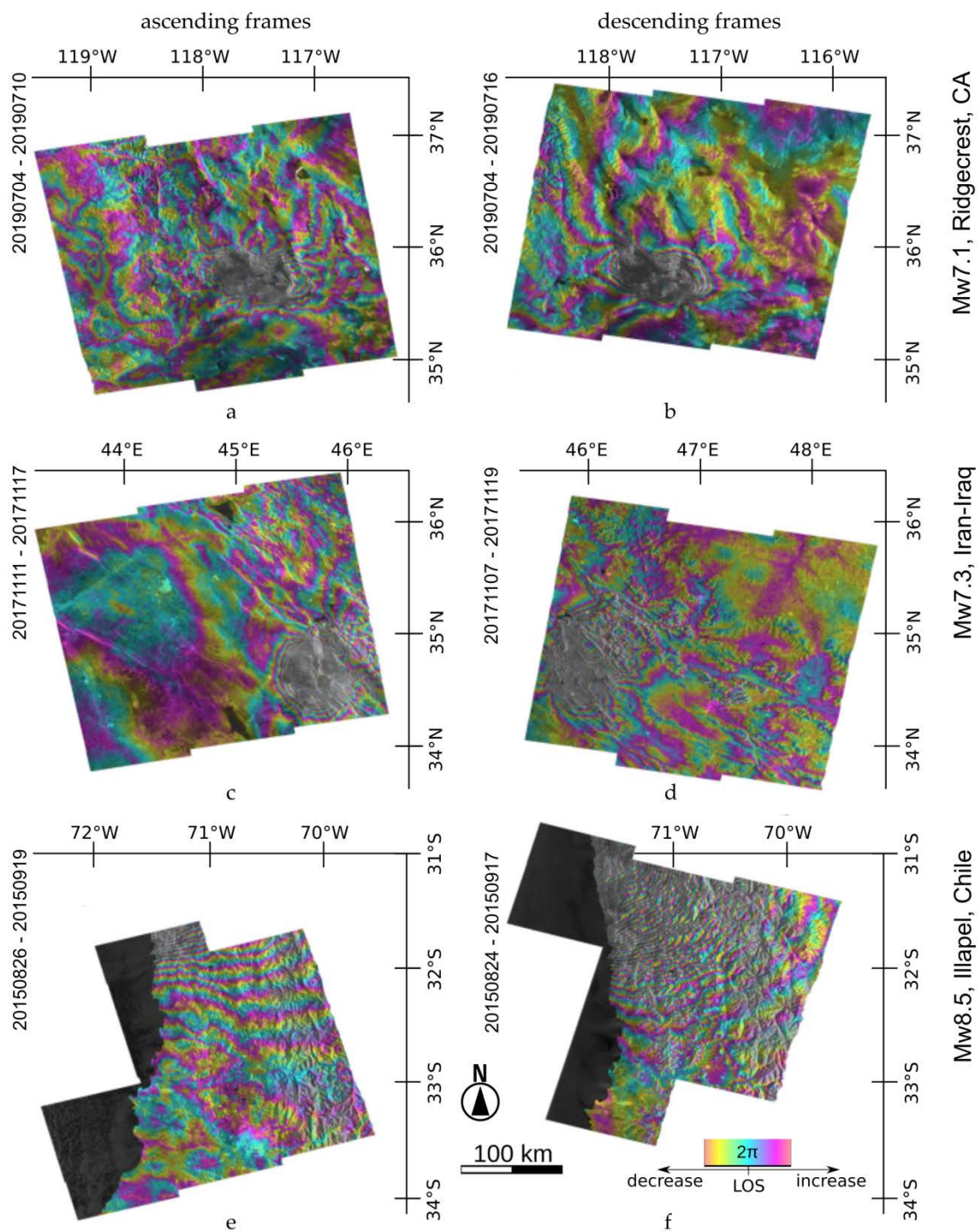
Figure 9. Coseismic interferograms generated in both ascending ( left ) and descending ( right ) orbital tracks of Sentinel-1 by the LiCSAR processor for: M_w 7.1 right-lateral, strike-slip earthquake in Ridgecrest, California (4 July 2019) from (a) frame 064A_05410_131313 and (b) frame 071D_05377_131313; M_w 7.3 dip-slip earthquake at the Iran–Iraq border (12 November 2017) from (c) frame 072A_05489_131313 and (d) frame 006D_05509_131313; and M_w 8.3 dip-slip earthquake in Illapel, Chile (16 September 2015) from (e) frame 018A_12301_061311 and (f) frame 156D_12184_101305. Note that the deformation from the Illapel earthquake covers too large an area to be completely captured in a single Sentinel-1 frame.
