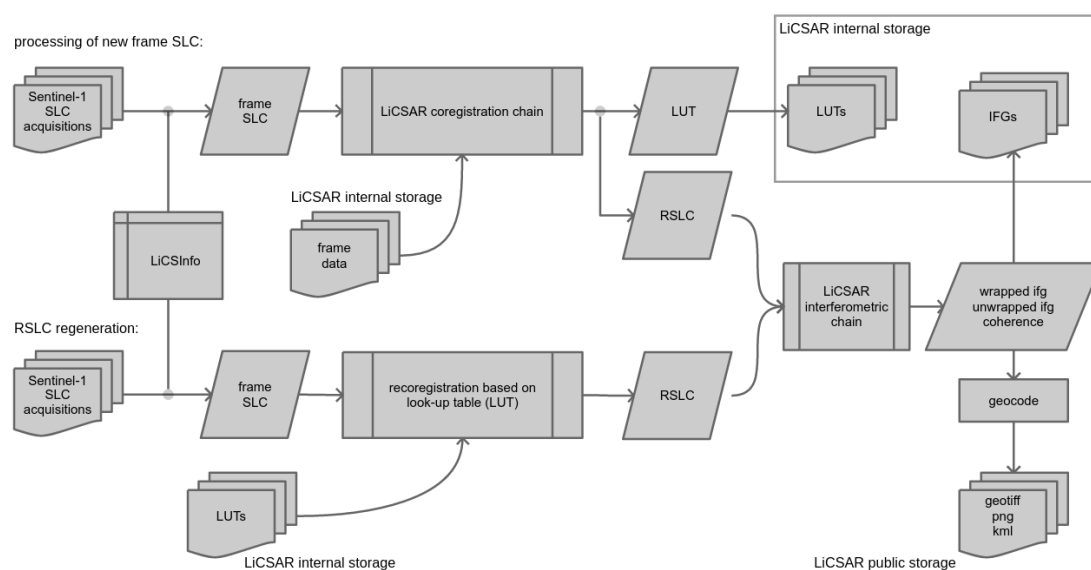
Figure 2. General flowchart of the LiCSAR processing chain.
