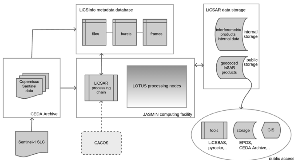
Figure 1. General overview of Looking Into Continents from Space with Synthetic Aperture Radar (LiCSAR) system architecture: interconnections between storage and computing structures leading the path from Sentinel-1 SLC acquisition to publicly accessible geocoded interferometric products.
