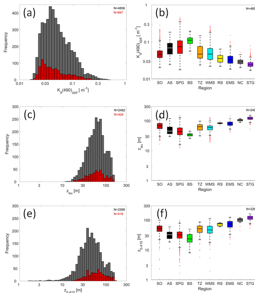
Figure 4. Histogram and boxplot of the distribution of the (a) and (b) near surface diffuse attenuation coefficient at 490 nm ( K_d(490)_{zpd} ), (c) and (d) euphotic layer depth ( z_{eu} ), (e) and (f) and isolume depth
