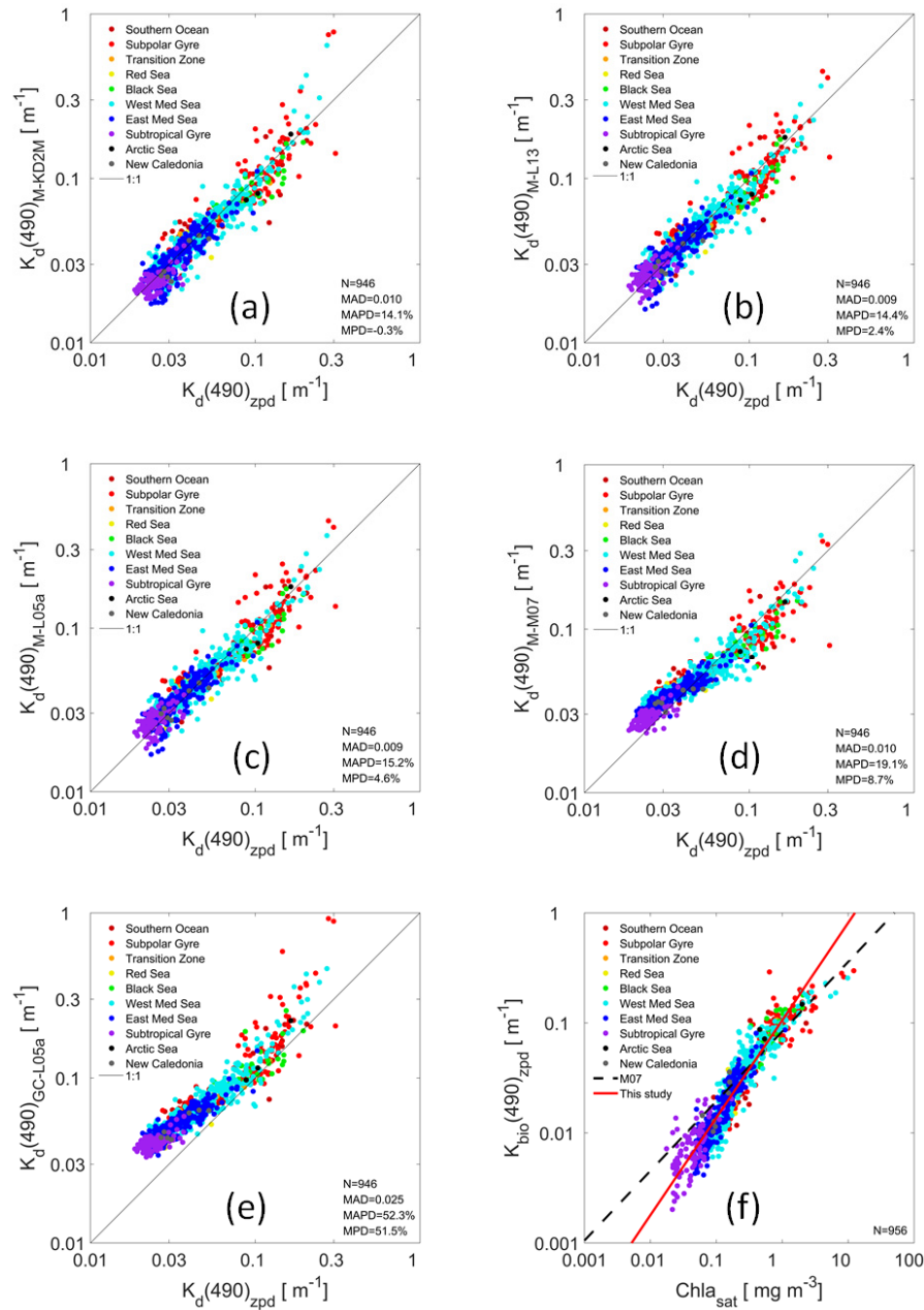
Figure 5. Assessment of satellite K_d(490) products based on BGC-Argo dataset.
