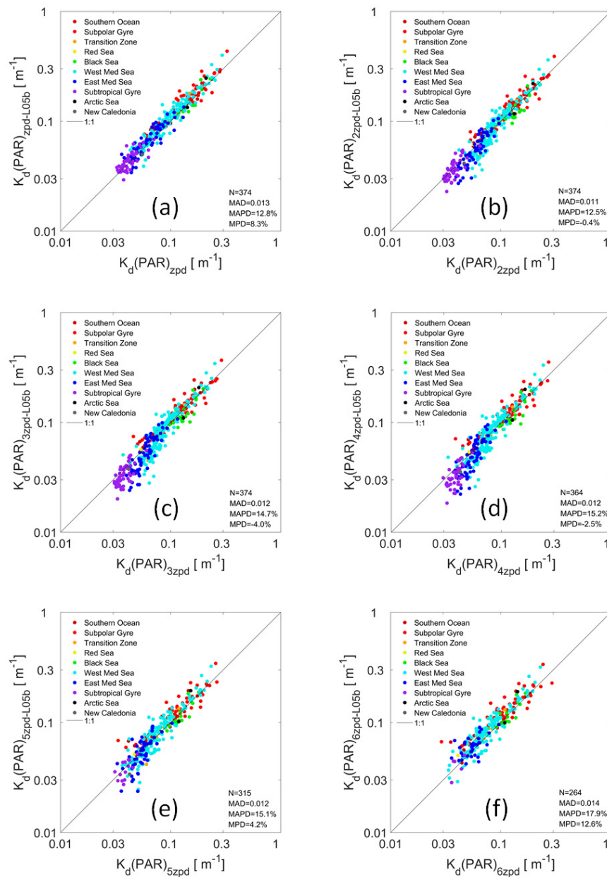
Figure 6. Assessment of satellite K_d(\text{PAR}) products based on BGC-Argo dataset.
