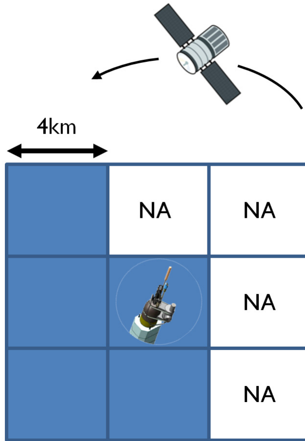
Figure 3. Diagram of a good match-up between satellite and float data.
