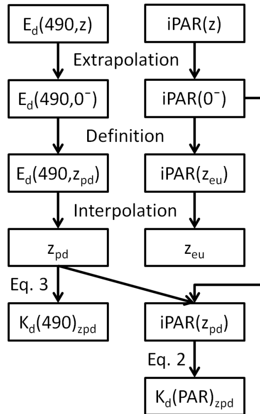
Figure 2. Flow chart of BGC-Argo radiometry data processing.
