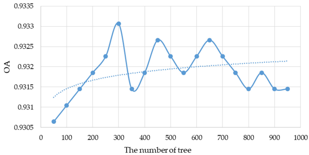
Figure S1. The impact of selection of number of trees in Radom Forest (RF) on classification results. RF models were built with the number of trees ranging from 50 to 950. OA represents Overall Accuracy.
