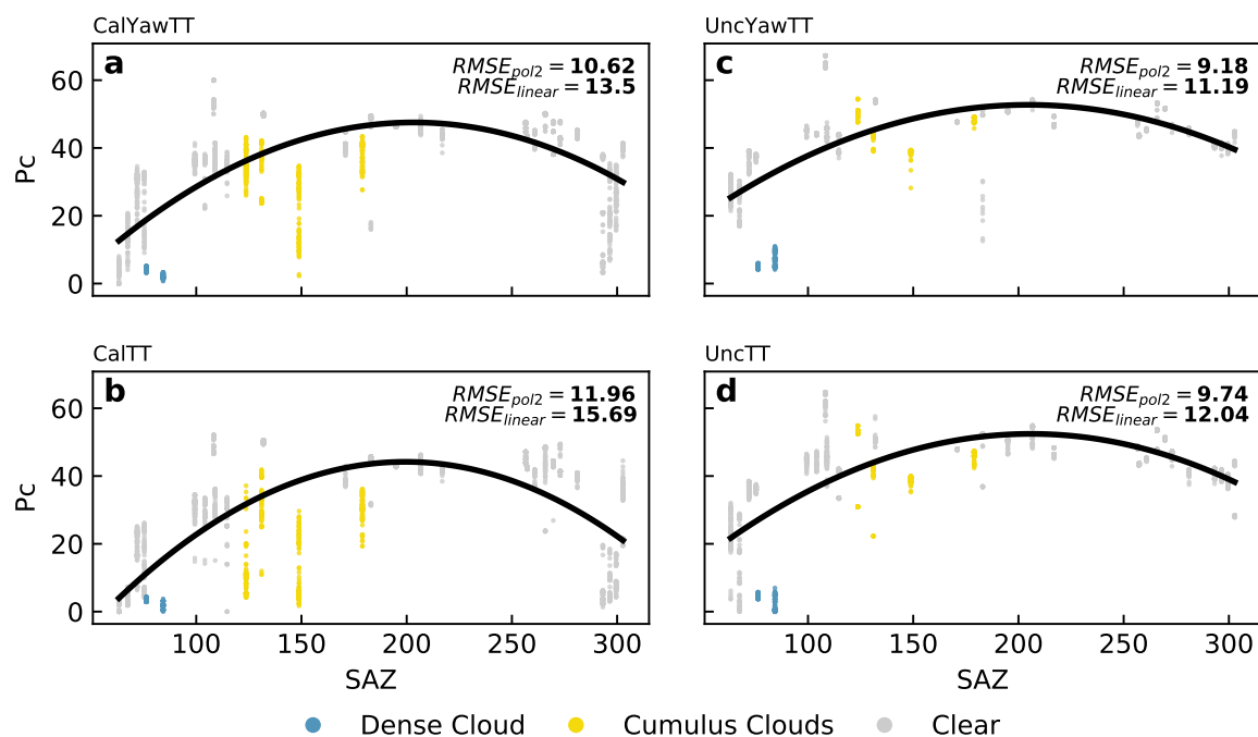
Figure A1. Stability of (c) UncYaTT in alignment of data sets acquired with Cumulus clouds covering the sky over Grassland areas in comparison to (a) CalYawTT, (b) CalTT and (d) UncTT and better fit of polynomial regression of PC along Sun azimuth angle.
