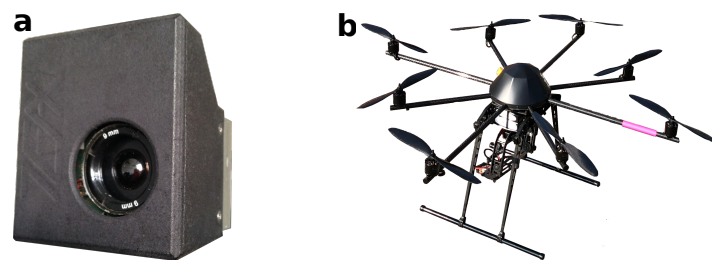
Figure 2. Image acquisition equipment. (a) Flir Tau 2 336 with external heated shutter system. (b) MK Okto XL 6S12.
