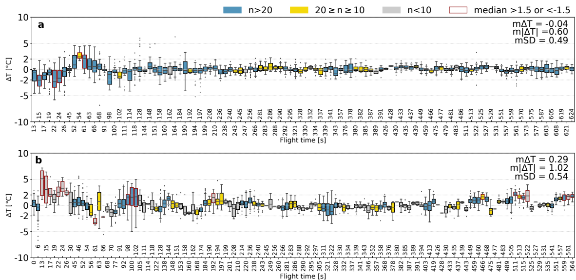
Figure 6. Temperature differences at time t of features in images acquired within (a) the next 4 seconds (b) minimum 50 seconds to paired features in image acquired at time t . n is the number of tiepoints. Please note the non-continuous and non-identical time scaling.
