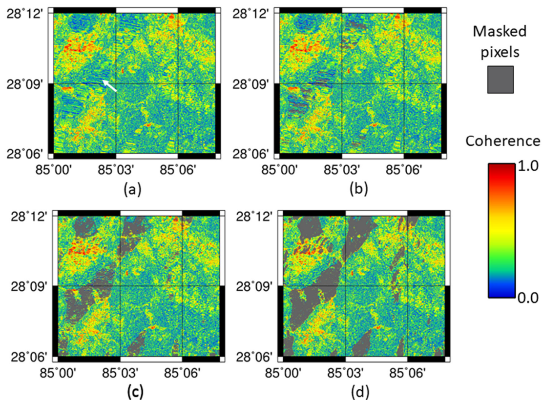
Figure A1 (a) Pre-event coherence map for Jharlang with white arrow indicating distorted pixels. (b, c, d) The effect of masking pixels for which the contributing area was over 5000, 2000 and 1000 m 2 respectively
