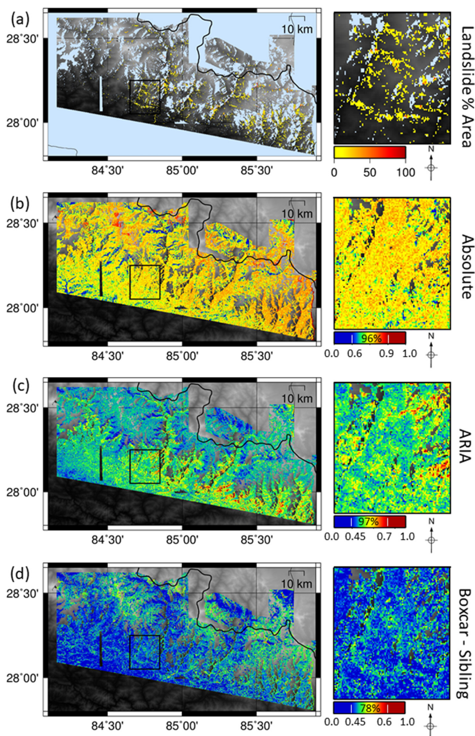
Figure 10. Classifier surfaces for 200 m \times 220 m aggregate pixels. (a) the percentage of each aggregate pixel made up of landslide pixels. (b, c, d) the mean value of the classification surface for each method within each aggregate pixel. These surfaces are normalized to a range between 0 and 1 with 1 being most likely to be a landslide. Colour bars are non-linear, but linear between the white lines and labelled with the percentage of pixels across the whole area that lie in this linear range.
