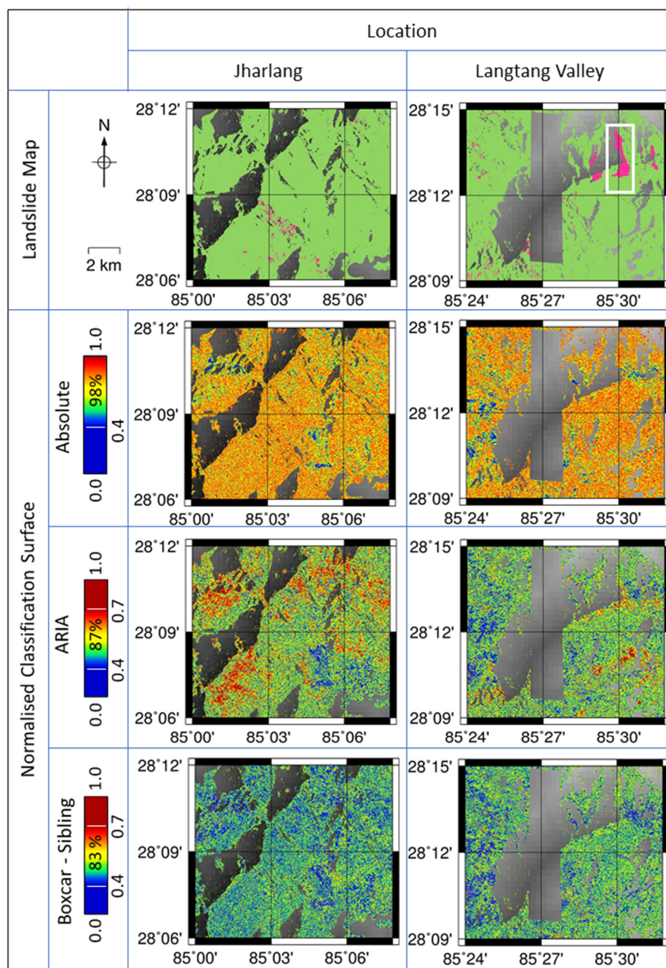
Figure 8. Classification of individual landslides for two example locations. Each column shows mapped landslide polygons (pink) [2] and the normalized classification surface calculated from each method for the Jharlang (left) and Langtang Valley (right) regions. Colour bars are non-linear but linear between the white lines and labelled with the percentage of pixels across the two areas that lie in this linear range. The main body of the Langtang Valley landslide is indicated in white.
