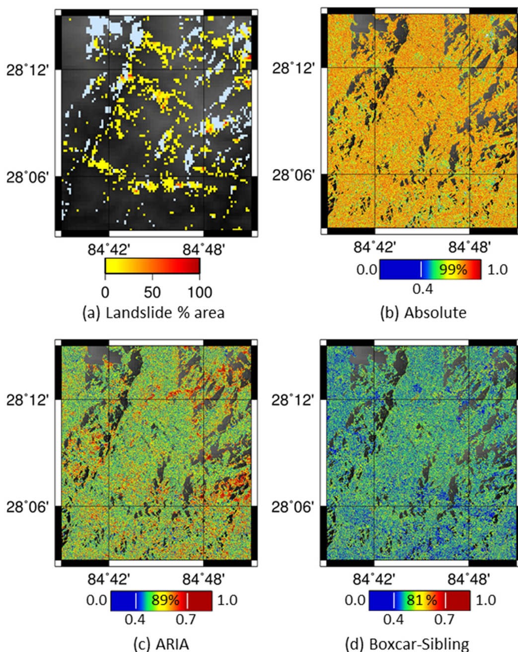
Figure A2 (a) The percentage of each 10 \times 10 aggregate pixel made up of landslide pixels. (b,c,d) The classifier value before aggregation for the surfaces produced by absolute, ARIA and Bx-S methods respectively. Each surface has been normalised to range between 0 and 1 with 1 most likely to be a landslide. Colour bars are non-linear, but linear between the white lines and labelled with the percentage of pixels across the whole area that lie in this linear range. The area shown corresponds to the smaller area shown in Figure 10
