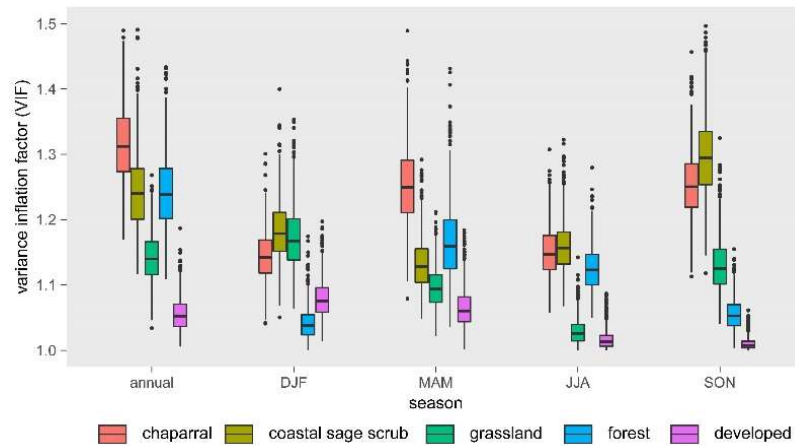
Figure S1. Variance inflation factors (VIFs) of the multiple linear regressions shown in Figure 12. VIF is a widely used indicator for measuring the multicollinearity in multiple linear regressions. Normally, VIF > 10 indicates severe multicollinearity, 5 < VIF < 10 indicates weak multicollinearity, and VIF < 5 indicates no multicollinearity. Nearly all the VIFs in this study < 1.5 , indicating these multiple linear regressions are not affected by multicollinearity.
