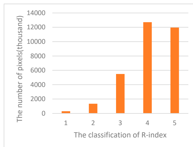
Figure 10. The histogram of R-index.
