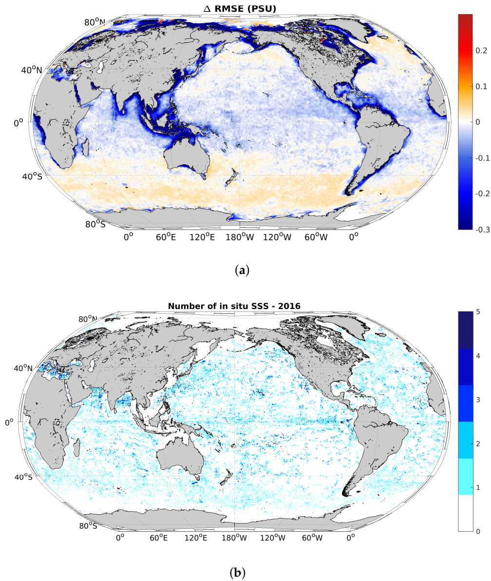
Figure 7. (a) \Delta RMSE based on weekly data, year 2016; (b) density of in situ SSS for the year 2016. The maximum number of in situ observations is \simeq 140 (in the North Atlantic). The colorbar is saturated to 5 in order to facilitate the visualization of the measurement sites at a global scale.
