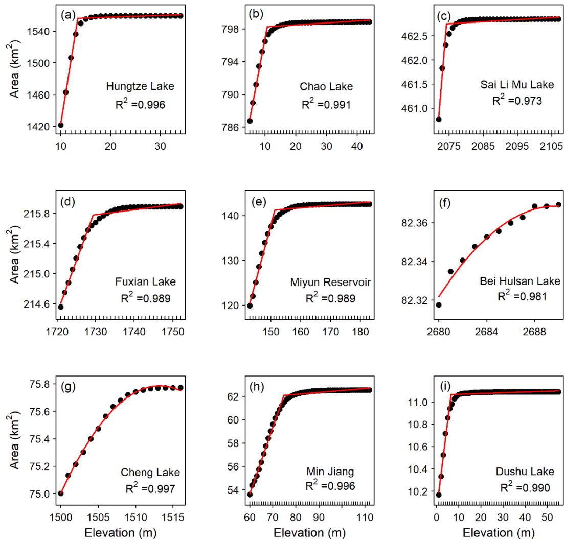
Figure S1. Hypsometric analysis for diverse sized lakes and reservoirs.
