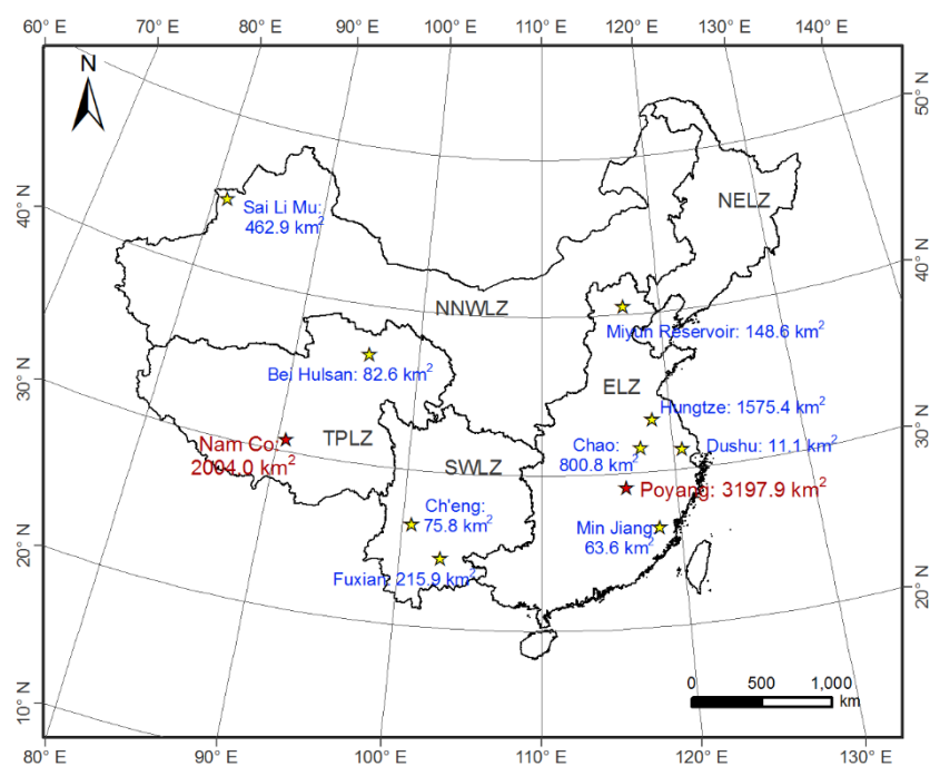
Figure S2. Locations of the 11 exemplary lakes and reservoirs on hypsometric analysis.
