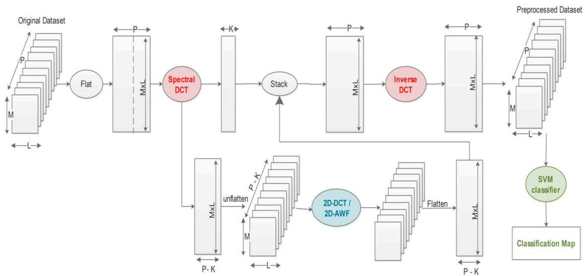
Figure 2. Detailed flowchart of the proposed spatial filtering in DCT domain-based frameworks for hyperspectral imagery classification.
