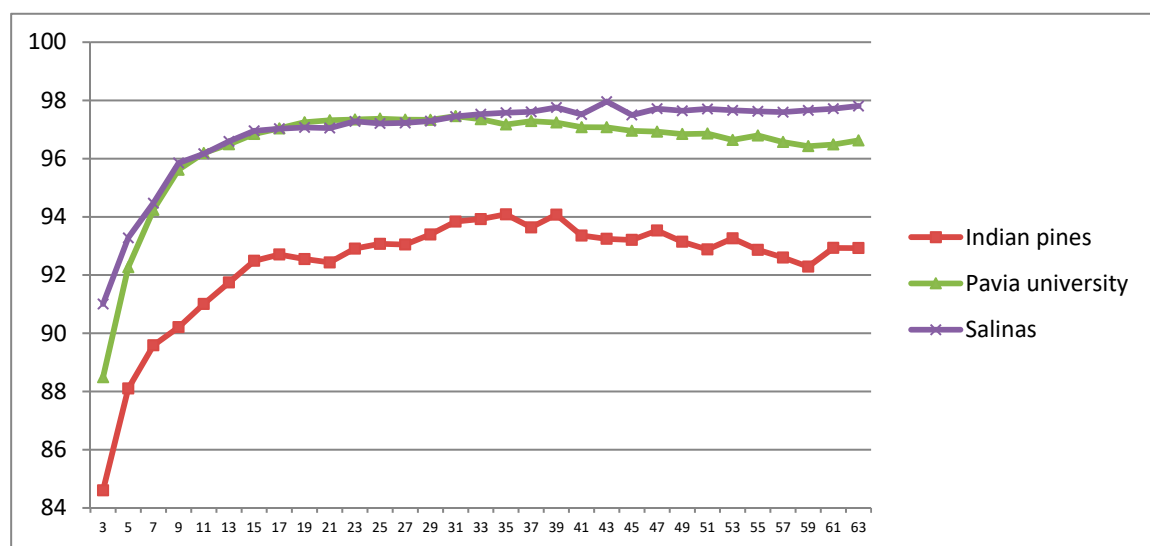
Figure 10. Overall Accuracy (OA%) with respect to the Wiener filter patch size in CDCT-WF_SVM on Indian Pines, Salinas, and Pavia University datasets.
