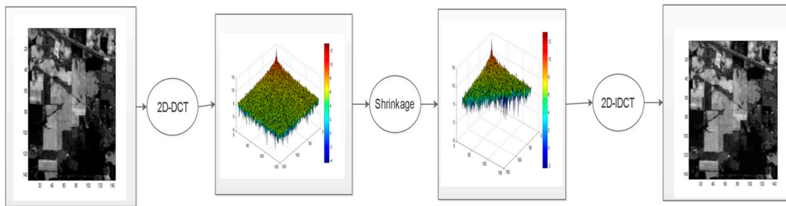
Figure 3. Flowchart of global 2D-DCT filtering step.
