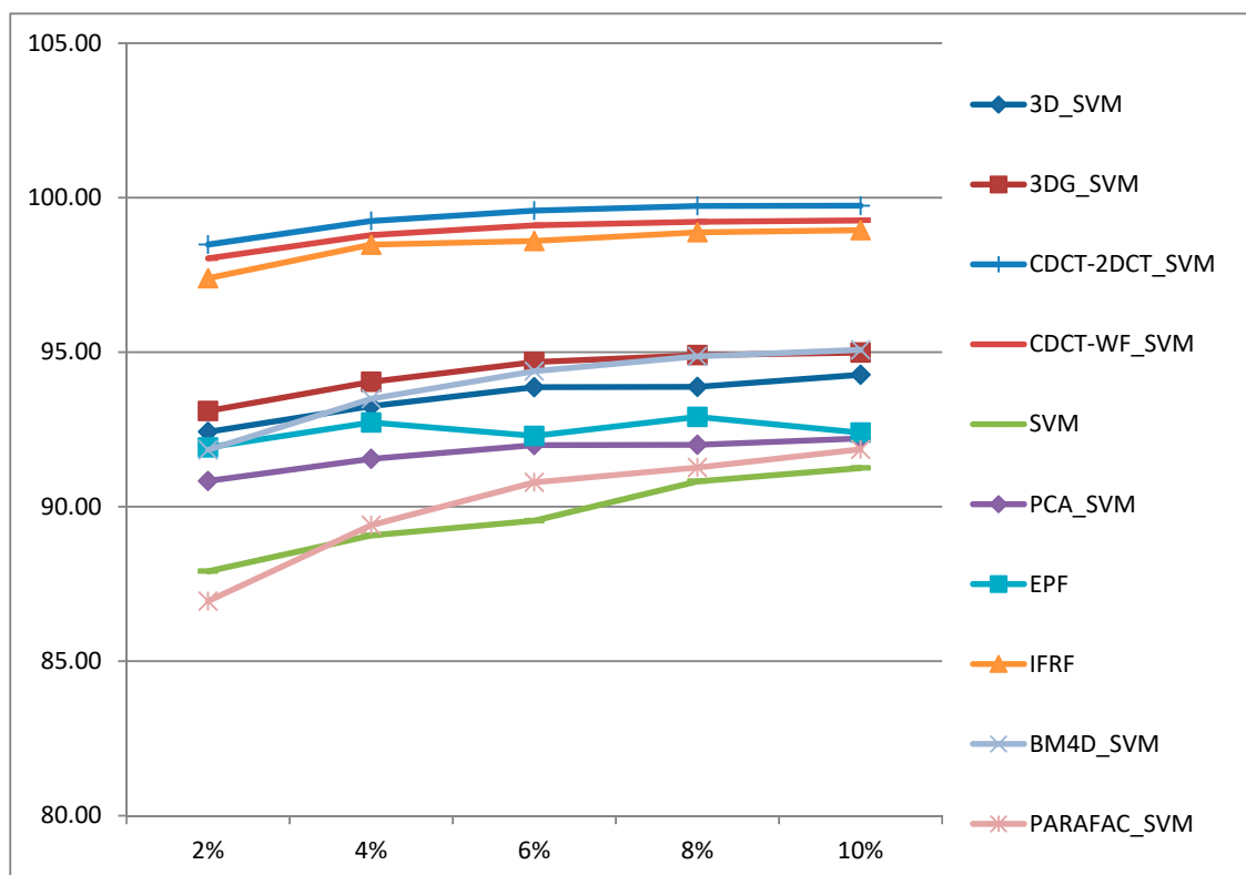
Figure 14. Overall Accuracy (OA%) of all methods with different training samples proportions on Salinas dataset.
