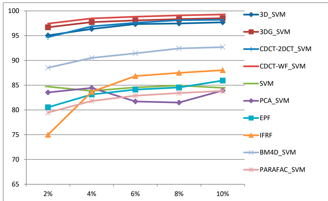
Figure 16. Overall Accuracy (OA%) of all methods with different training samples proportions on the Pavia University dataset.
