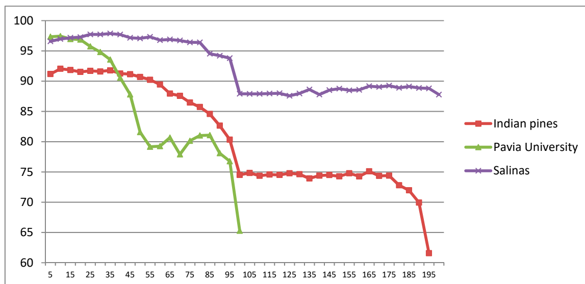
Figure 7. Overall Accuracy (OA%) with respect to the number of the first retained DCT coefficients in CDCT-2DCT_SVM on the Indian Pines, Salinas, and Pavia University datasets.
