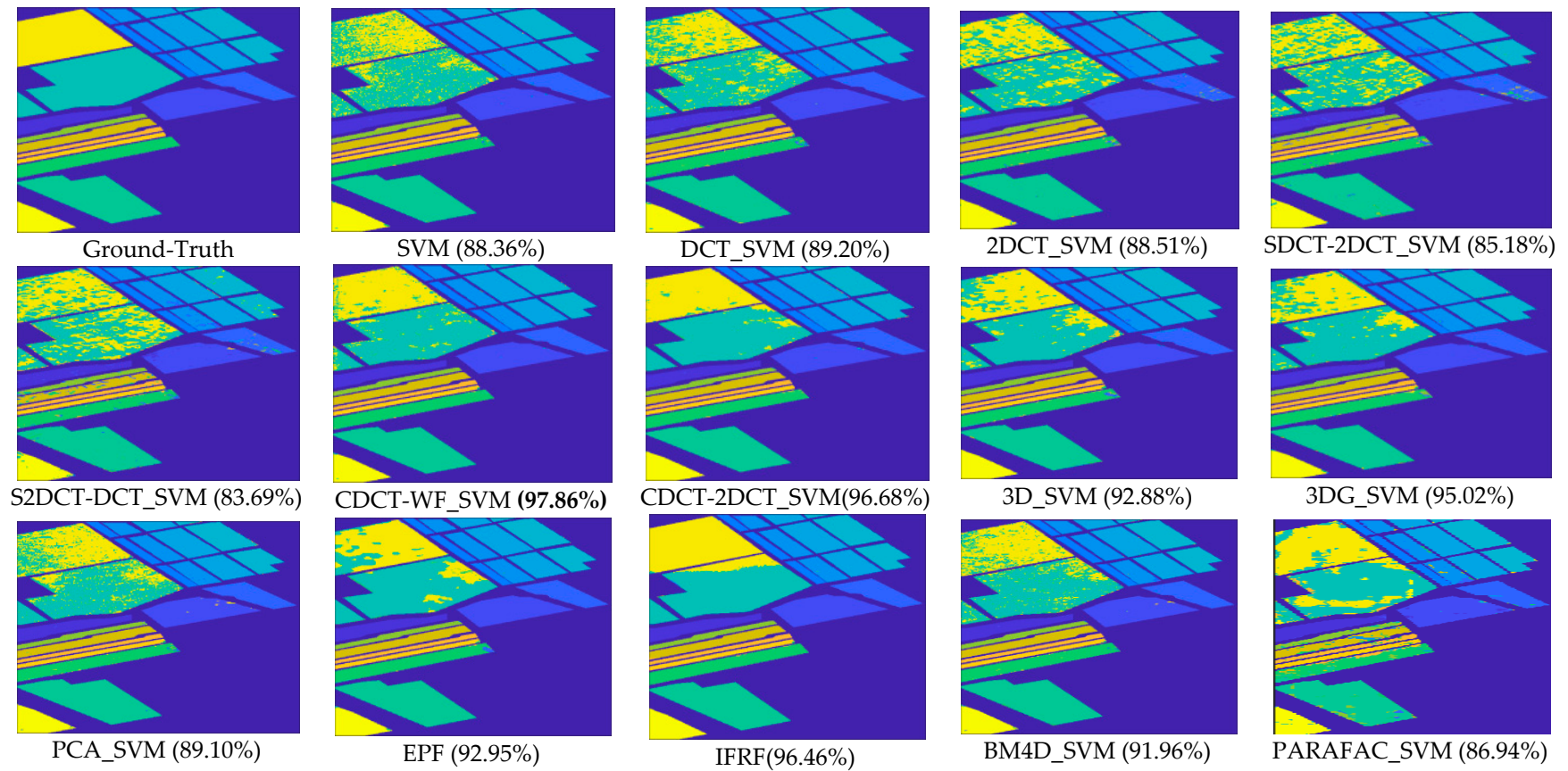
Figure 13. Classification maps created from the results of different methods on the Salinas dataset.
