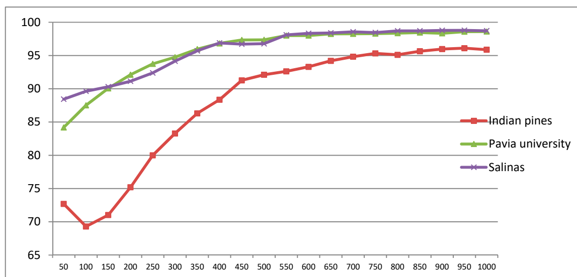
Figure 8. Overall Accuracy (OA%) with respect to the different selected 2D-DCT thresholds in CDCT-2DCT_SVM on Indian Pines, Salinas, and Pavia University datasets.
