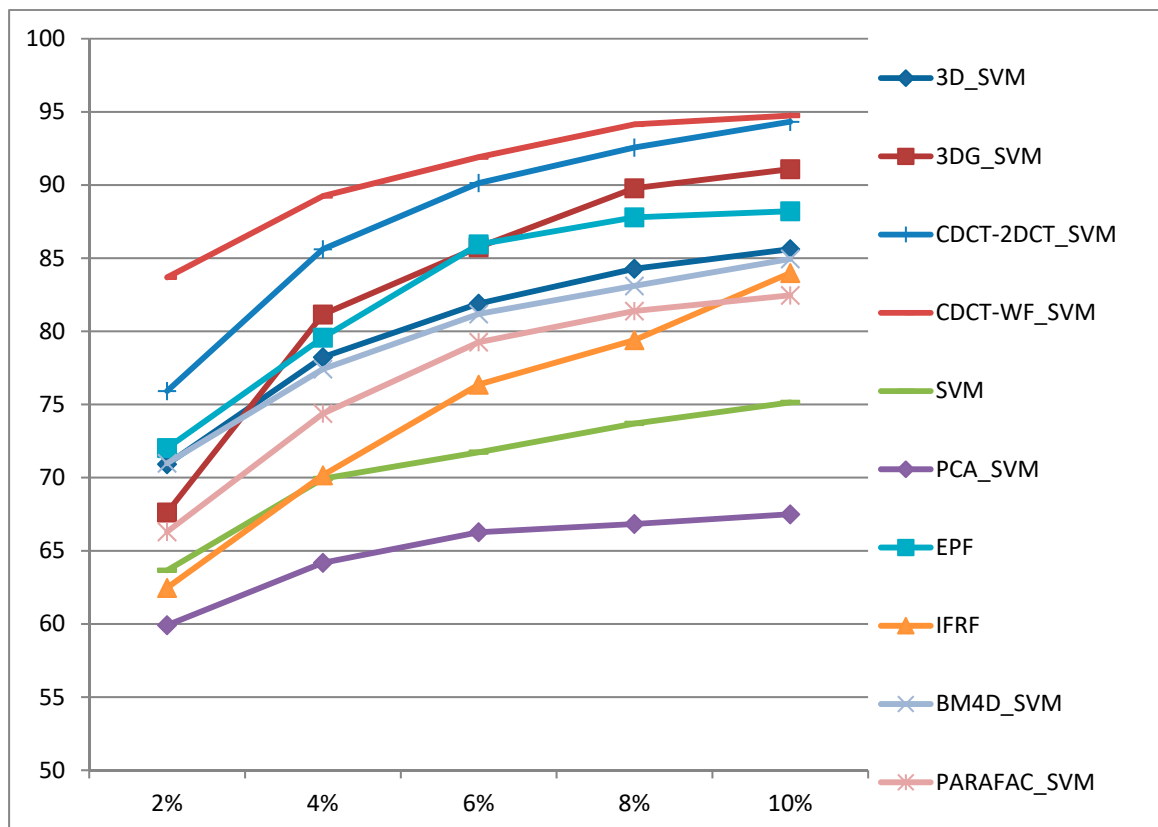
Figure 12. Overall Accuracy (OA%) of the compared methods with different training samples proportions on Indian Pine dataset.
