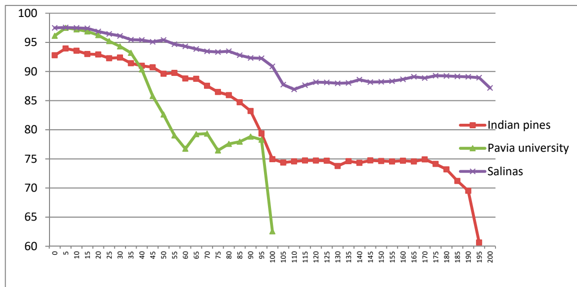
Figure 9. Overall Accuracy (OA%) with respect to the number of the first retained DCT coefficients in CDCT-WF_SVM on Indian Pines, Salinas, and Pavia University datasets.
