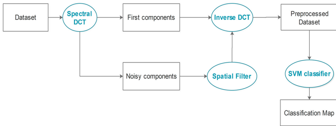
Figure 1. General flowchart of the spatial filtering in DCT domain-based classification framework for hyperspectral imagery.
