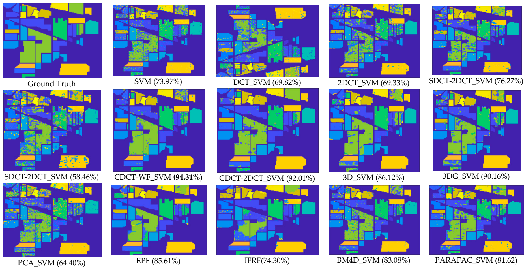
Figure 11. Classification maps created from the results of different methods on the Indian Pines dataset.
