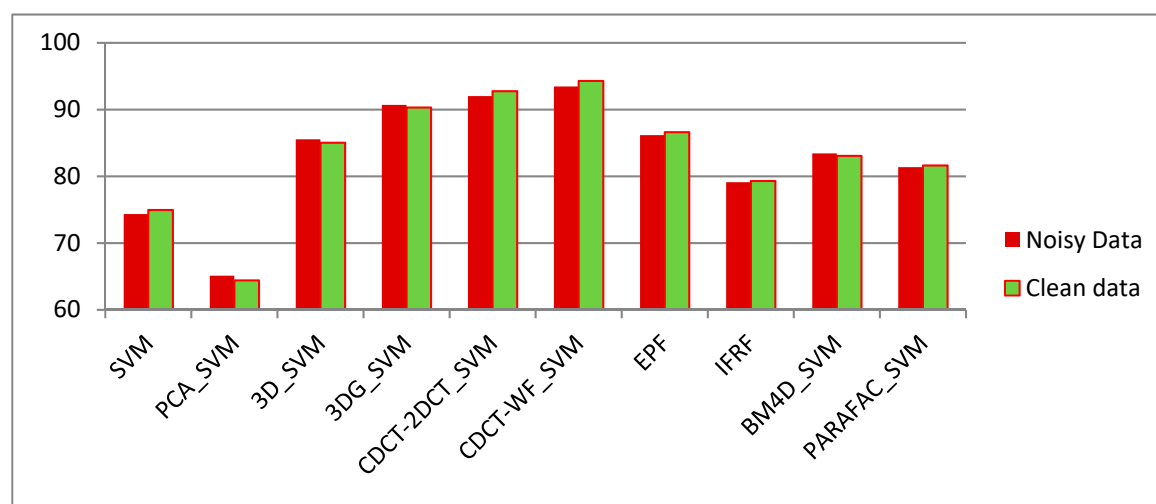
Figure 17. Overall Accuracy (%) of all competing methods on clean and noisy Indian Pines dataset.
