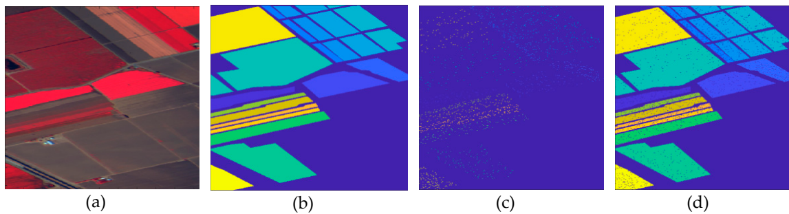
Figure 5. The ground truth related information of Salinas image: (a) false-color composite, (b) ground truth map, (c) training map, (d) test map.
