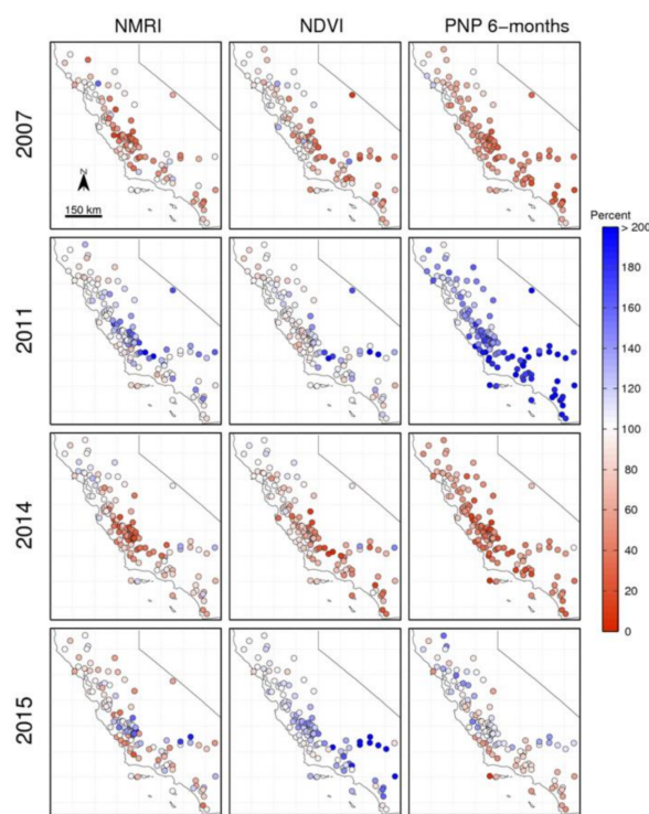
Figure 7. NMRI (left) and NDVI (middle) relative peak amplitude for Plate Boundary Observatory (PBO) H 2 O sites in California, during two dry years (2007 and 2014), a wet year (2011), and a normal year (2015) following a multi-year drought; (Right) six-month Percent of Normal Precipitation (PNP). Both vegetation metrics and PNP are compared to the average for 2007–2016 and reported as a percentage, as shown in the color bar.
