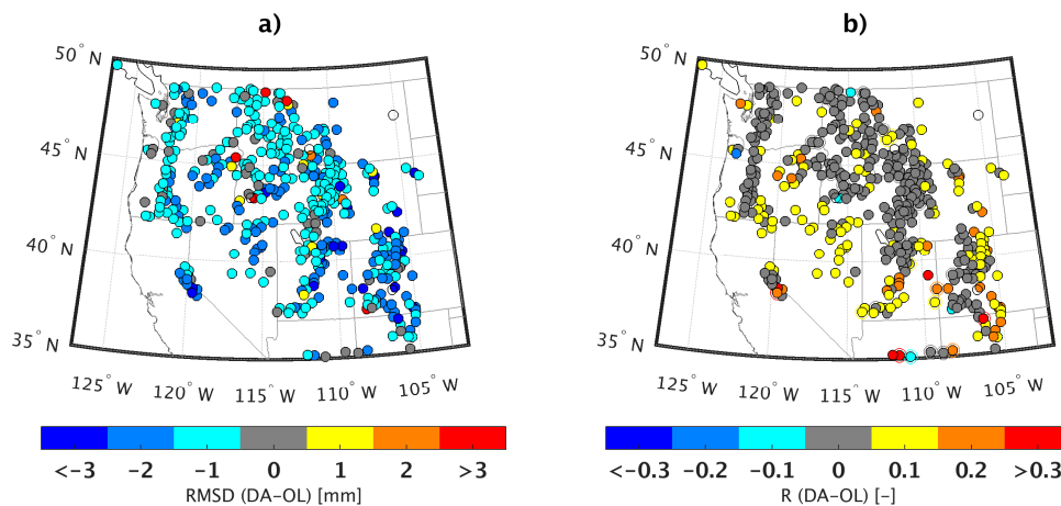
Figure 7. Changes in (a) RMSD and (b) correlation coefficient, R , from OL to DA (computed as DA–OL). The original DA and OL statistics were computed relative to daily SNOTEL SWE observations from 1 September 2001 to 1 September 2009.
