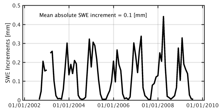
Figure 8. Time series of absolute values of SWE increments (i.e., the difference in DA–OL) averaged across the entire study domain, including the temporal mean of the entire simulation as shown in the title.
