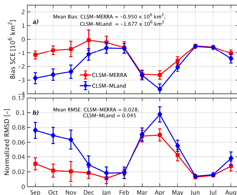
Figure 1. (a) Bias and (b) normalized RMSD of monthly SCE from CLSM-MERRA and CLSM-MLand for part of the Northern Hemisphere poleward of 35^\circ\text{N} for the period 1 September 2001 to 1 September 2009. Metrics are computed vs. monthly MODIS SCE observations. Error bars represent the standard deviation across space. Normalization of the RMSD in (b) is by the maximum annual MODIS SCE.
