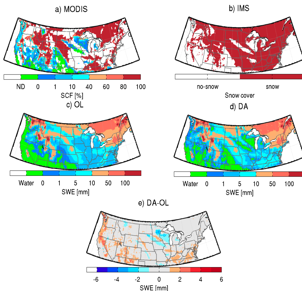
Figure 4. Maps of (a) MODIS snow cover (%); (b) IMS snow cover; (c) open-loop (OL) (model control run) SWE (mm); (d) model analysis (DA) SWE (mm) and; (e) the difference between DA and OL SWE (mm) for 17 January 2003.
