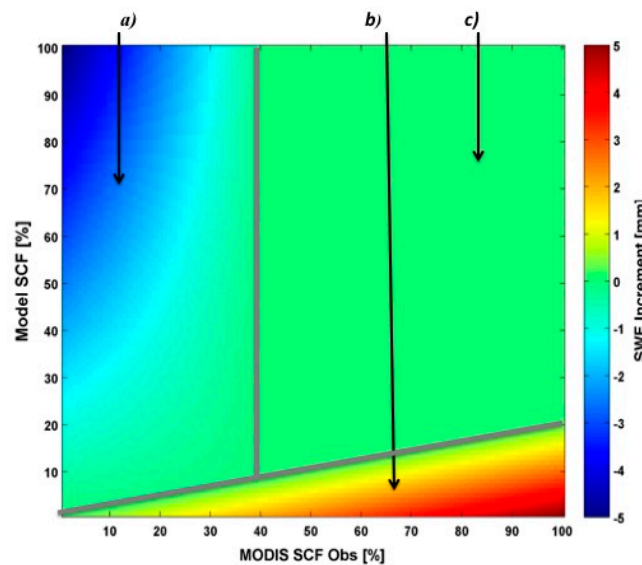
Figure 2. Graphical representation of the empirical formulation used to compute the SWE increment during assimilation of daily MODIS SCF for incr_{SWE}^{Max} = 5 \text{ kg} \cdot \text{m}^{-2} , SWE_{min} = 26 \text{ kg} \cdot \text{m}^{-2} , \alpha = 0.2 [-] , and \beta = 40\% . Blue (a) corresponds to snow removal, red and yellow (b) represent the addition of snow and, green (c) corresponds to when there is no significant difference between the model and the observations.
