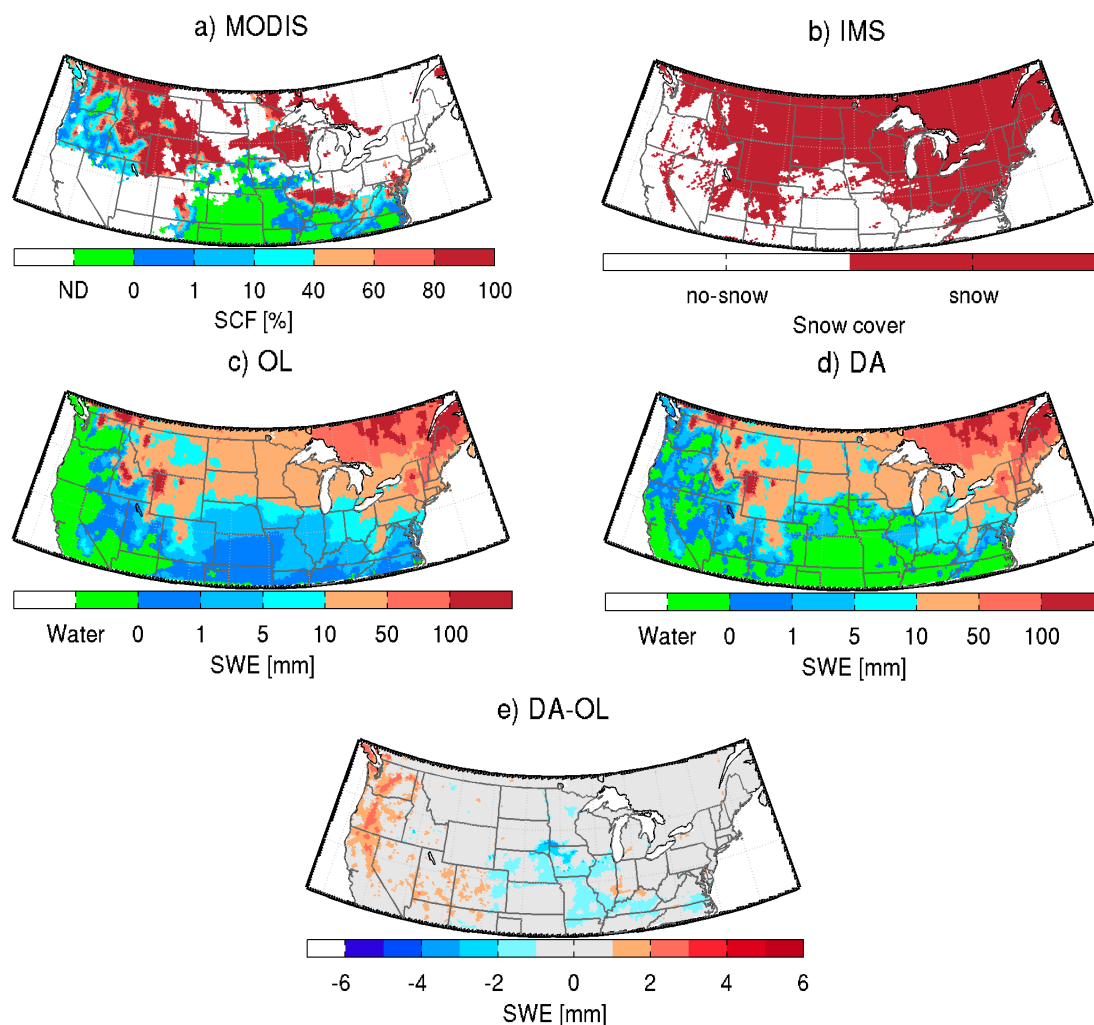
Figure 5. Same as in Figure 4 except for 12 February 2003.
