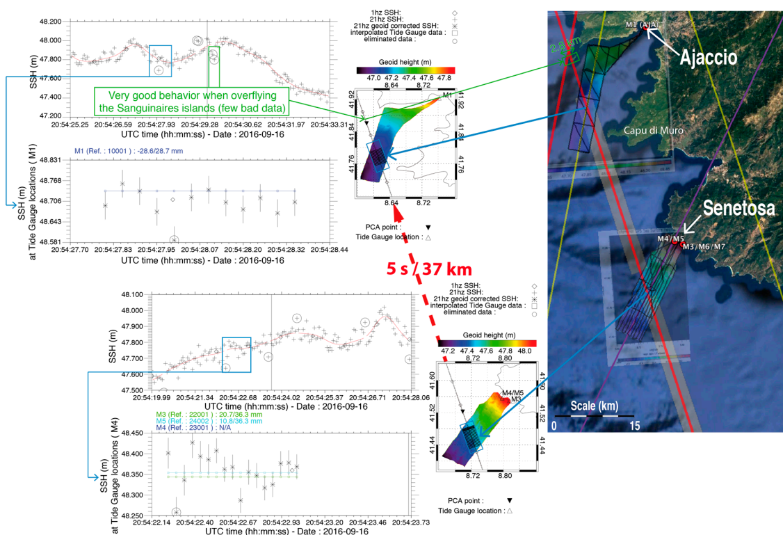
Figure 5. Example of sea surface height (SSH) bias processing for Sentinel-3A in synthetic aperture radar (SAR) mode (pass 741, cycle 8). For each independent processing (Ajaccio, top/Senetosa, bottom) the upper plot shows \pm 4 s of altimeter SSH series around the point of closest approach (PCA). The lower plots show the selected SSH (inside the geoid area) that are corrected from the geoid height differences between the SSH location and the tide gauge locations.
