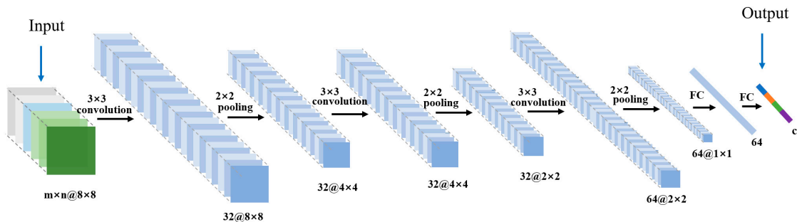
Figure 4. The network structure of 2D CNN for multi-temporal crop classification.
