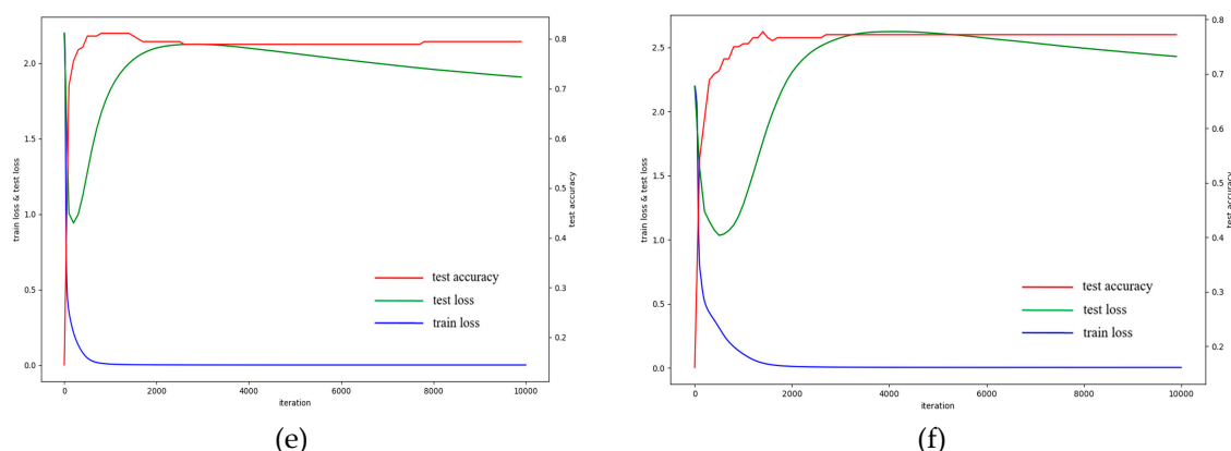
Figure 7. Test accuracy (red line), training loss (blue line), and test loss (green line) with optimal parameters. The test accuracy of 3D CNN shows 0.7%, 1.7% and 2.2% higher than that of 2D CNN in GF2-2015, GF2-2016 and GF1 data, respectively. (a) 3D CNN for GF2 2015 data; (b) 2D CNN for GF2 2015 data; (c) 3D CNN for GF2 2016 data; (d) 2D CNN for GF2 2016 data; (e) 3D CNN for GF1 data; and, (f) 2D CNN for GF1 data.
