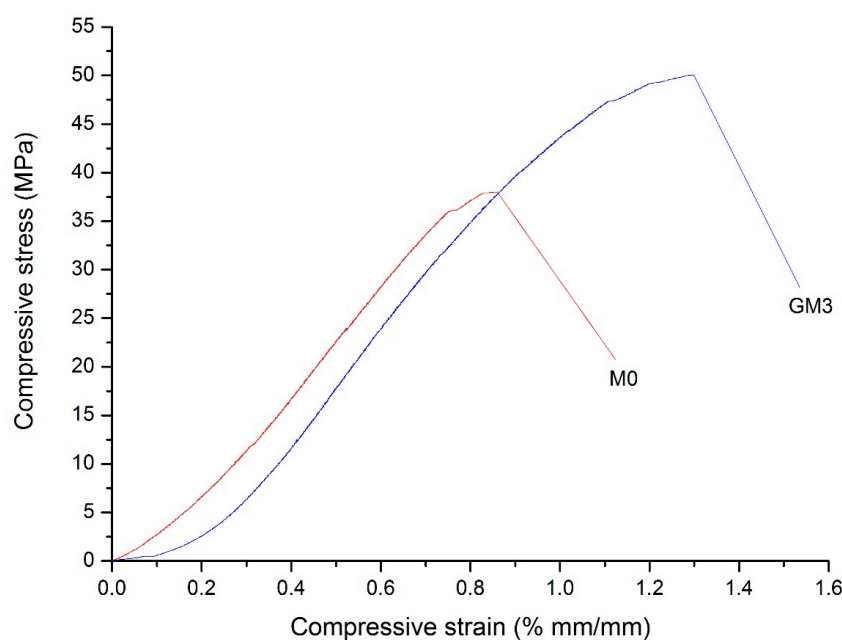
Figure 4. Stress–strain curve for cement paste (M0) and graphene–cement paste (GM3).
