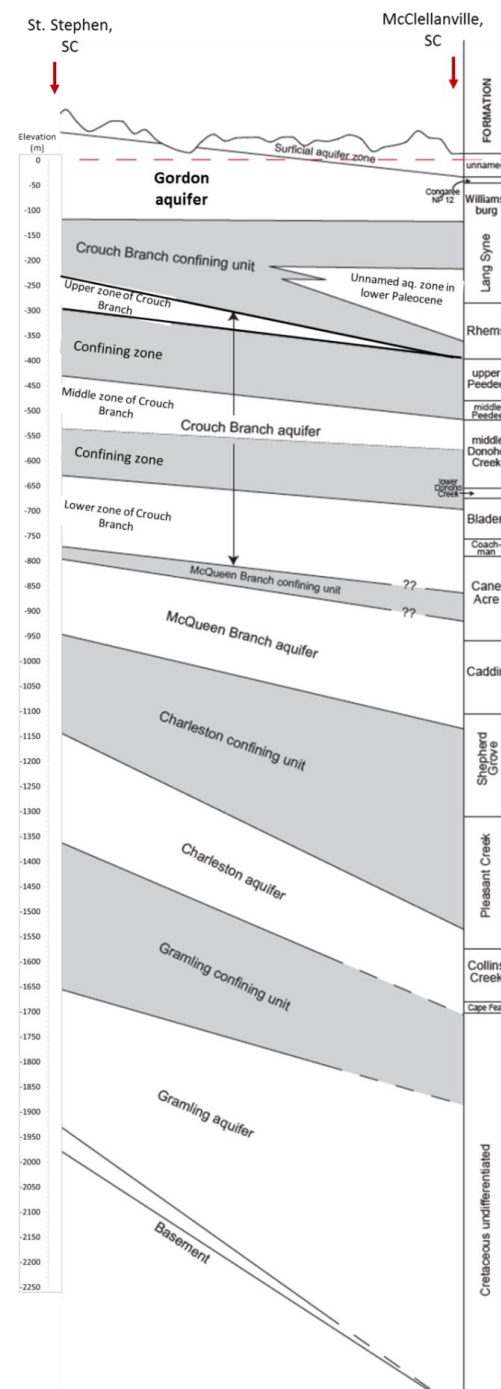
Figure A1. Idealized cross-section of outer coastal plain, central South Carolina, USA [31].
