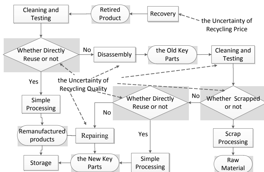
Figure 1. The remanufacturing processes flowchart of EOL construction machinery.
