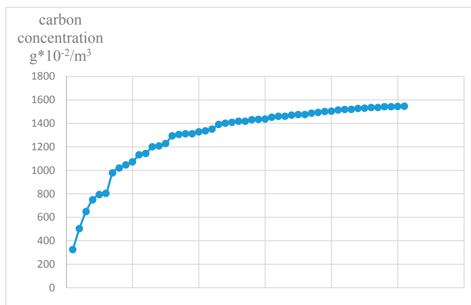
Figure 10. Discrete point of each concentration value.
