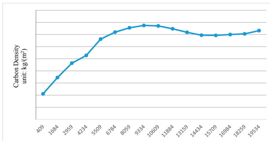
Figure 9. Carbon density in different rings.
