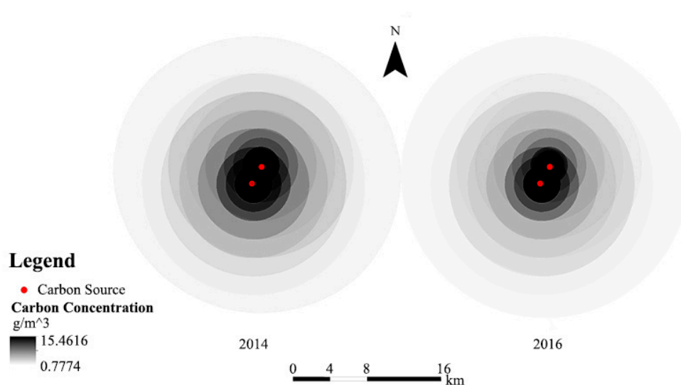
Figure 6. The spatial distribution of carbon concentration.
