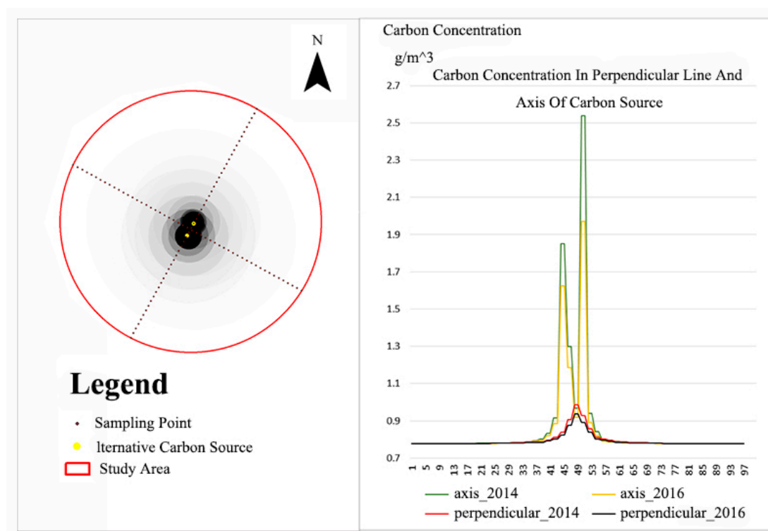
Figure 7. The sampling points and the sampling results.
