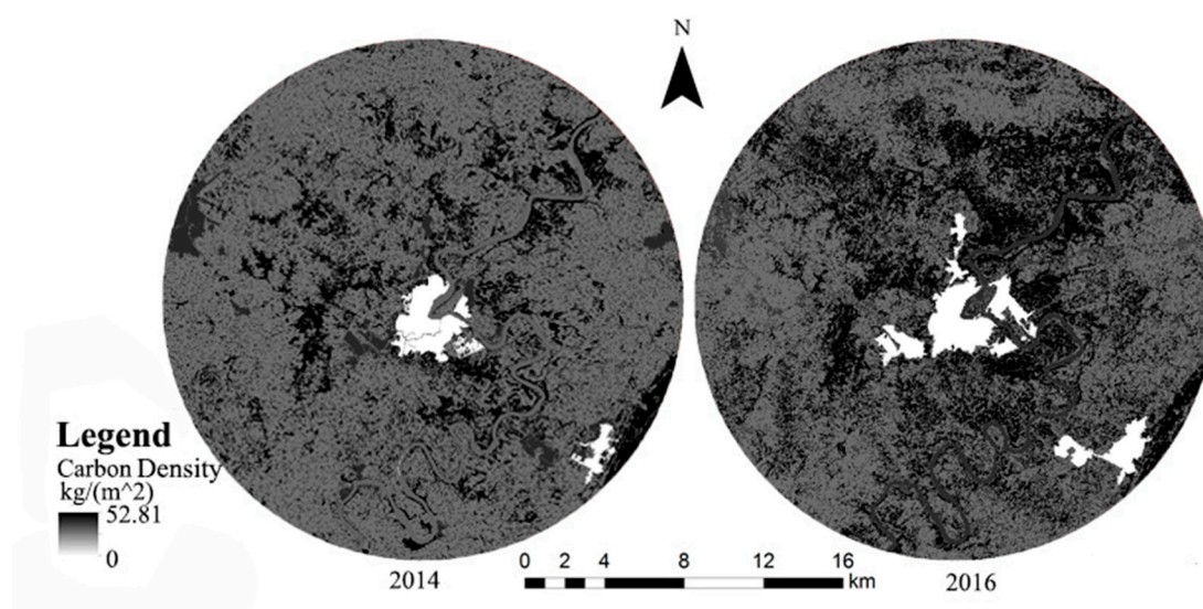
Figure 3. The distribution of carbon stocks in 2014, the distribution of carbon stocks in 2016.
