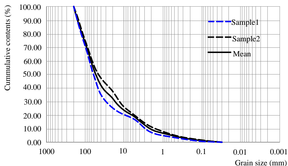
Figure 8. Grain-size distribution of the Yanshuijin sediment.
