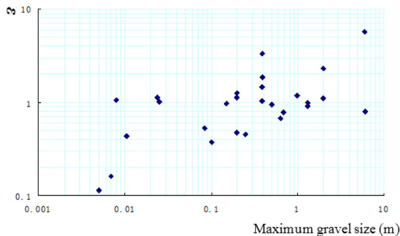
Figure 16. Maximum gravel size in accumulation zones for the 27 debris flow catchments.
