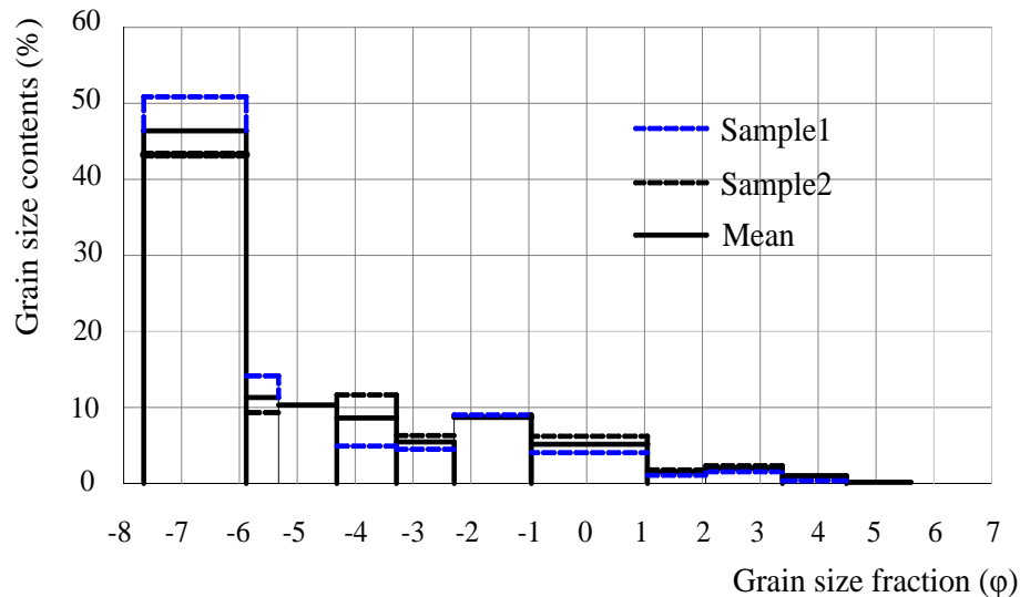
Figure 9. Histogram of the grain-size distribution of the Yanshuijin deposition.
