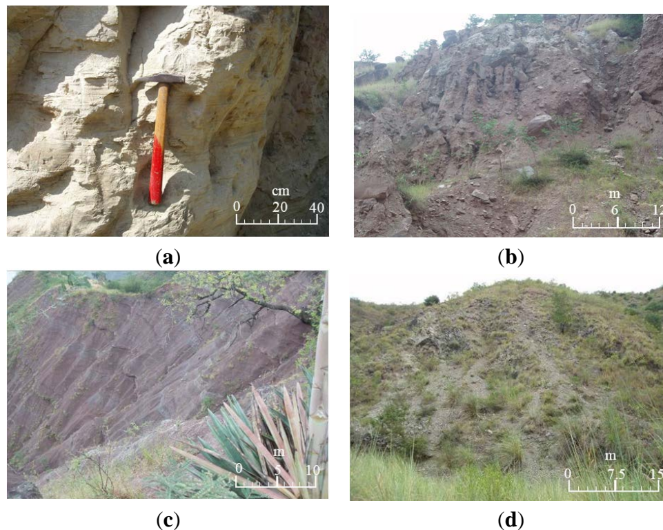
Figure 2. Main loose materials developed in the study region: (a) Longjie fine sand layer; (b) Madianhe layer; (c) Red-bed layer; and (d) Metamorphic layer (phyllite).
