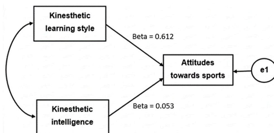
Figure 1. Path analysis model of the predictive power of kinesthetic profile on attitude toward sports in adolescents. Note: Values are standardized \beta coefficients; R^2 = 0.423 .
