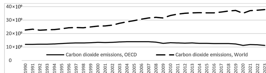
Figure 3. CO 2 emissions from the OECD and the world, in billion tons. Source: Our World in Data, https://ourworldindata.org/co2-emissions (accessed on 22 December 2025).
