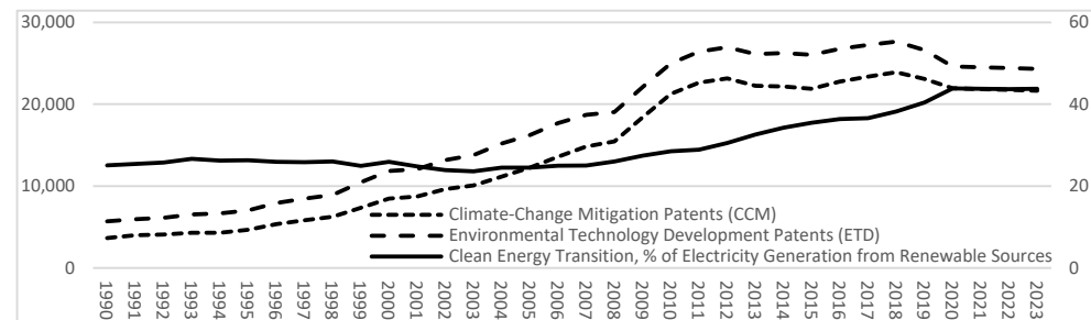
Figure 4. Clean energy transition (right lane), CCM and ETD patents (left lane) in OECD, 1990–2023. Source: OECD Patents Database and World Bank WDI.
