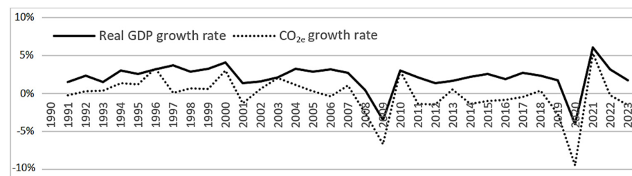
Figure 2. Yearly real GDP and CO 2 e % growth rates in OECD, 1990–2023. Note: Growth rates reflect logarithmic first differences. Source: OECD Database, https://data-explorer.oecd.org/ (accessed on 22 December 2025).
