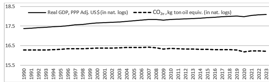
Figure 1. Real GDP and CO 2 emissions in OECD, in logarithms, 1990–2023. Notes: Real GDP is PPP adjusted and is in constant 2015 US$. CO 2 emissions are in kg ton of oil equivalent. Source: OECD Database, https://data-explorer.oecd.org/ (accessed on 22 December 2025).
