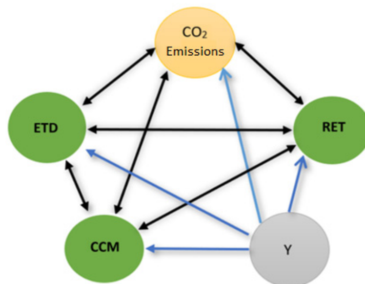
Figure 6. Fourier–Granger-causality results. Note: The black (blue) arrow indicates bidirectional (unidirectional) causality. The green (gray) circle indicates the CO 2 e mitigation (acceleration) effect of the variable in the relevant circle.
