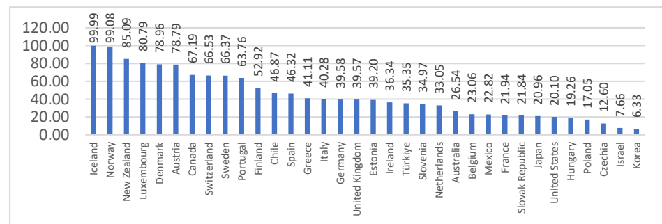
Figure 5. Energy mixes of selected OECD nations, 2023. Source: World Bank WDI Database.
