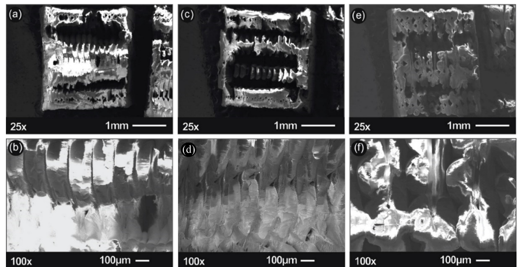
Figure 8. SEM images of the tensile fracture area of the representative specimens for the 1st (a,b), 2nd (c,d) and 3rd (e,f) recycle courses.
