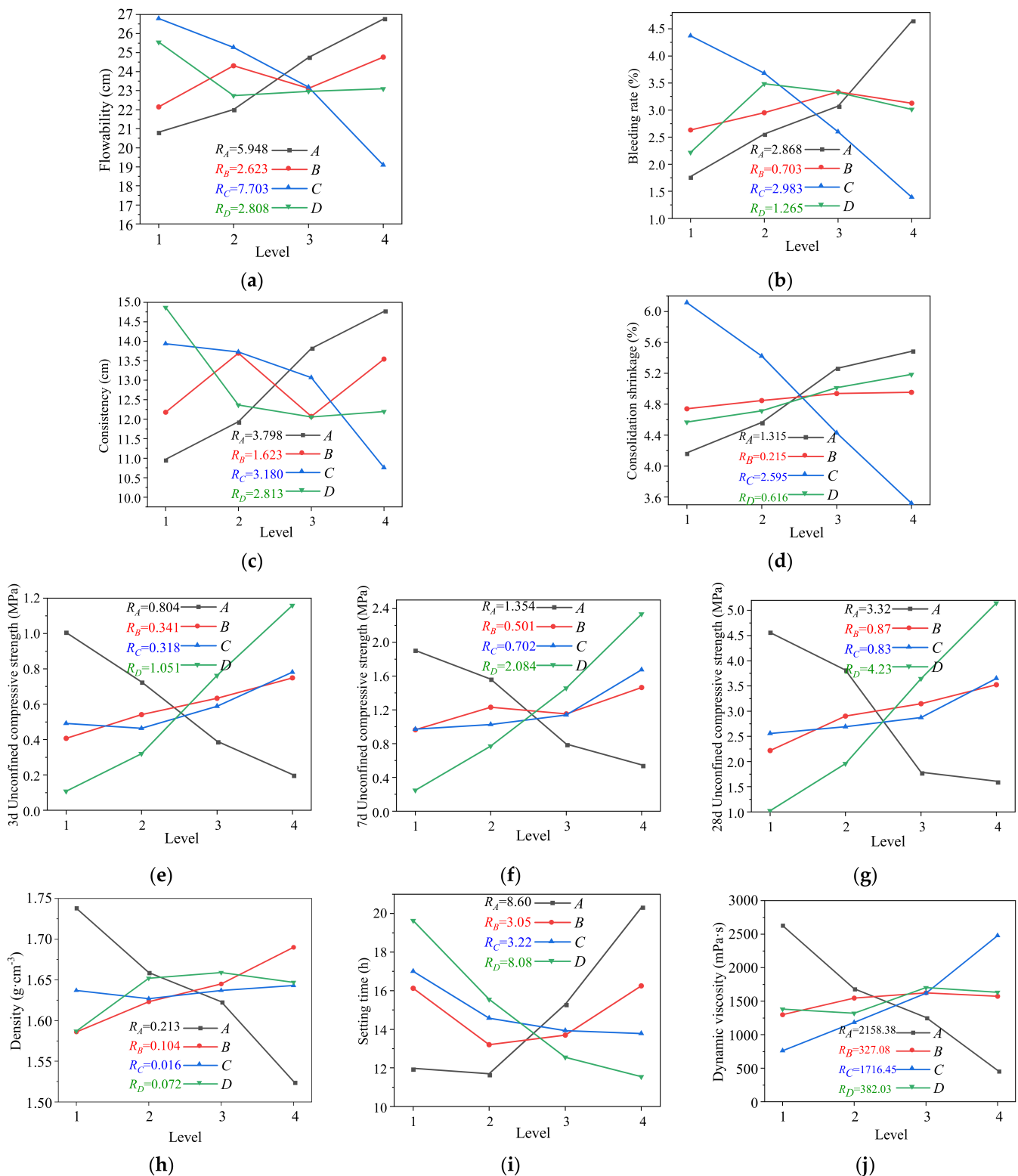
Figure 5. Range analysis of basic grout properties: (a) flowability; (b) bleeding rate; (c) consistency; (d) consolidation shrinkage; (e) 3 d compressive strength; (f) 7 d compressive strength; (g) 28 d compressive strength; (h) density; (i) setting time; (j) dynamic viscosity.
