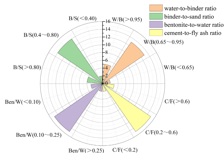
Figure 1. Distribution frequency of grout ratios.
