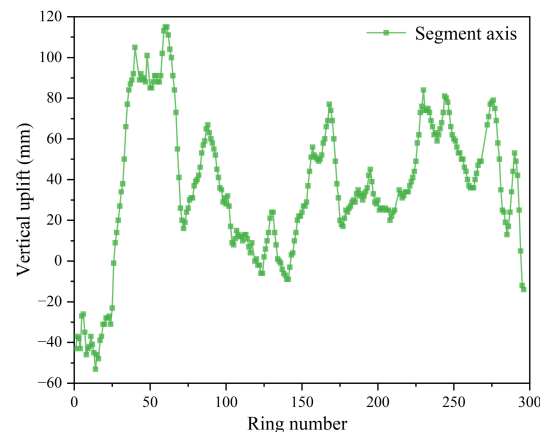
Figure 12. Segment floating displacement of the tunnel.
