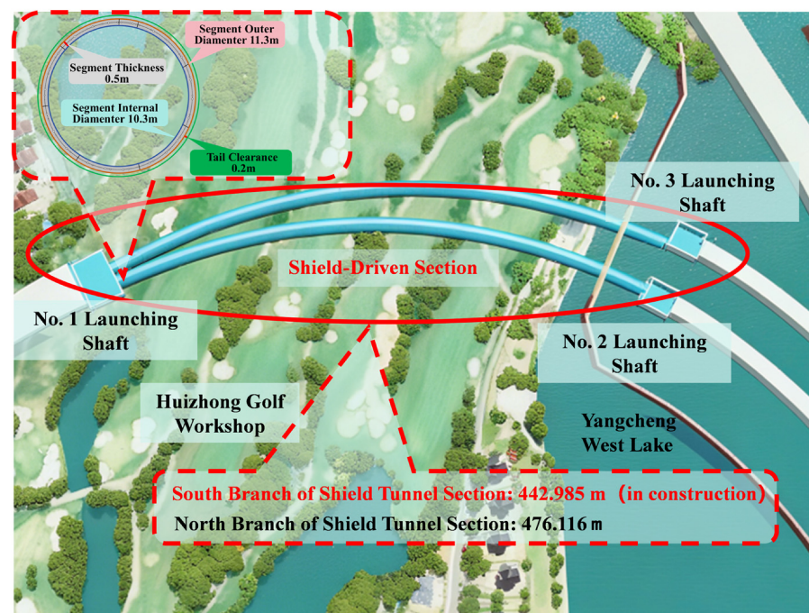
Figure 3. Overview of the Yangcheng West Lake Third Channel Shield Tunnel Project.
