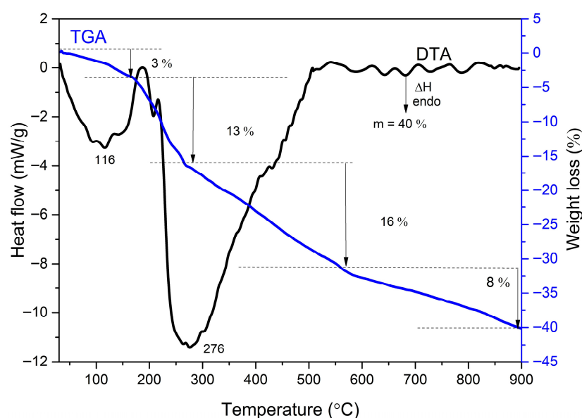
Figure 14. TGA/DTA thermogram of AgNPs synthesized by the extract of the Zinnia elegans L. blossoms.
