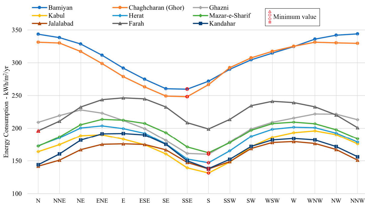
Figure 14. Annual energy usage of different orientations in various cities across Afghanistan.
