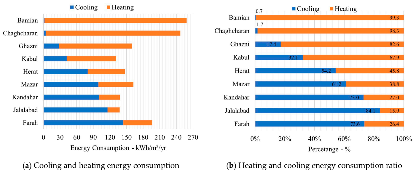
Figure 17. Annual cooling and heating energy consumption in various cities.
