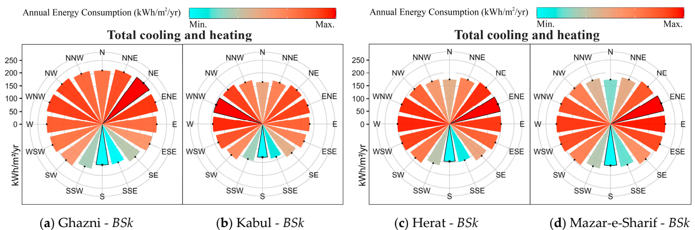
Figure 13. Impact of orientation on total annual energy consumption in (a) Ghazni, (b) Kabul, (c) Herat, and (d) Mazar-e-Sharif.
