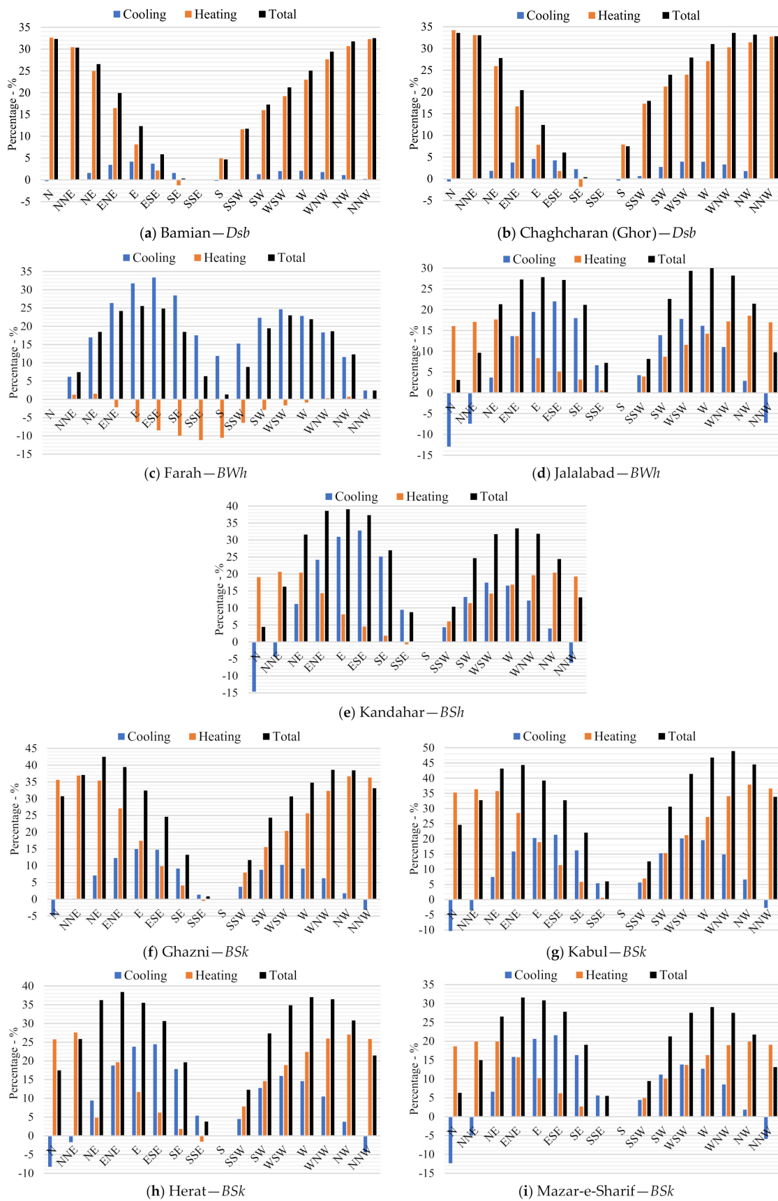
Figure 16. Percentage increase or decrease in cooling, heating, and total energy consumption compared to the optimal orientation.
