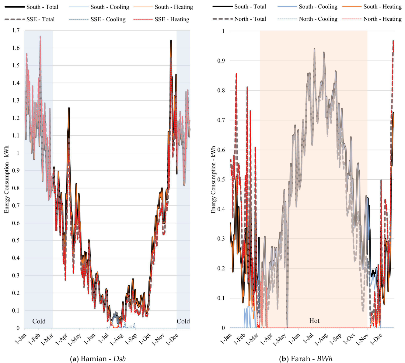
Figure 15. Comparison of the daily energy consumption of best orientation to south orientations in (a) Bamian and (b) Farah.
