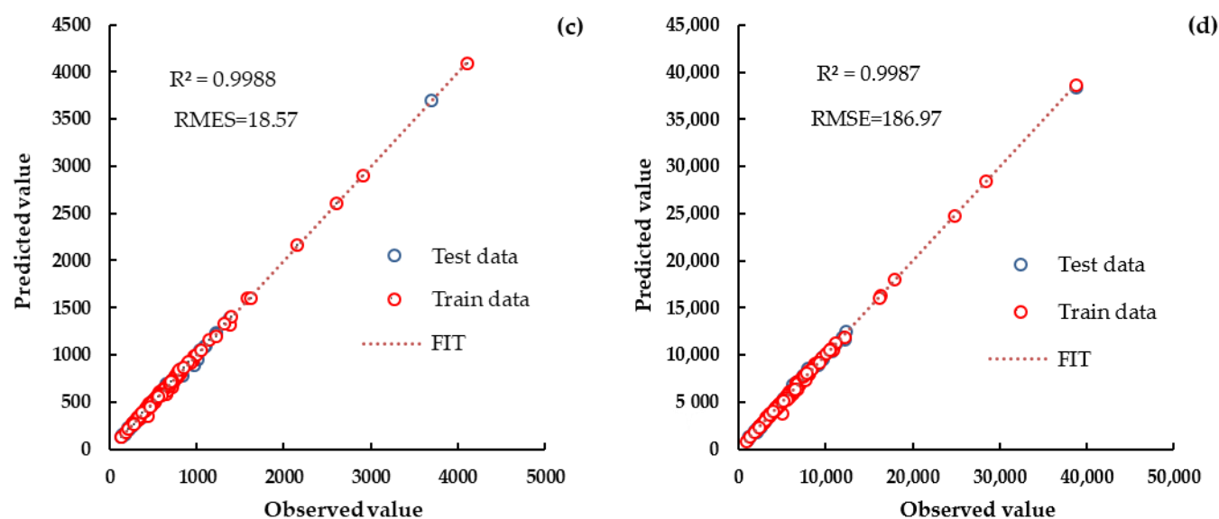
Figure 9. Comparison between observed and predicted values for (a) human health, (b) ecosystem quality, (c) climate change, and (d) resources.
