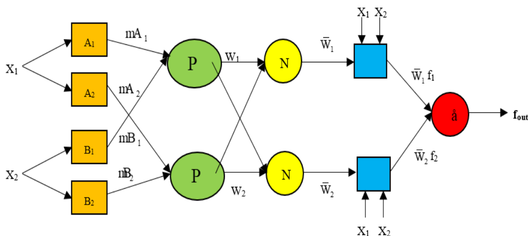
Figure 4. The structure of ANFIS.
