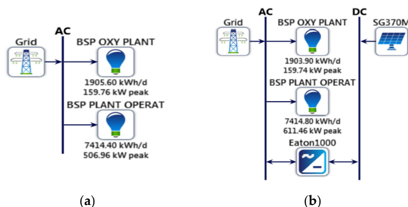
Figure 6. (a) Schematic of the grid-only simulation model, (b) Schematic of FSPV-grid simulation model.
