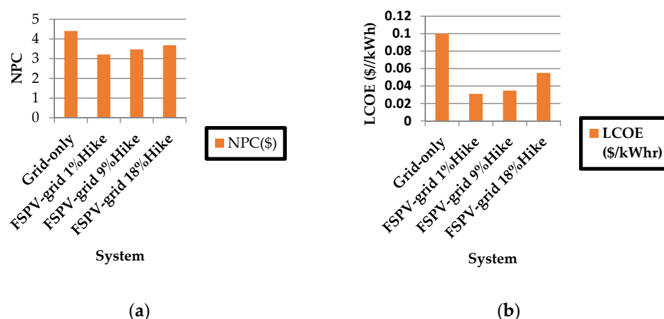
Figure 7. (a) NPC of grid-only and FSPV-grid systems with various price hikes, (b) LCOE of grid-only and FSPV-grid systems with various price hikes.
