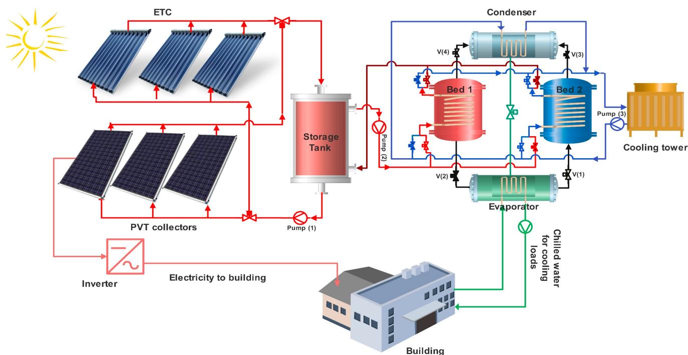
Figure 1. Schematic diagram of the proposed system.
