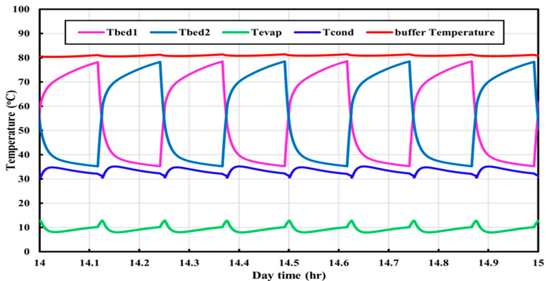
Figure 4. Temperature profiles throughout four cycles for the condenser, evaporator, two beds, and water tank.
