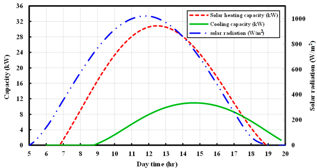
Figure 7. Variation of solar radiation, solar heating capacity and cooling capacity over time for Sharjah city on the 15 June 2019.
