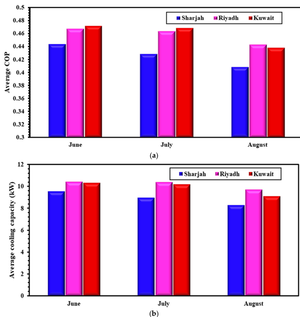
Figure 5. Average COP and cooling capacity of the adsorption chiller for the three months; (a) average COP, (b) average cooling capacity.
