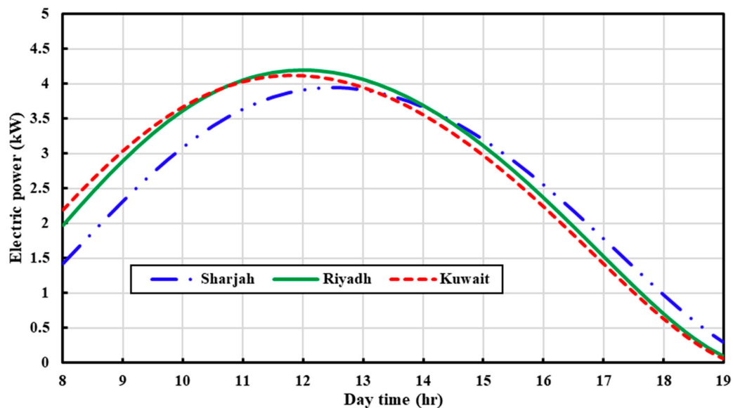
Figure 8. PVT-generated electricity on the 15 June 2019 in the three cities.
