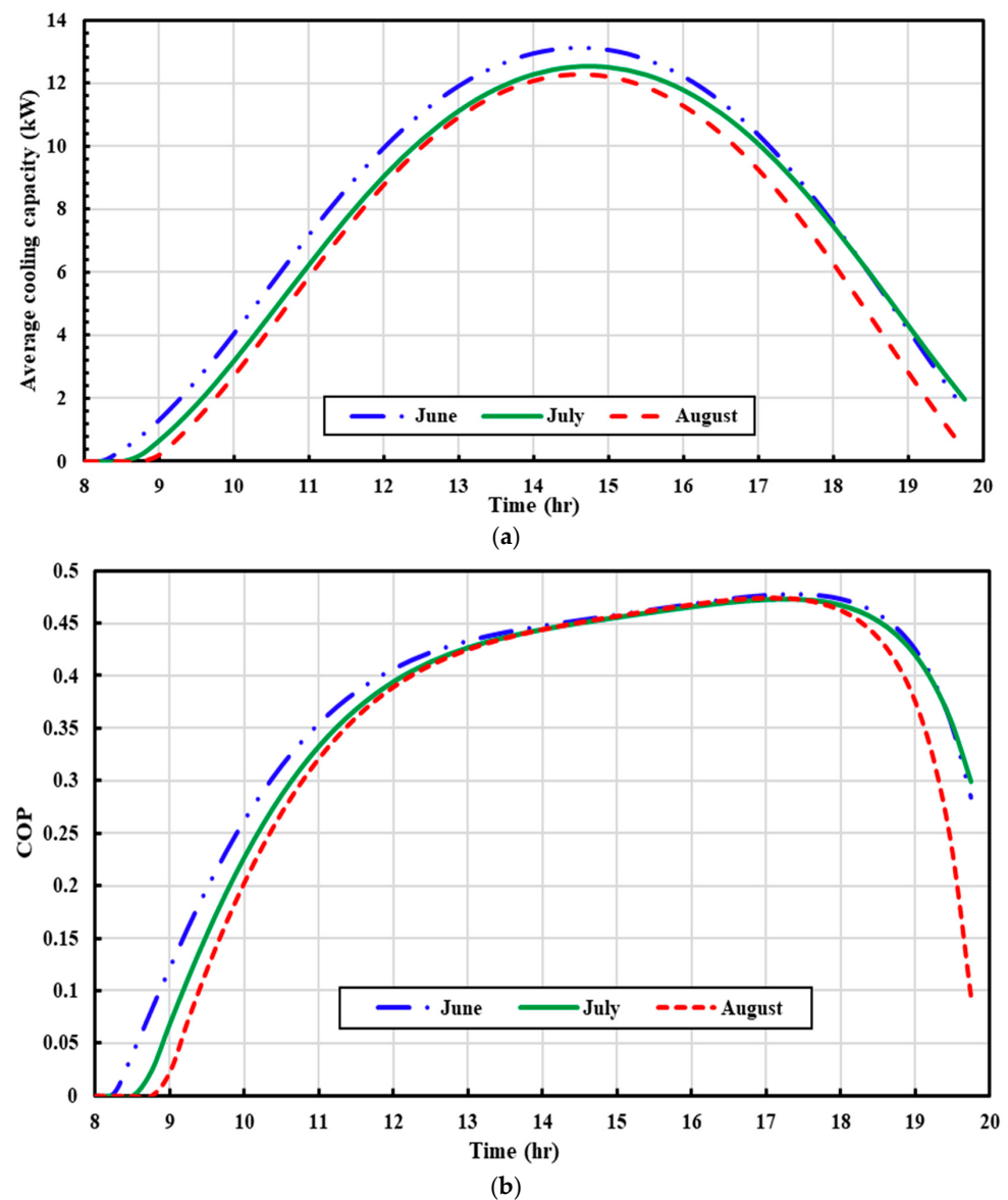
Figure 6. Variation of cooling capacity and COP over time for Sharjah city: (a) cooling capacity, (b) COP.
