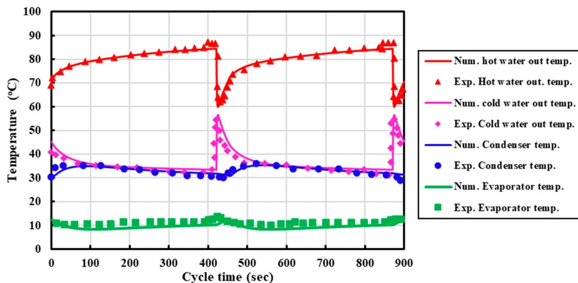
Figure 2. Mathematical model verification: the lines represent the present study and the dots represent experimental data from Ref. [32].
