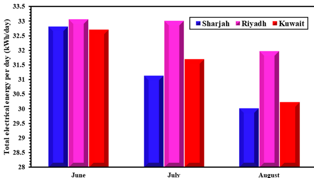
Figure 9. Total electrical generated energy per day for the three months.
