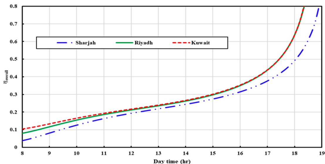
Figure 10. Total system efficiency for all cities under investigation on the 15 June 2019.
